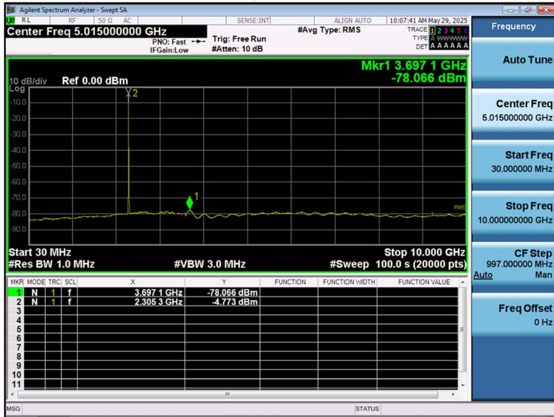
LTE B30_5 M_Conducted Spurious(30 M-10 G)_Low_QPSK_1RB
