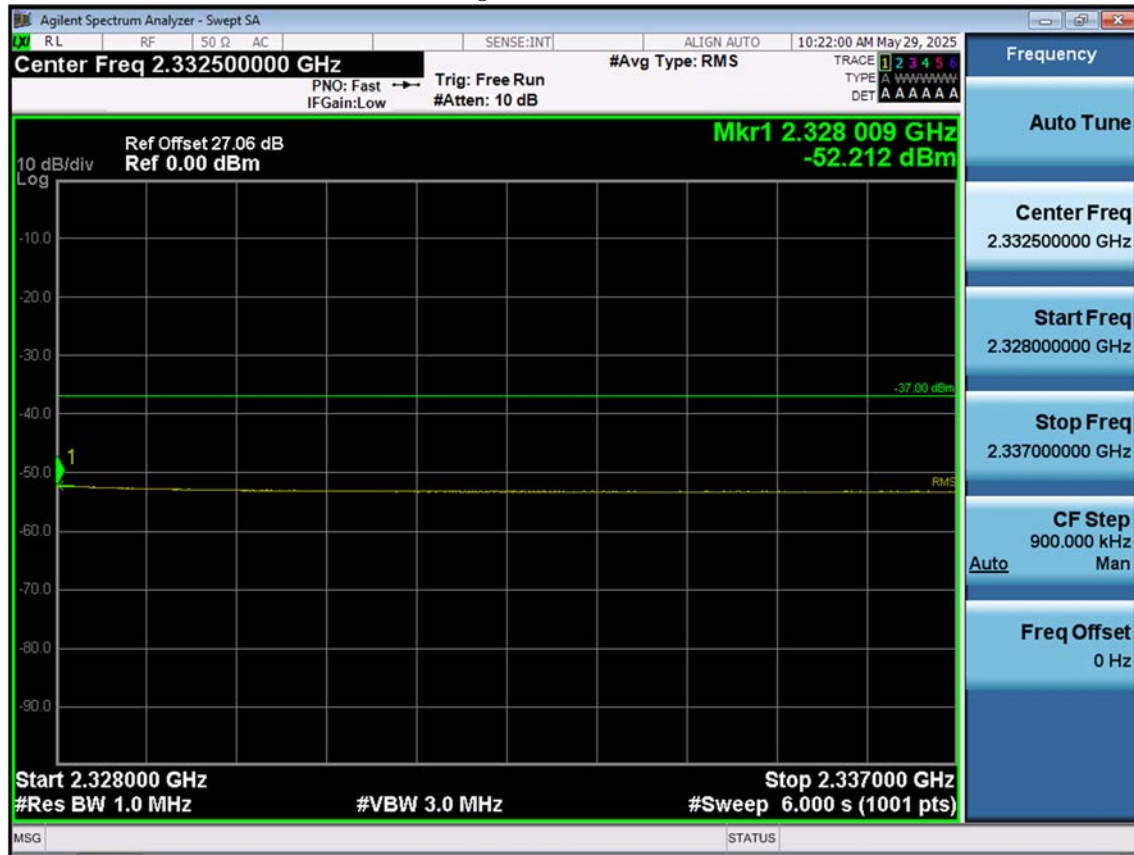
LTE B30_5 M_Band Edge(2328MHz-2337MHz)_Mid_QPSK_1RB
