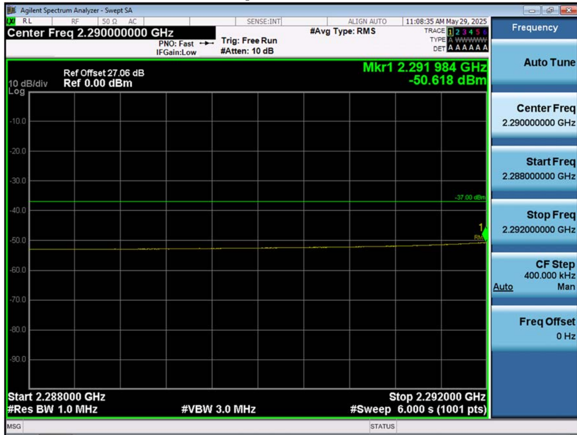
LTE B30_10 M_Band Edge(2288MHz-2292MHz)_Low_QPSK_1RB
