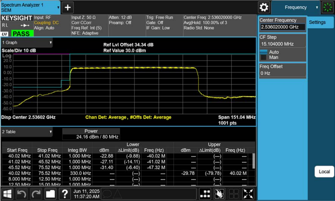
NR41_80 M_Band Edge_Lower_Low_BPSK_FullRB
