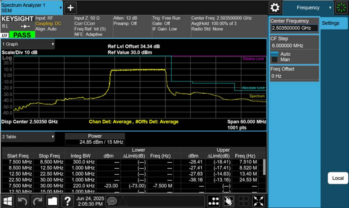
NR41_15 M_Band Edge_Upper_Low_BPSK_FullRB
