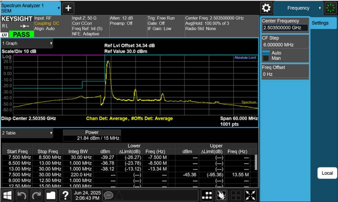
NR41_15 M_Band Edge_Lower_Low_BPSK_1RB
