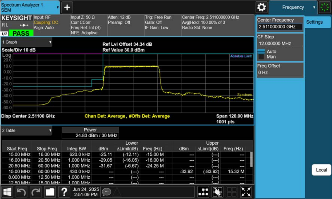
NR41_30 M_Band Edge_Lower_Low_BPSK_FullIRB
