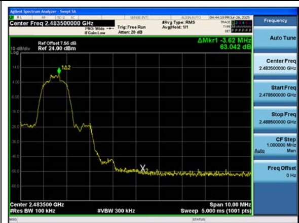
Dual ANT.2 \pi/4 DQPSK Band Edge(Ch. 78)
