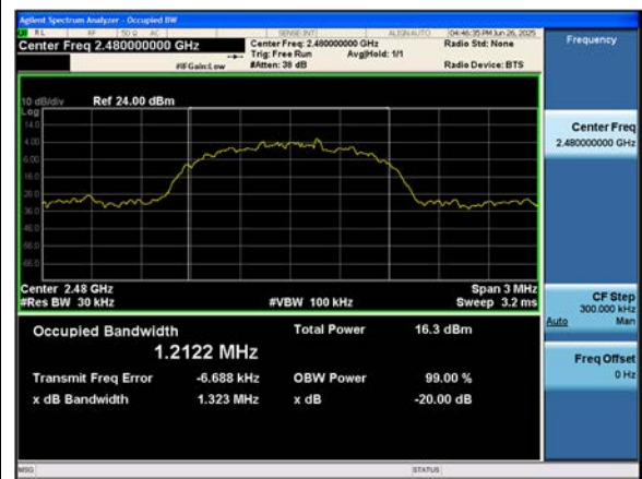
Dual ANT. 2 \pi/4 DQPSK 20 dB BW & 99% OBW (Ch. 78)
