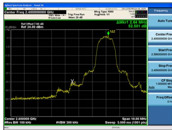
ANT.2 8DPSK Band Edge(Ch. 0)
