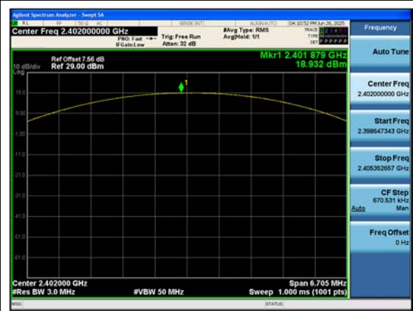
ANT.2 \pi /4DQPSK : Peak Power (Ch. 0)
