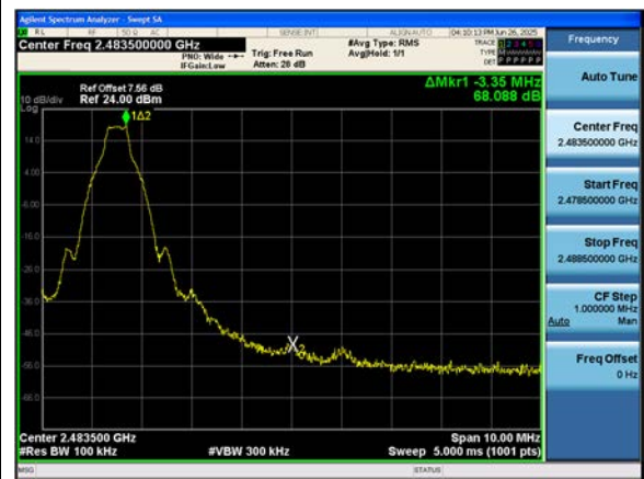
ANT.2 GFSK Band Edge(Ch. 78)
