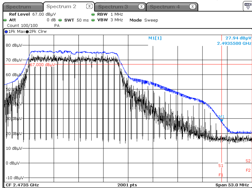
Peak result(802.11ax(HE20) 242T RU61, MCS0, ch.11, X-H)
