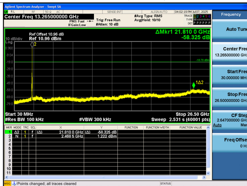
[ANT.2] BW 20M Ch.11(2 462 MHz) 52T RU 40
