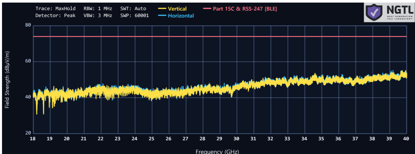
Plot 6-2 18 GHz to 40 GHz GHZ Worst case LE 1M SISO ANT1 2440 MHz
