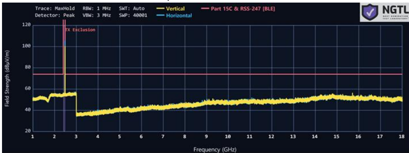
Plot 12-4 Radiated Spurious Emission - MIMO LE 2M 2478 MHz
