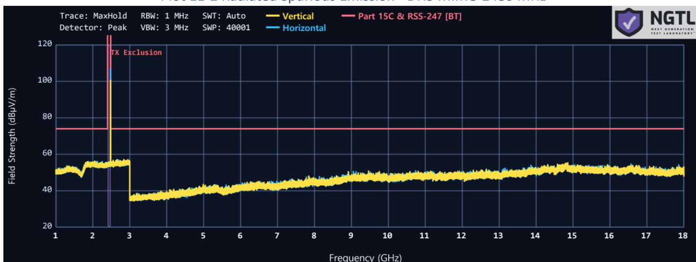
Plot 11-2 Radiated Spurious Emission - DH5 MIMO 2480 MHz
