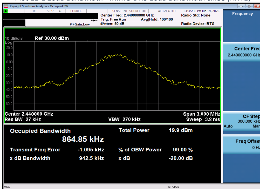
Plot 11-1 20dB Bandwidth - MIMO DH5 20dB Bandwidth ch.38 (ANT1)
