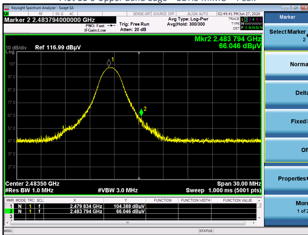
Plot 11-3 Upper Band Edge – 3DH5 MIMO – Peak
