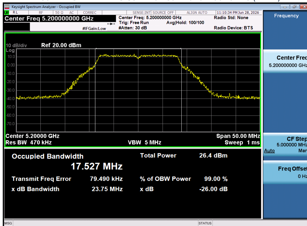
Plot 12-1 OFDM MIMO 802.11a 26dB Bandwidth ch.40 (ANT1)
