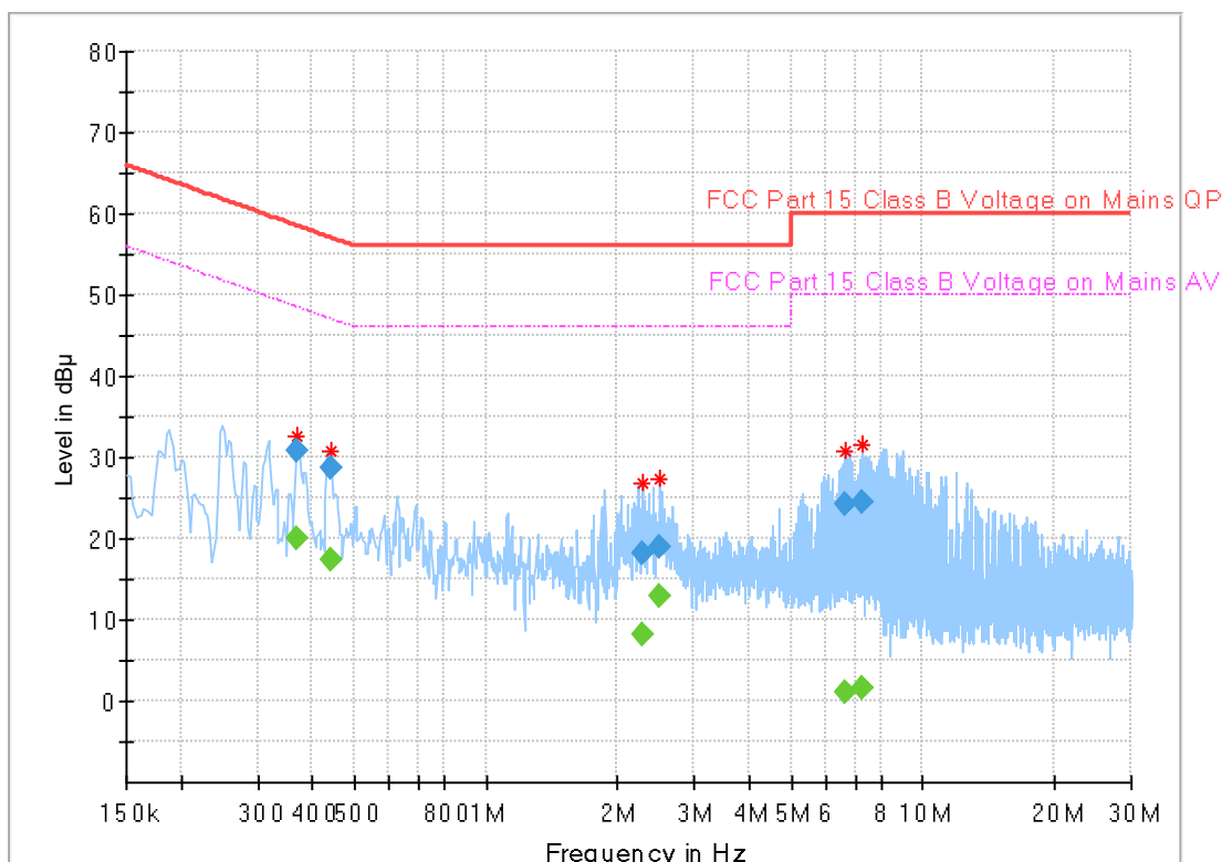
Plot 7-1 UNII 1 – Line L
