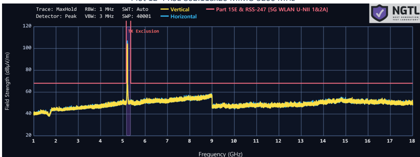
Plot 12-4 RSE 802.11ax20 MIMO 5200 MHz
