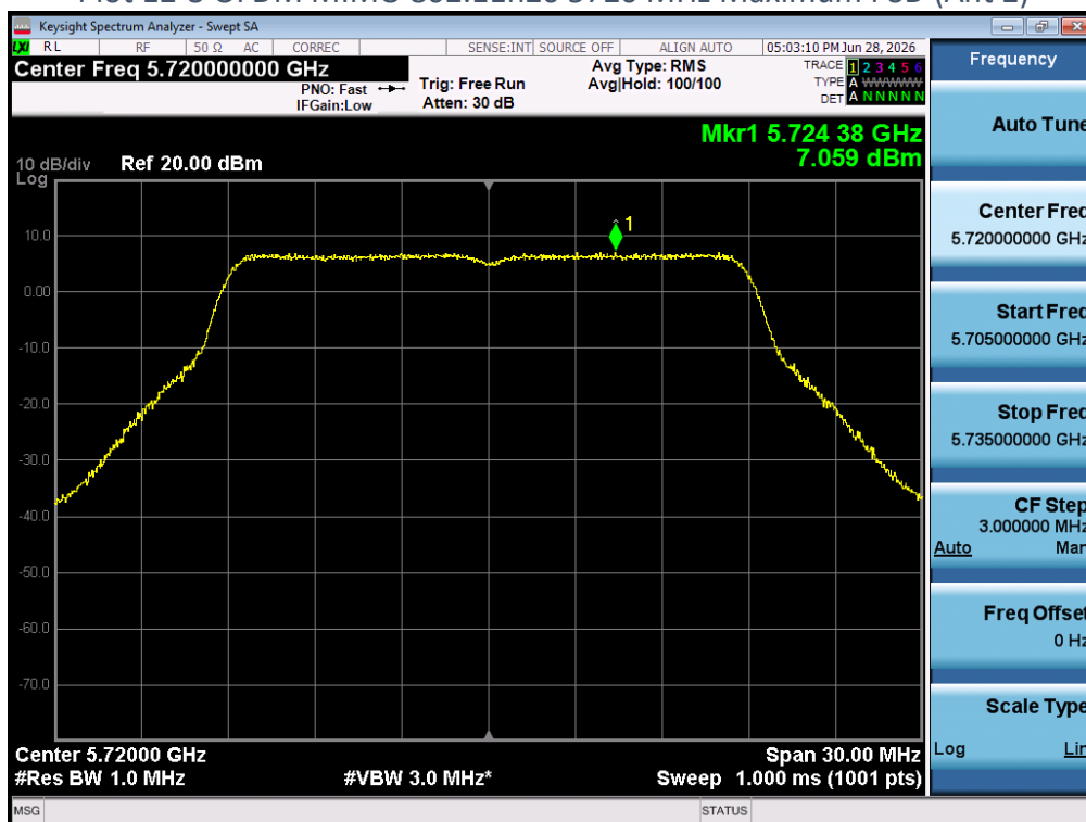
Plot 12-3 OFDM MIMO 802.11n20 5720 MHz Maximum PSD (Ant 2)
