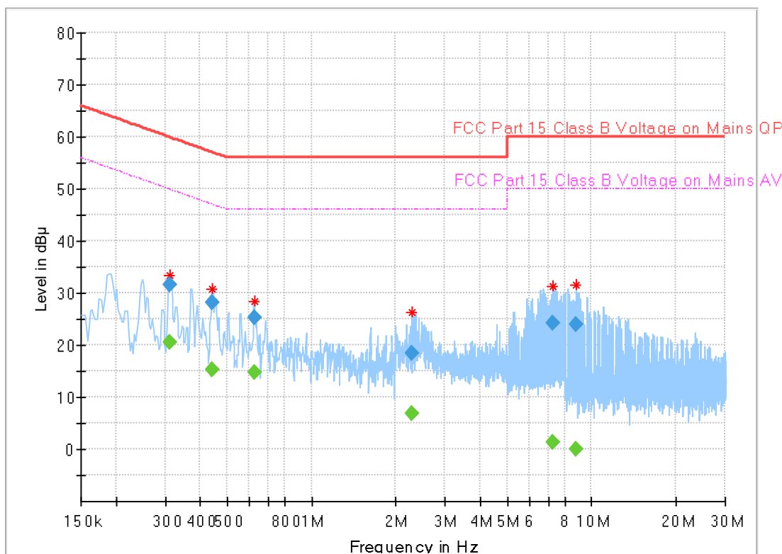
Plot 7-9 UNII 4 – Line L
