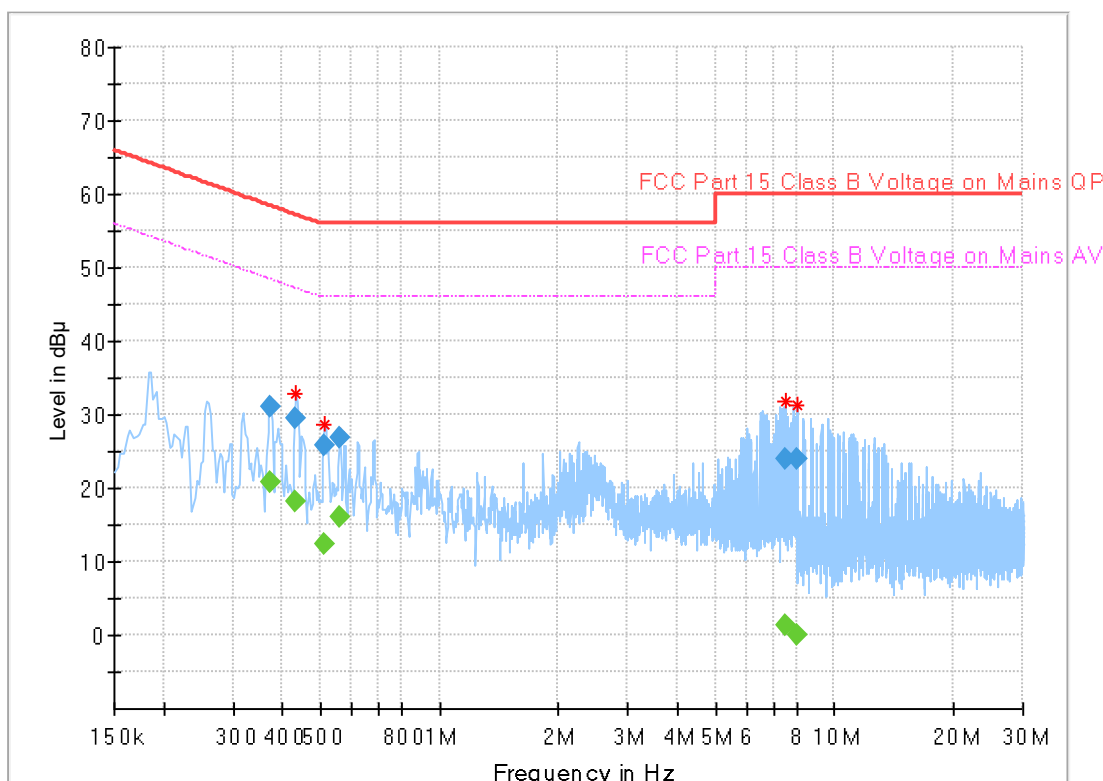
Plot 7-3 UNII 2A – Line L
