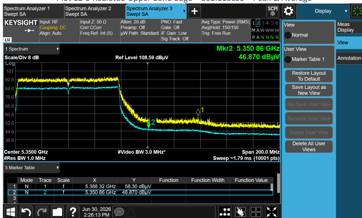
Plot 12-5 Radiated Upper Band Edge – 802.11ac80 – Peak & Average
