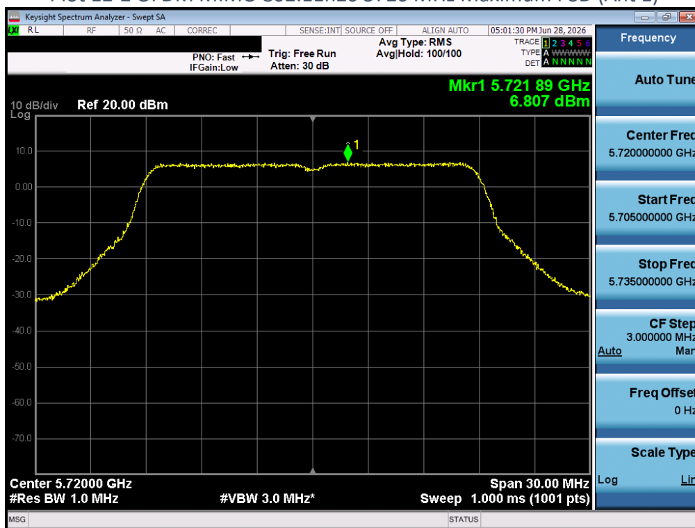
Plot 12-3 OFDM MIMO 802.11n20 5720 MHz Maximum PSD (Ant 2)
