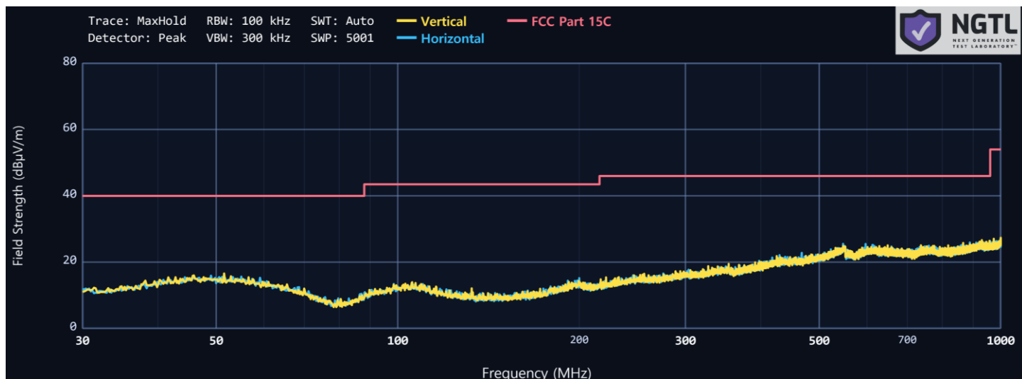
Plot 4-3 30 MHz to 1000 MHz Spurious Emission
