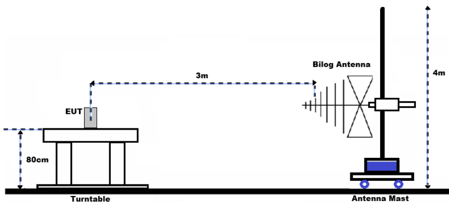
Figure 4-5 Radiated Measurement Setup Above 1 GHz
