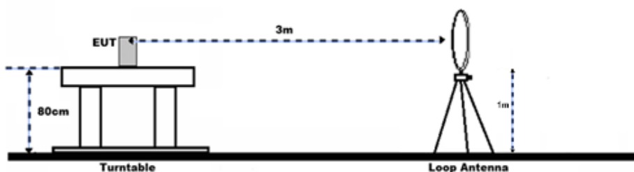
Figure 4-4 Radiated Measurement Setup Below 1 GHz
