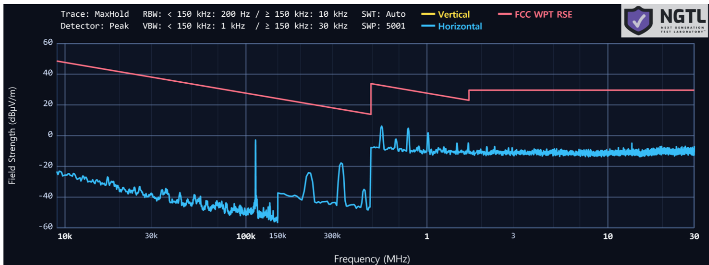
Plot 4-2 9 kHz to 30 MHz Spurious Emission
