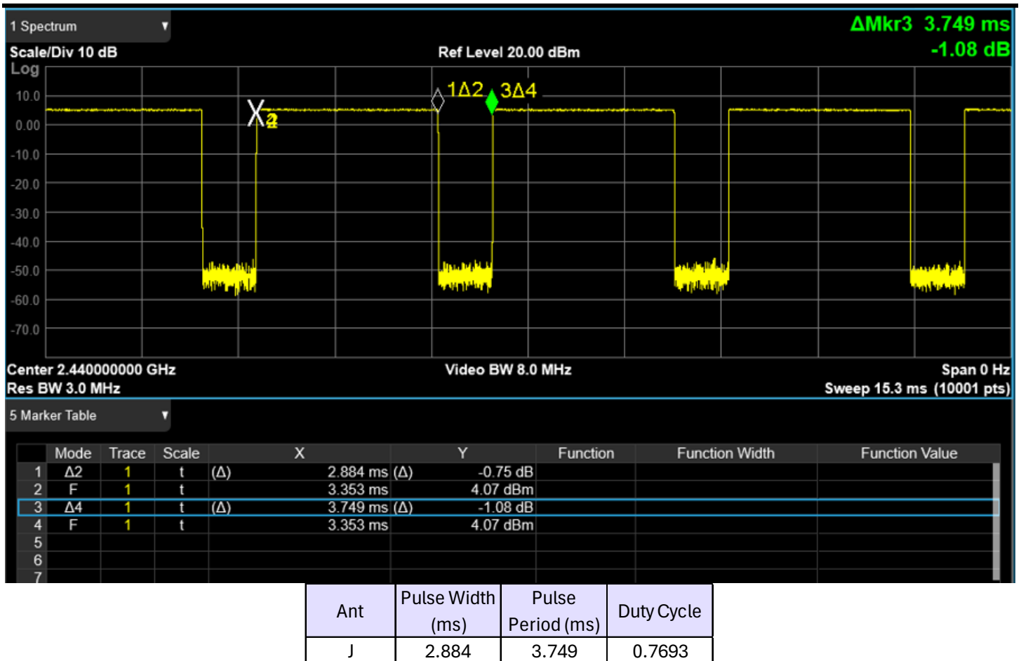
Figure 2-5 2.4 GHz Bluetooth Ant J Duty Cycle Plot and Calculation
