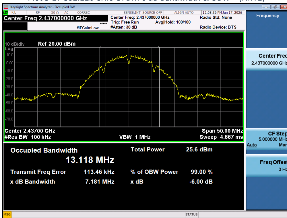
Plot 5-27 802.11b CH.6 OFDM 6 dB Bandwidth & OBW – (ANT1)
