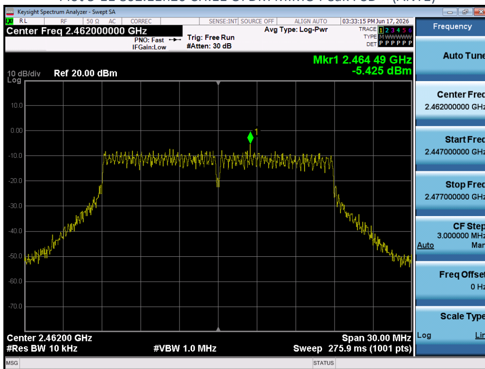
Plot 5-11 802.11n20 CH.11 OFDM MIMO Peak PSD – (ANT1)
