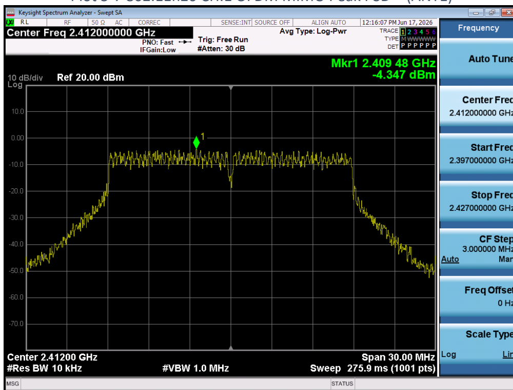
Plot 5-7 802.11n20 CH.1 OFDM MIMO Peak PSD – (ANT1)
