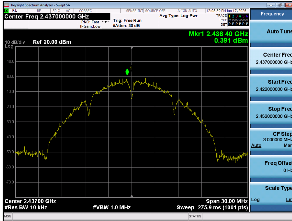
Plot 5-3 802.11b CH.6 OFDM MIMO Peak PSD – (ANT1)
