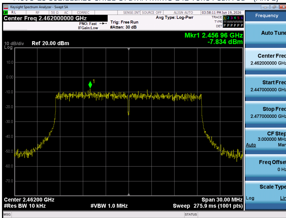
Plot 5-23 802.11ax20 CH.11 OFDMA MIMO 242 Tone Peak PSD - (Ant 1)
