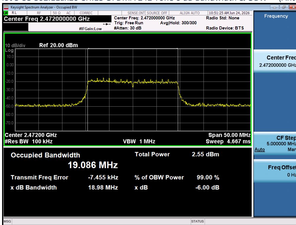
Plot 5-55 802.11ax20 CH.13 OFDMA 242 Tone 6 dB Bandwidth & OBW – (Ant 1)
