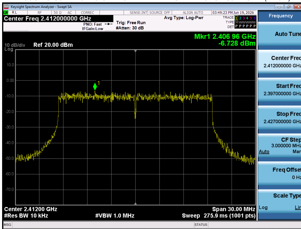
Plot 5-19 802.11ax20 CH.1 OFDMA MIMO 242 Tone Peak PSD - (Ant 1)
