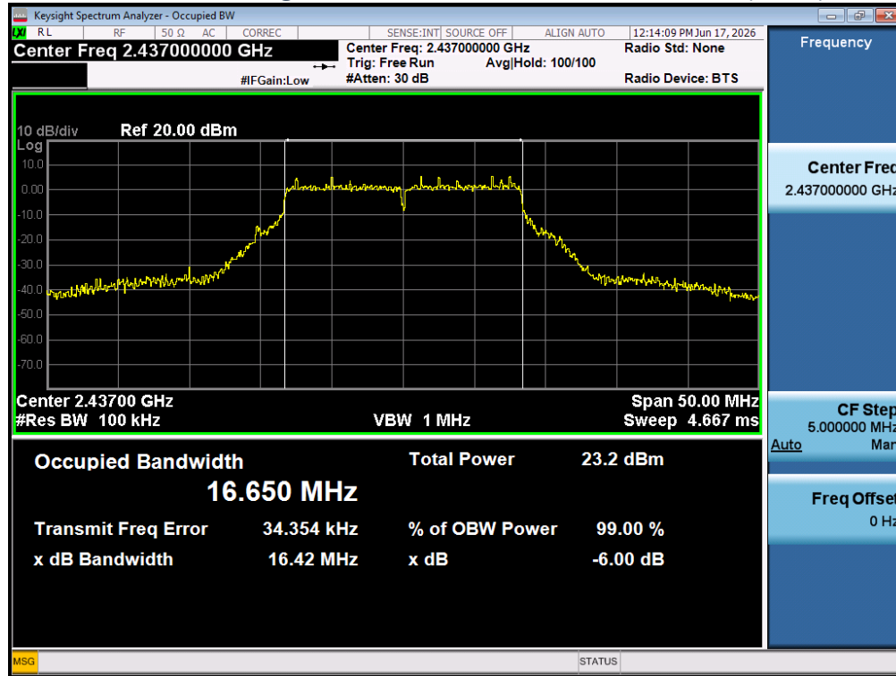
Plot 5-35 802.11g CH.6 OFDM 6 dB Bandwidth & OBW – (ANT1)
