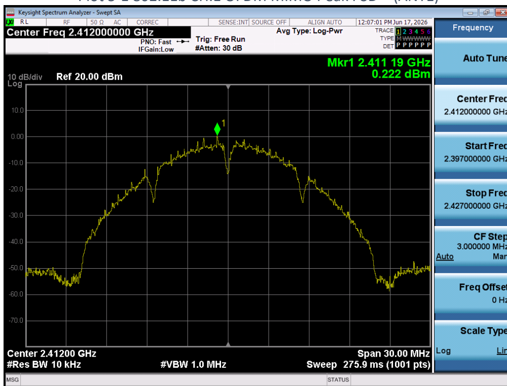
Plot 5-1 802.11b CH.1 OFDM MIMO Peak PSD – (ANT1)
