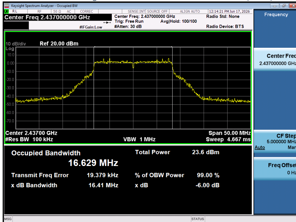
Plot 5-36 802.11g CH.6 OFDM 6 dB Bandwidth & OBW – (ANT2)
