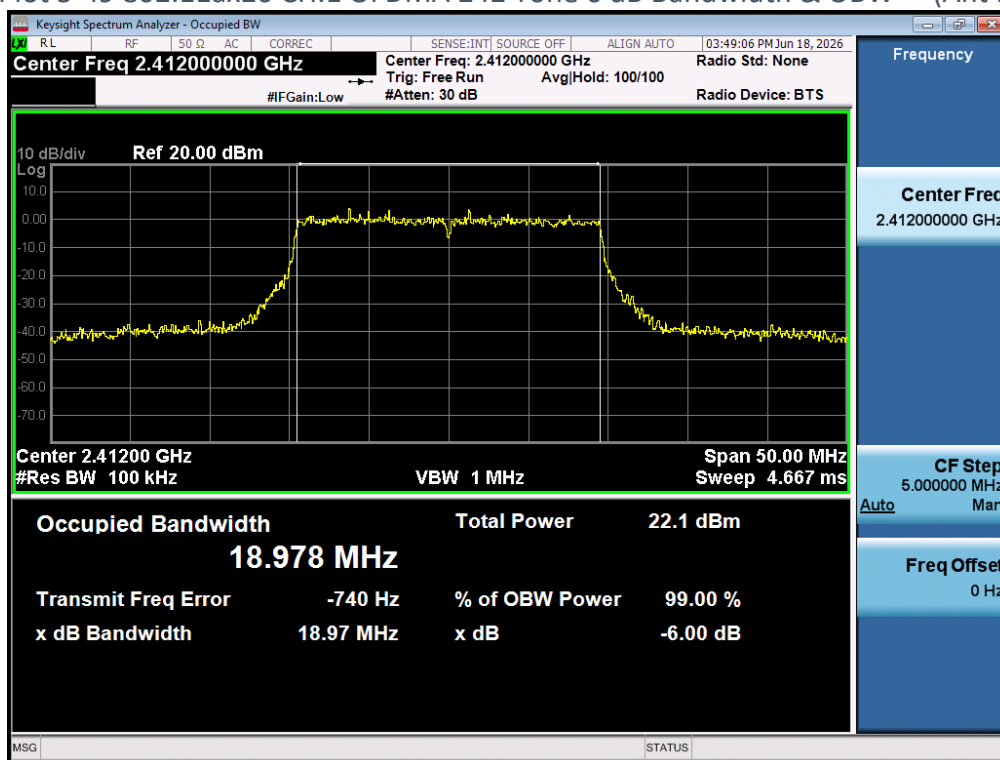
Plot 5-49 802.11ax20 CH.1 OFDMA 242 Tone 6 dB Bandwidth & OBW – (Ant 1)
