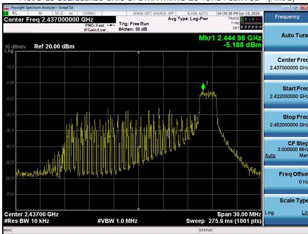
Plot 5-15 802.11ax20 CH.6 OFDMA MIMO 26 Tone Peak PSD - (Ant 1)
