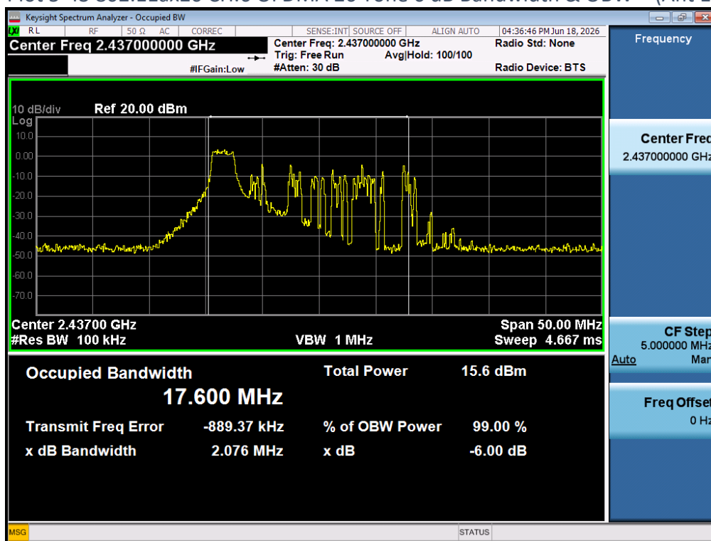
Plot 5-43 802.11ax20 CH.6 OFDMA 26 Tone 6 dB Bandwidth & OBW – (Ant 1)
