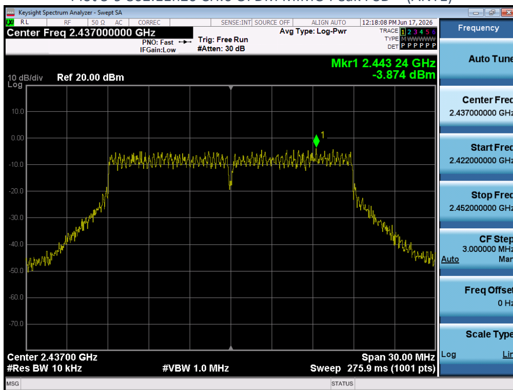
Plot 5-9 802.11n20 CH.6 OFDM MIMO Peak PSD – (ANT1)
