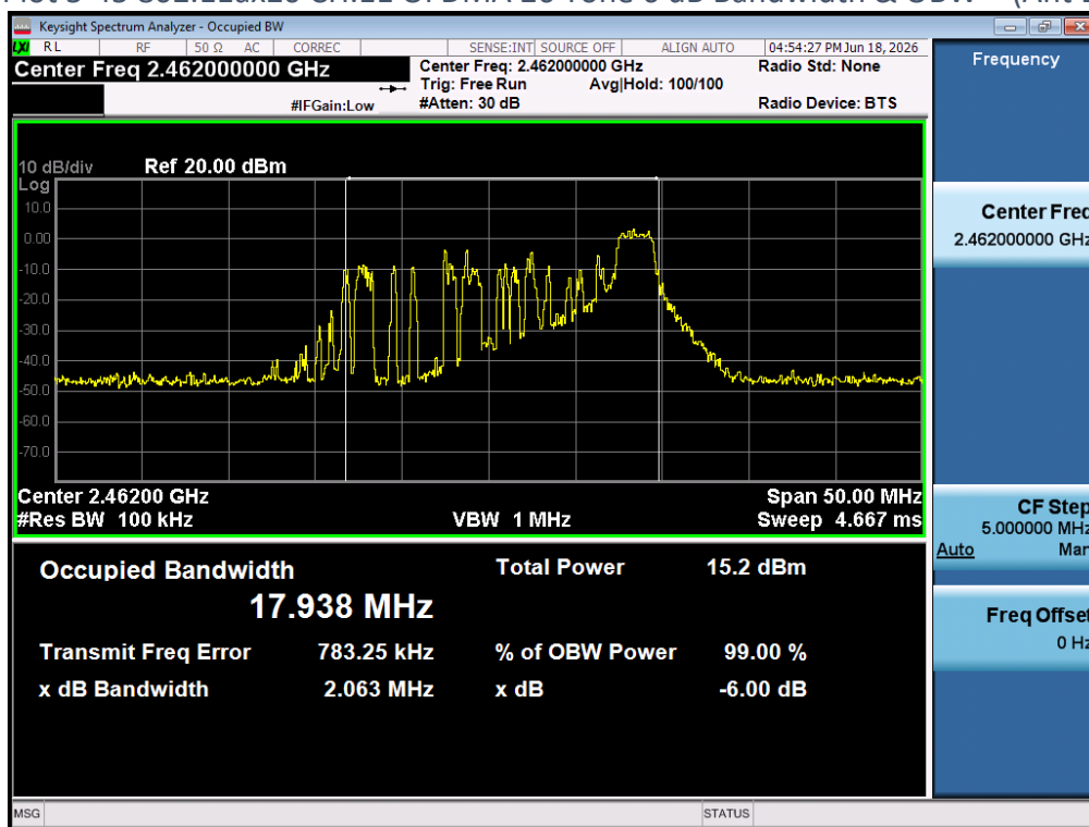
Plot 5-45 802.11ax20 CH.11 OFDMA 26 Tone 6 dB Bandwidth & OBW – (Ant 1)
