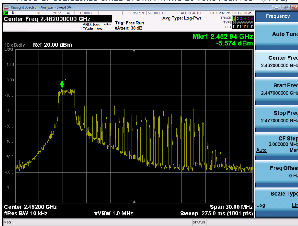
Plot 5-17 802.11ax20 CH.11 OFDMA MIMO 26 Tone Peak PSD - (Ant 1)
