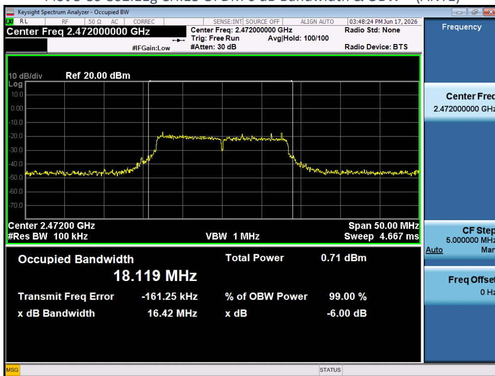
Plot 5-39 802.11g CH.13 OFDM 6 dB Bandwidth & OBW – (ANT1)
