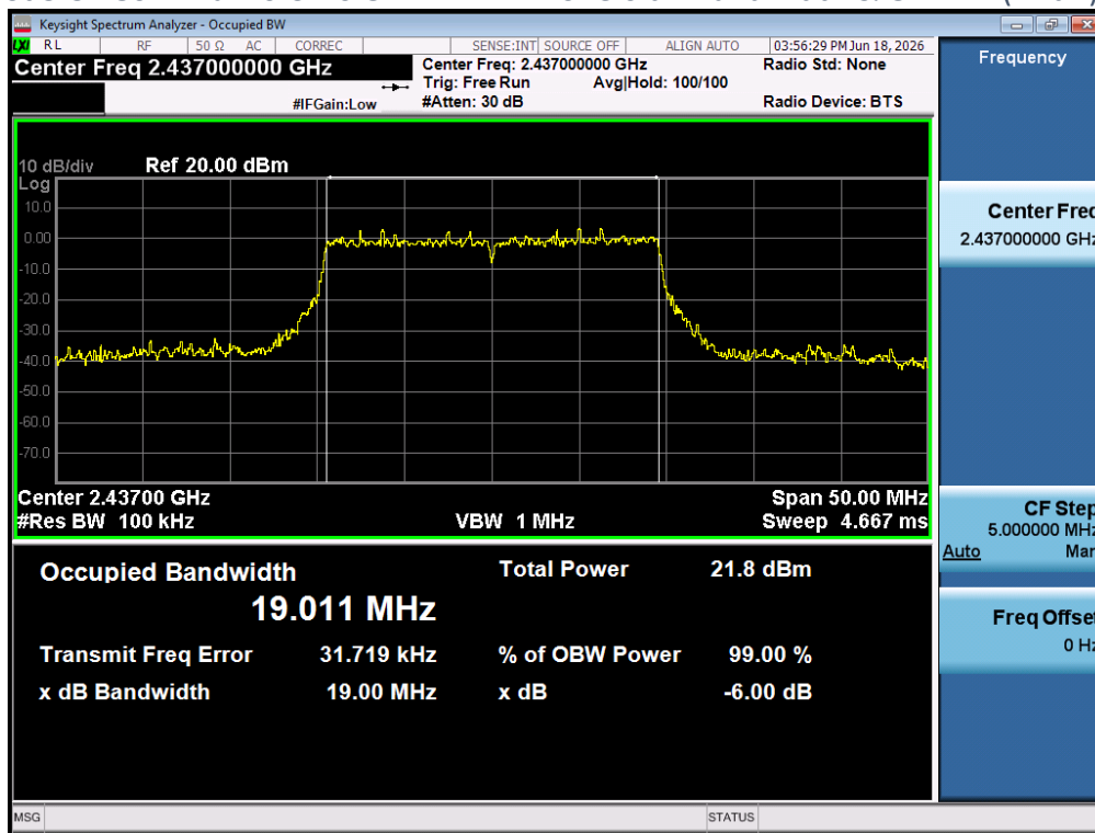
Plot 5-51 802.11ax20 CH.6 OFDMA 242 Tone 6 dB Bandwidth & OBW – (Ant 1)
