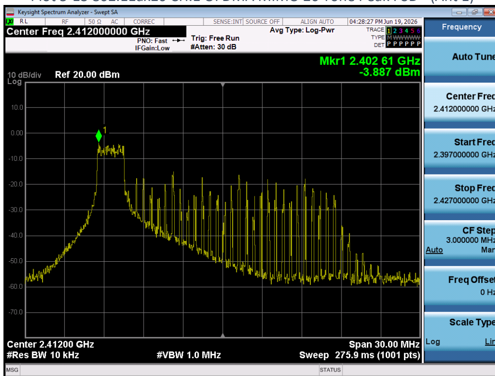
Plot 5-13 802.11ax20 CH.1 OFDMA MIMO 26 Tone Peak PSD - (Ant 1)
