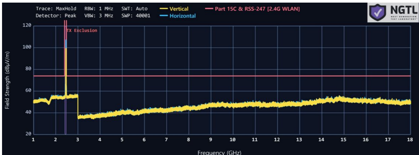
Plot 6-5 1 GHz to 18 GHz 802.11n(HT20) 2462 MHz
