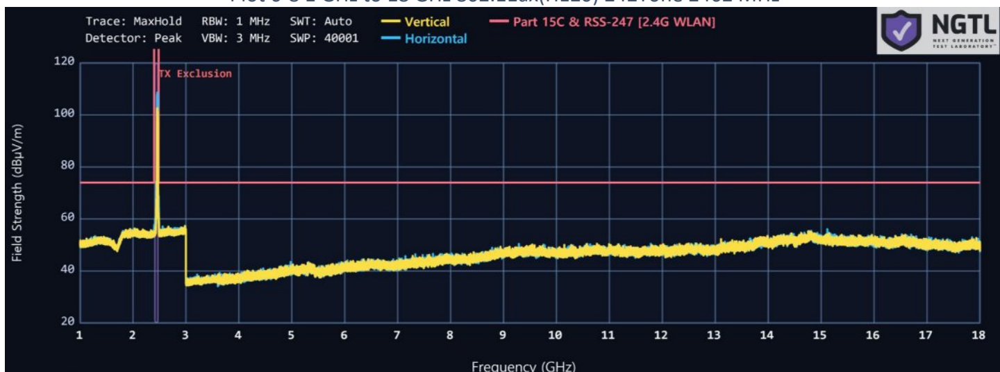
Plot 6-8 1 GHz to 18 GHz 802.11ax(HE20) 242Tone 2462 MHz
