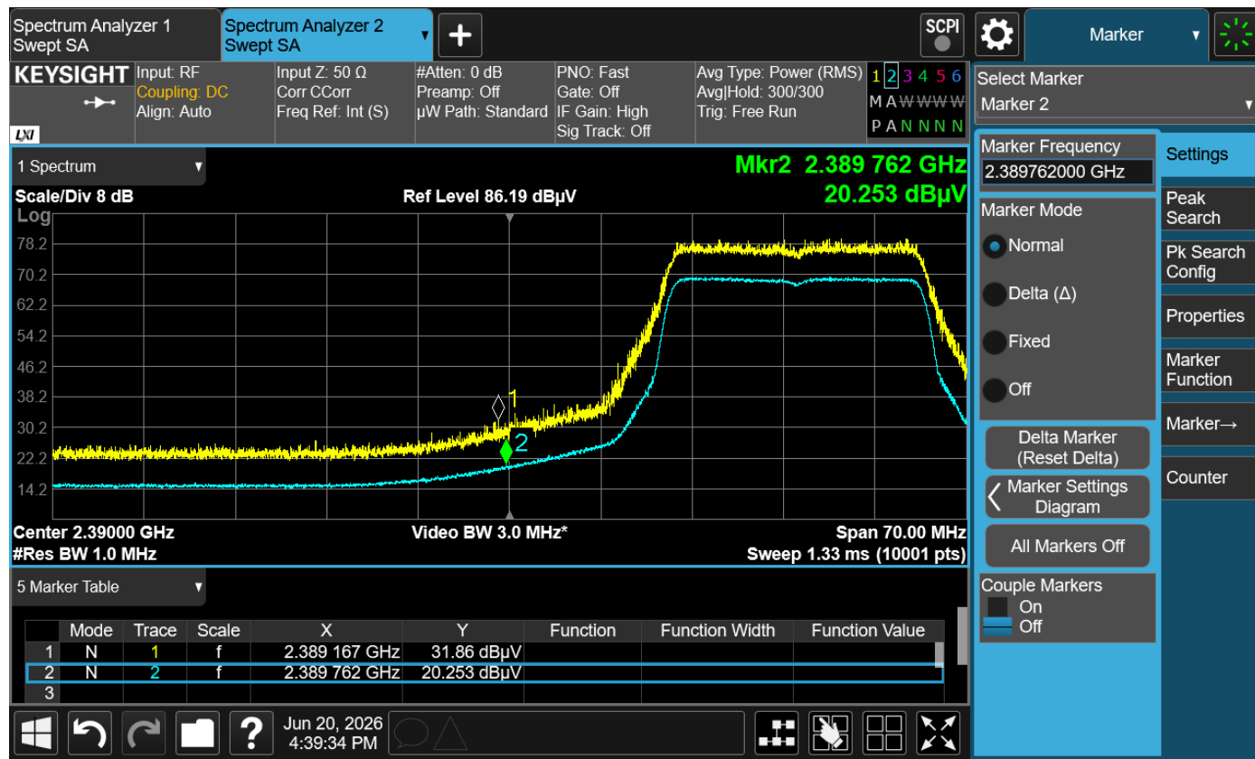
Plot 6-9 Lower Band Edge – 802.11ax20 OFDM – Peak & Average
