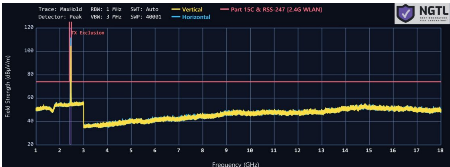
Plot 6-3 1 GHz to 18 GHz 802.11b 2462 MHz
