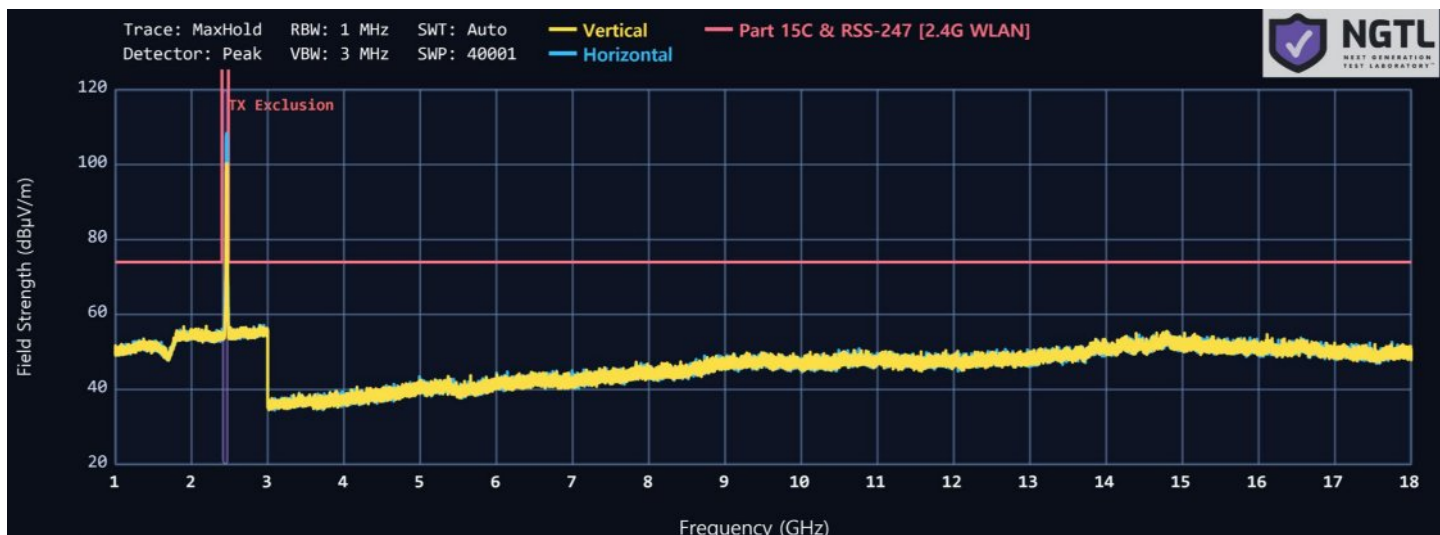
Plot 6-4 1 GHz to 18 GHz 802.11g 2462 MHz
