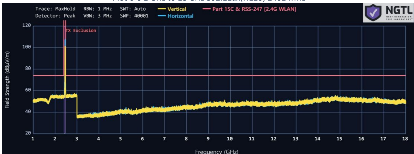
Plot 6-6 1 GHz to 18 GHz 802.11ax(HE20) 2462 MHz
