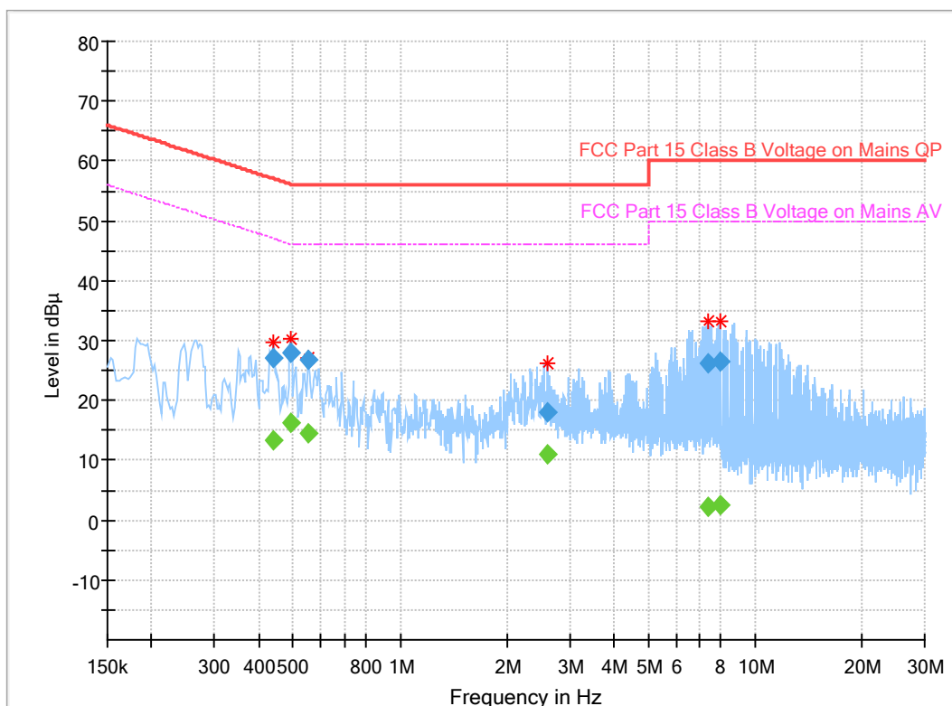
Plot 7-2 2.4G WLAN – Line N
