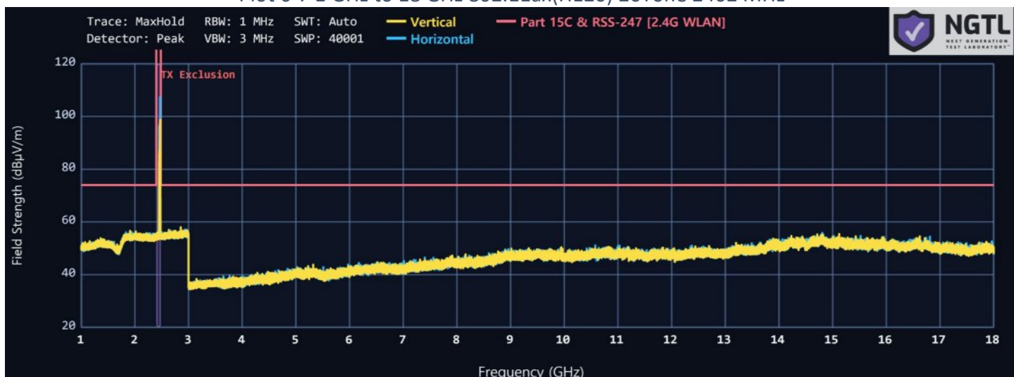
Plot 6-7 1 GHz to 18 GHz 802.11ax(HE20) 26Tone 2462 MHz
