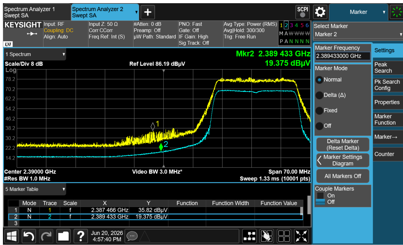
Plot 6-10 Lower Band Edge – 802.11ax20 OFDMA 242 Tone – Peak & Average
