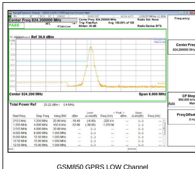
GSM850 GPRS LOW Channel
