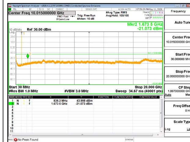
GSM850 GPRS MID Channel
