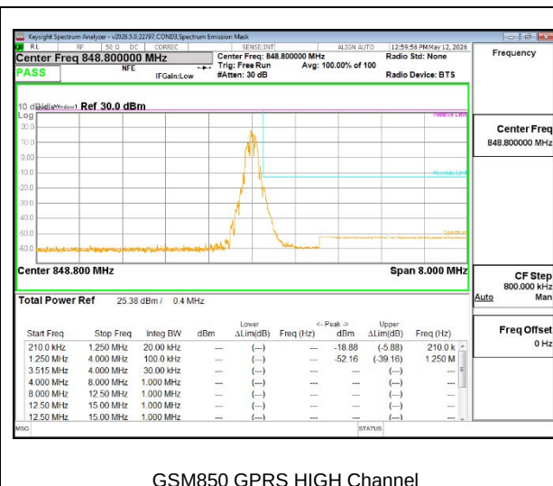
GSM850 GPRS HIGH Channel
