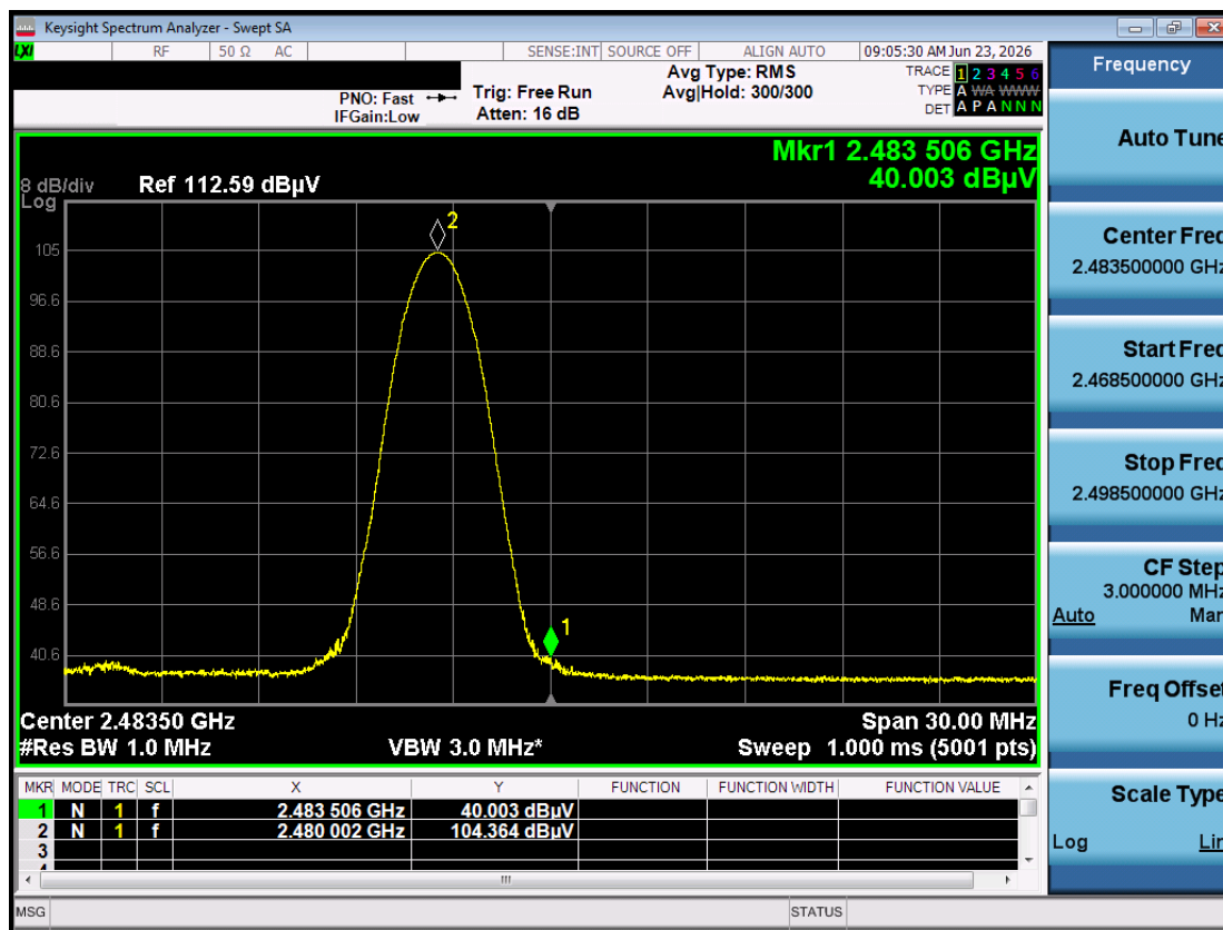
Plot 6-11 Upper Band Edge – LE 1M MIMO 2480 MHz – Average
