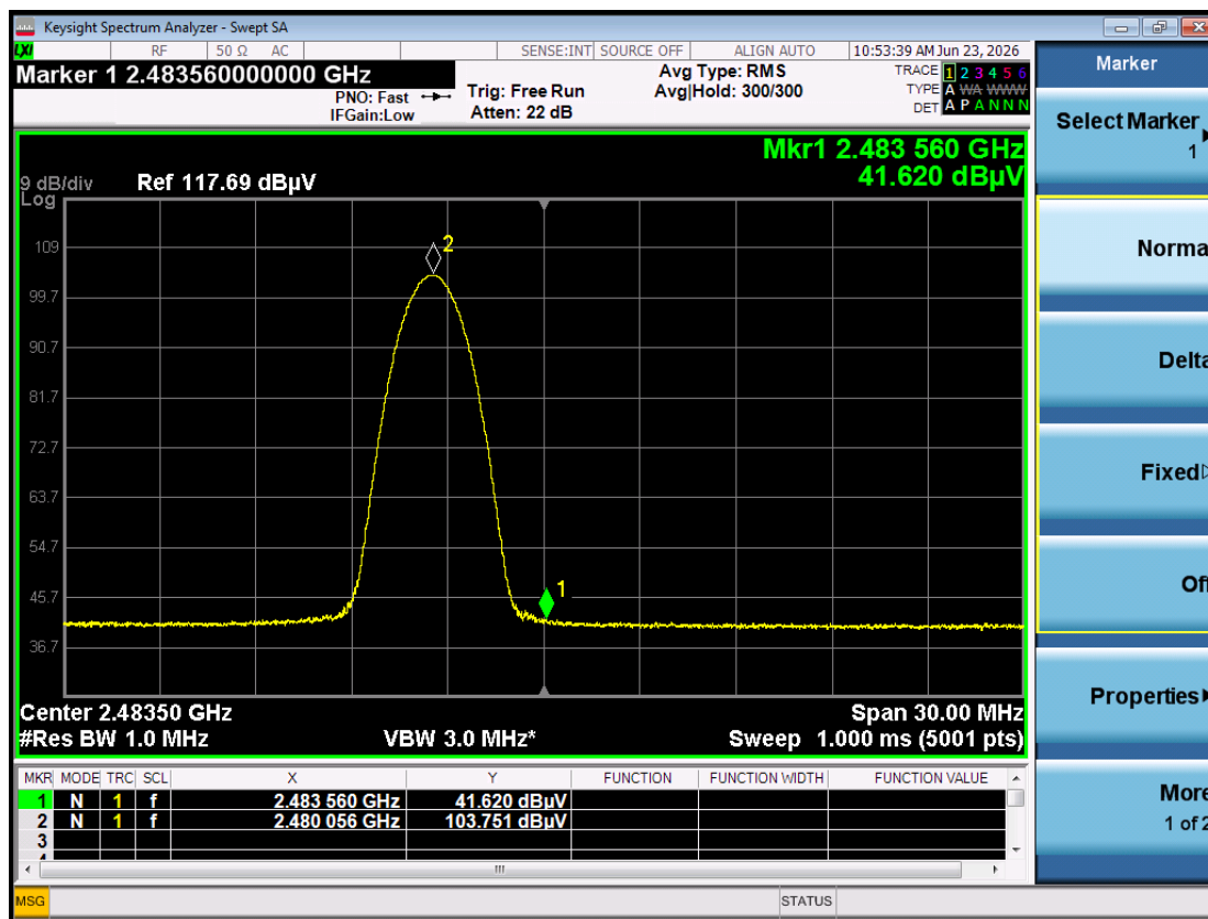
Plot 6-9 Upper Band Edge – LE 1M SISO ANT2 2480 MHz – Average
