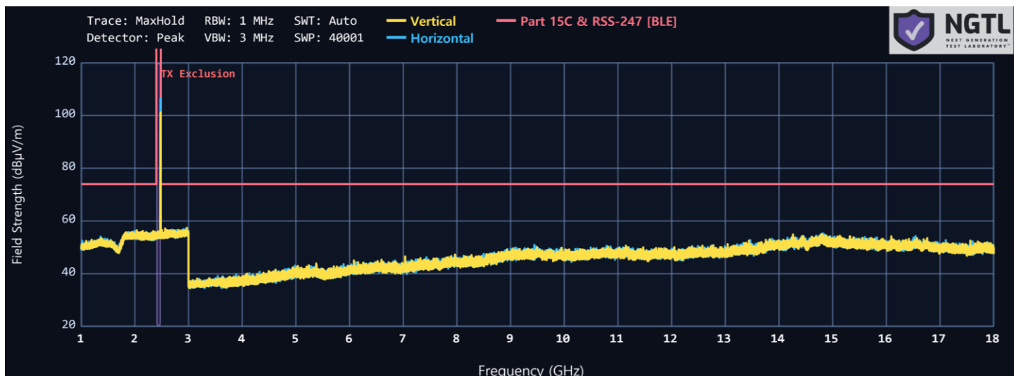
Plot 6-5 1 GHz to 18 GHz LE 2M MIMO 2478 MHz
