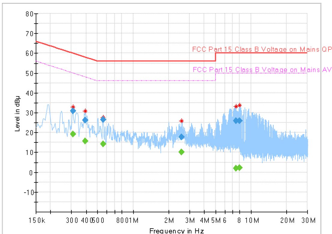
Plot 7-2 LE – Line N
