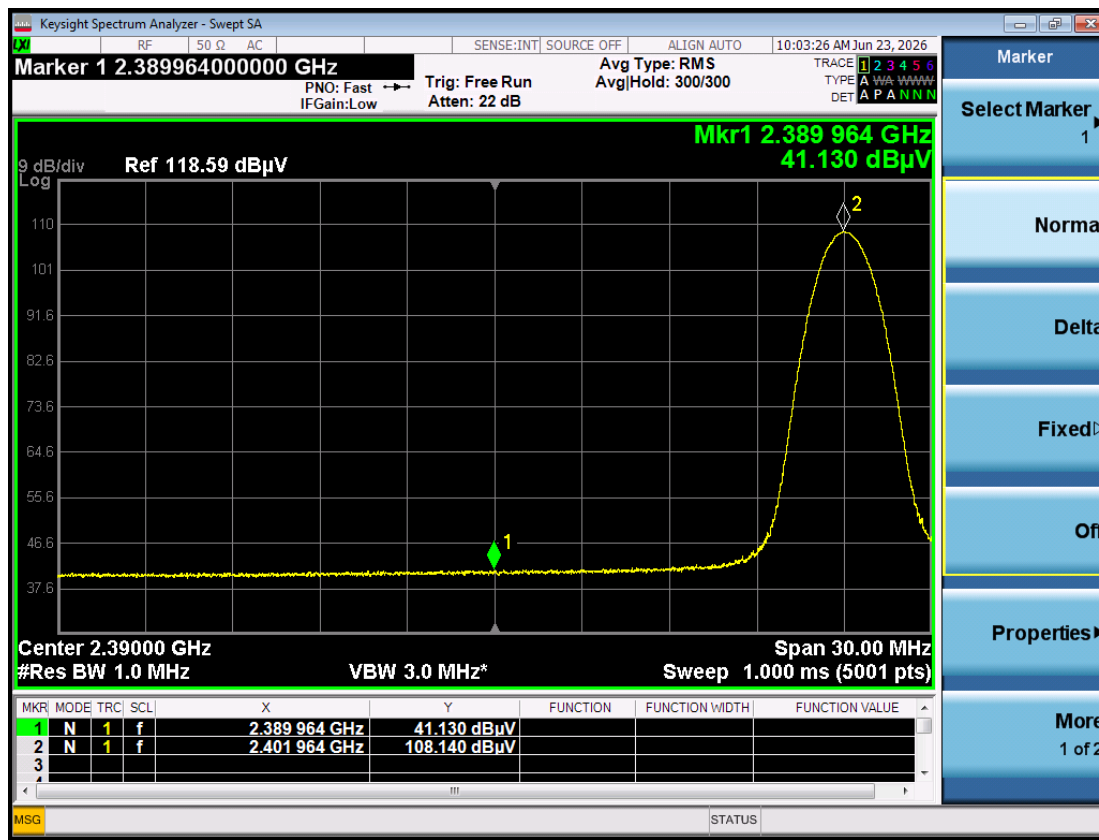
Plot 6-6 Lower Band Edge – LE 1M SISO ANT1 2402 MHz – Average
