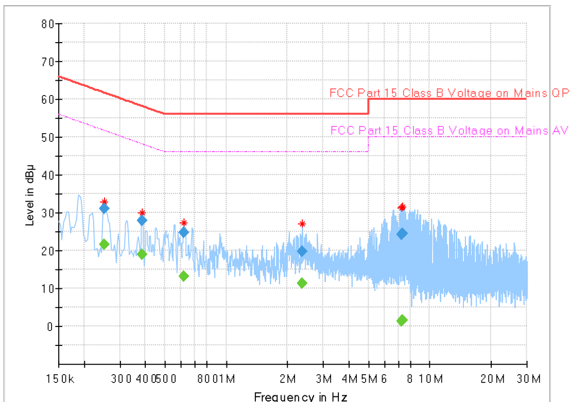
Plot 7-1 LE – Line L
