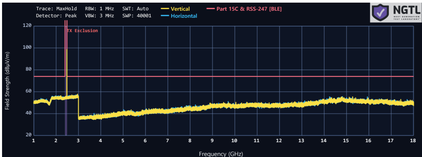
Plot 6-4 1 GHz to 18 GHz LE 1M SISO ANT2 2480 MHz
