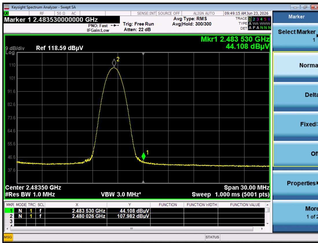
Plot 6-7 Upper Band Edge – LE 1M SISO ANT1 2480 MHz – Average
