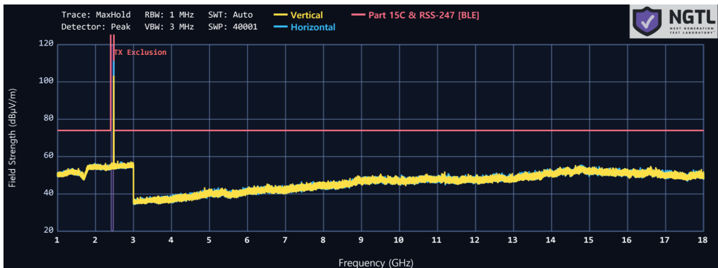
Plot 6-3 1 GHz to 18 GHz LE 1M SISO ANT1 2480 MHz
