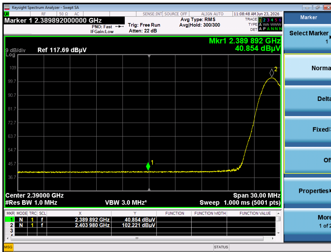
Plot 6-8 Lower Band Edge – LE 2M SISO ANT2 2404 MHz – Average
