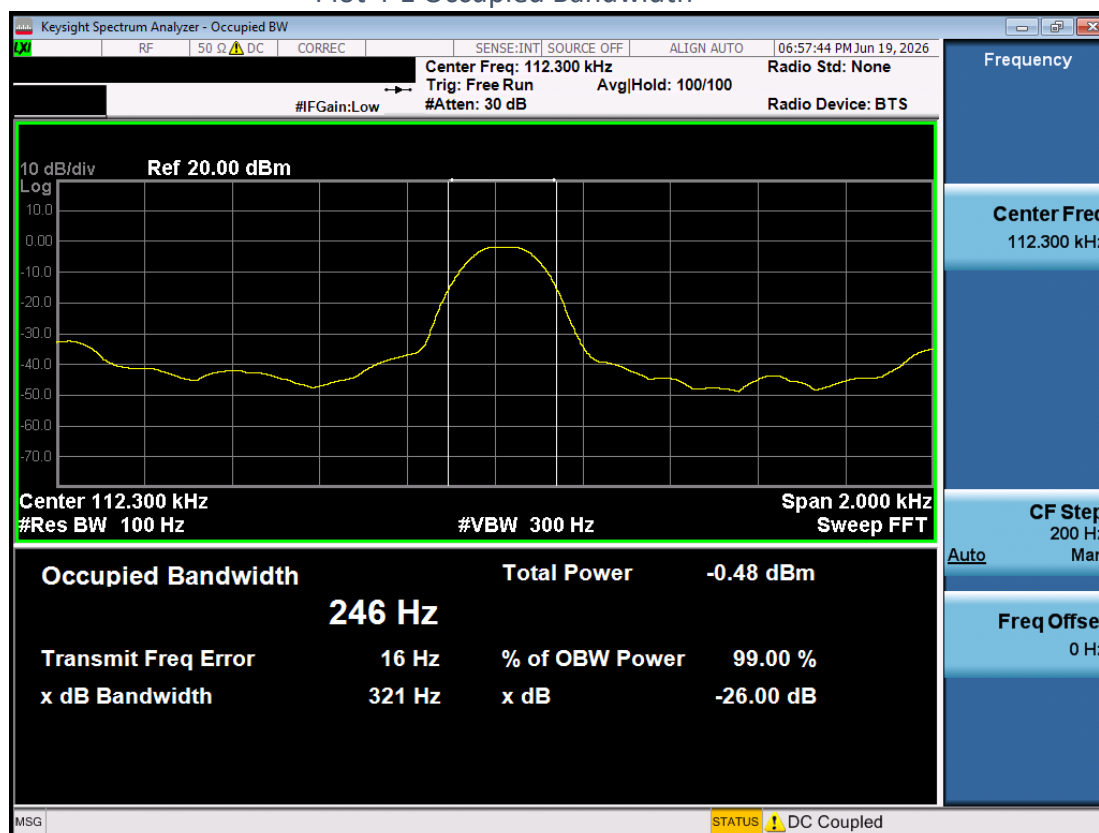
Plot 4-1 Occupied Bandwidth
