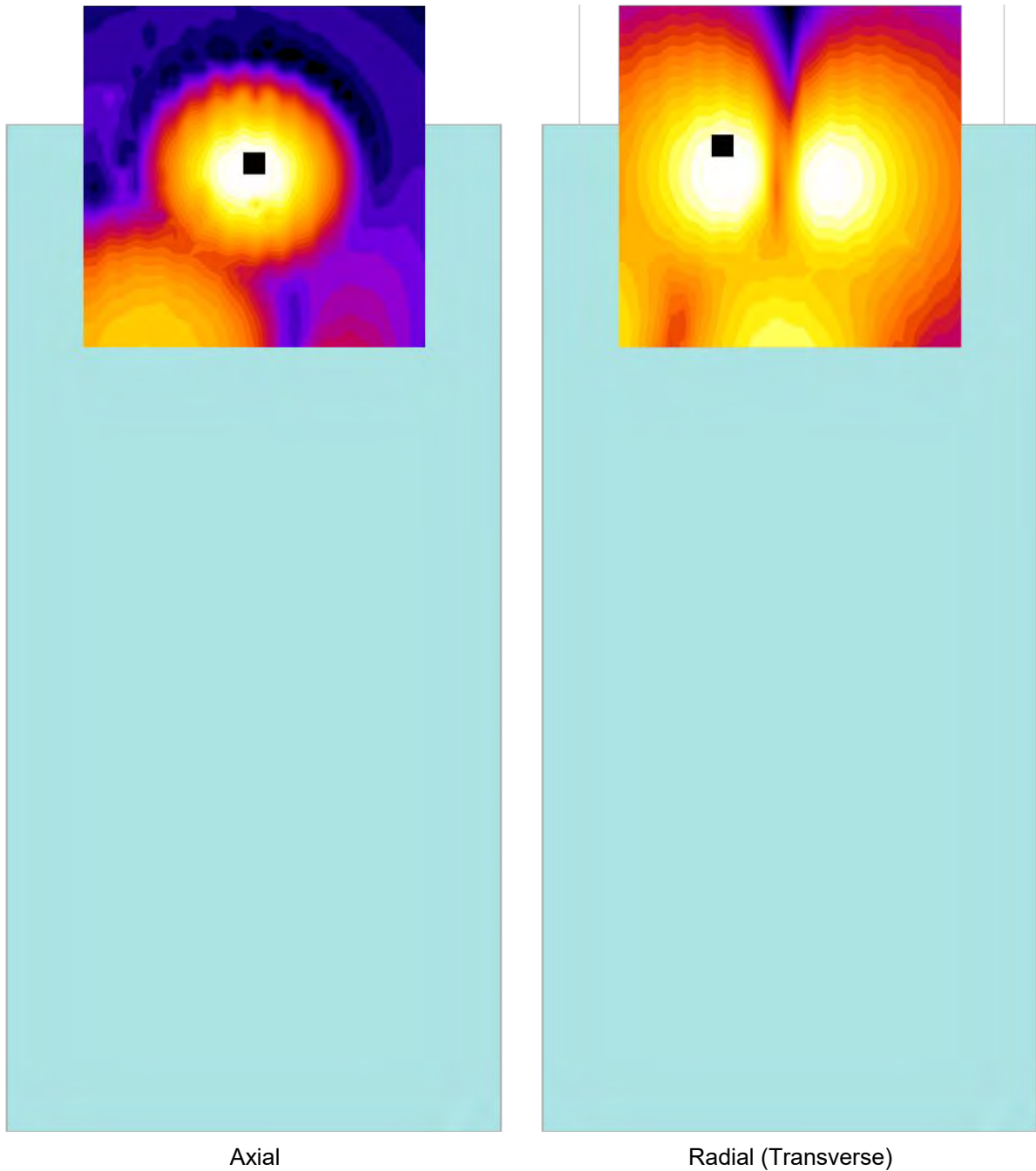
Figure 9-1 T-Coil Scan Overlay Magnetic Field Distributions
