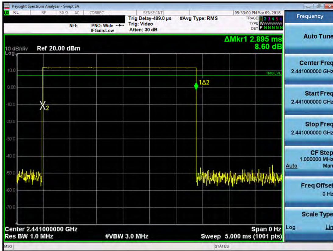
Plot 7-33. Time of Occupancy Plot (Bluetooth)
