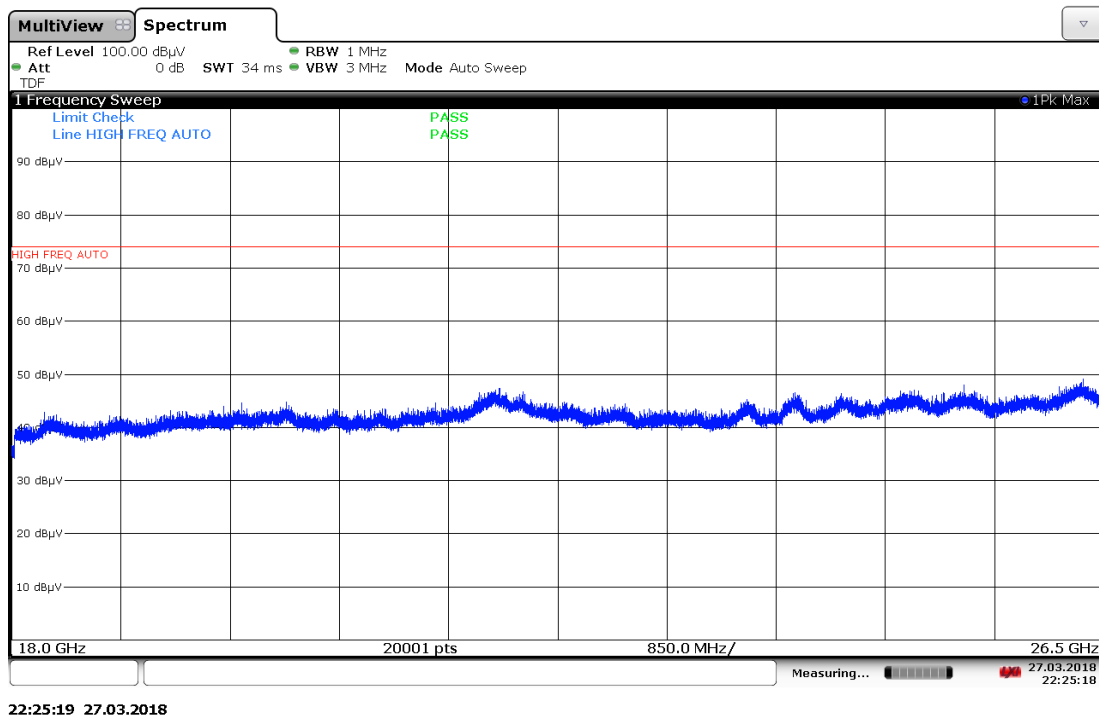
Plot 7-83. Radiated Spurious Plot 18GHz - 26.5GHz (802.11a) – Horizontal
