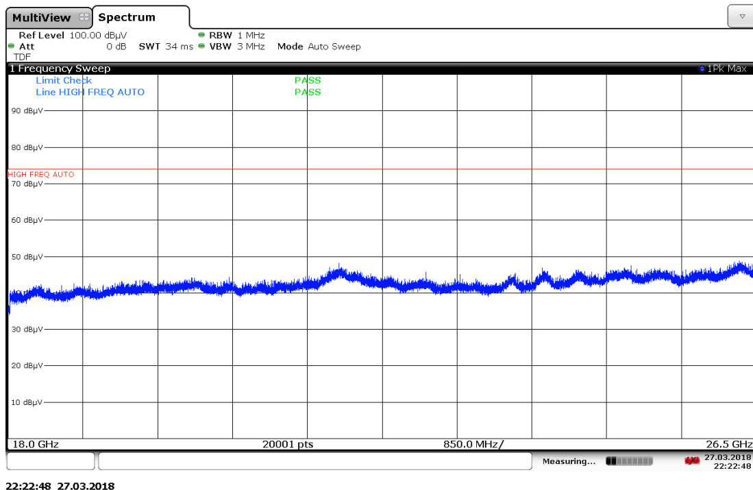
Plot 7-84. Radiated Spurious Plot 18GHz - 26.5GHz (802.11a) – Vertical
