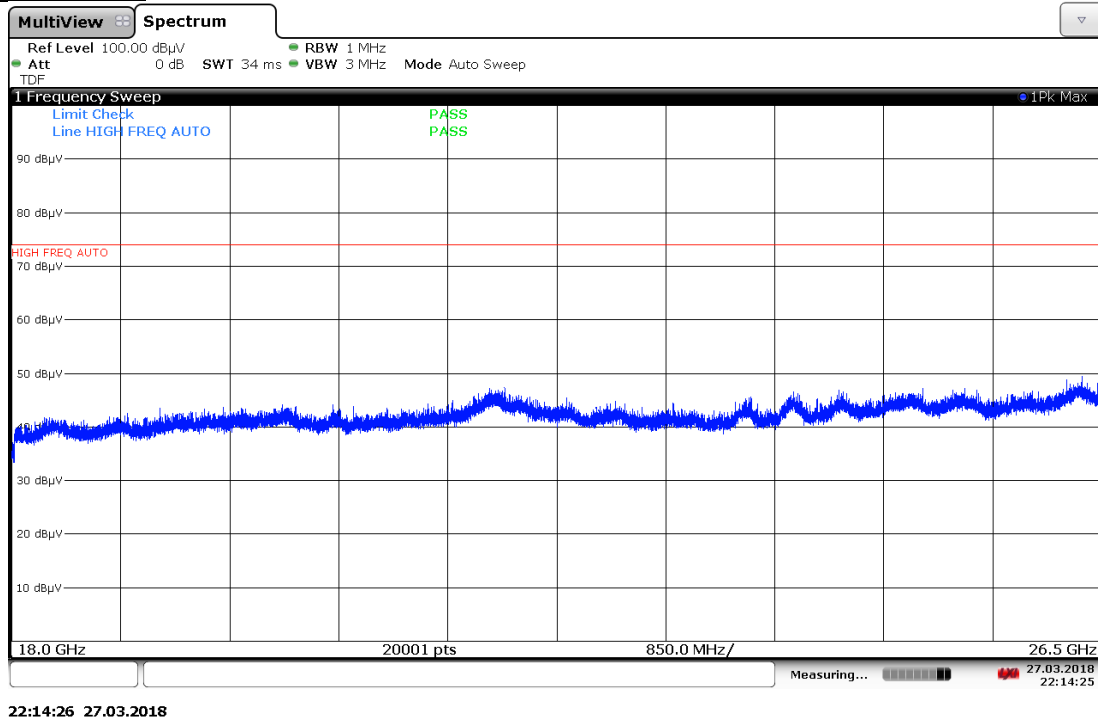
Plot 7-34. Radiated Spurious Plot above 18GHz – Horizontal
