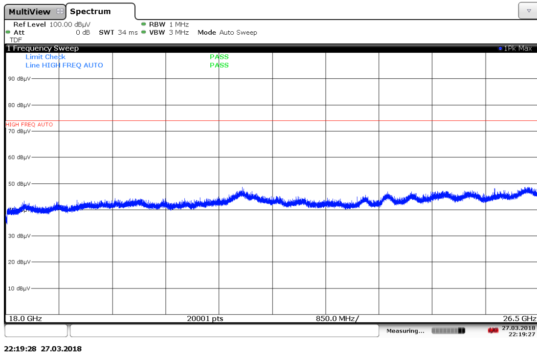
Plot 7-35. Radiated Spurious Plot above 18GHz – Vertical
