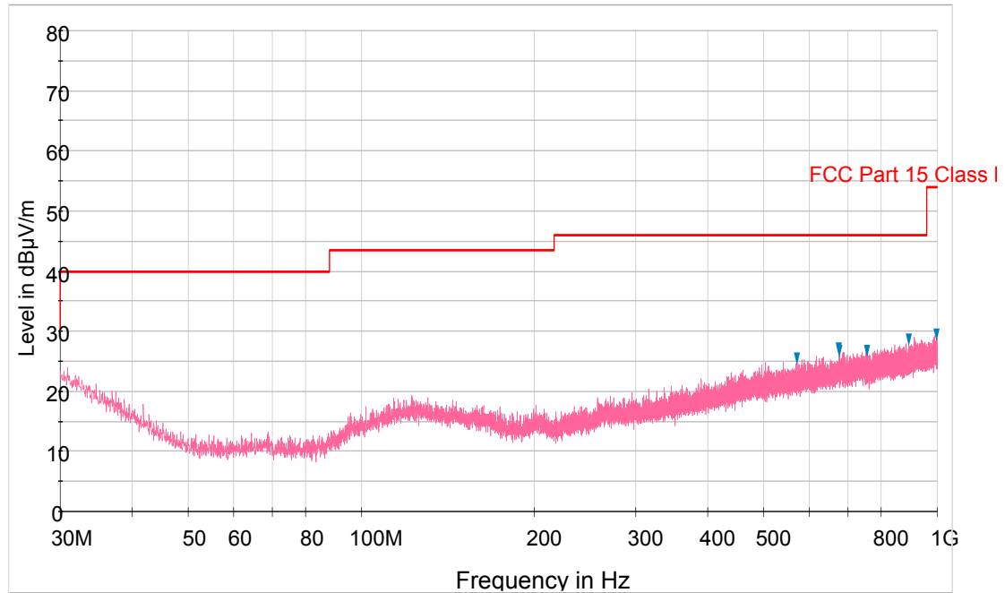
Plot 6-43. Radiated Spurious Plot below 1GHz (Pol. H)
