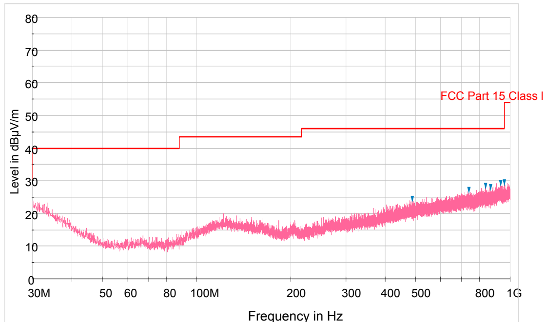
Plot 6-44. Radiated Spurious Plot below 1GHz (Pol. V)
