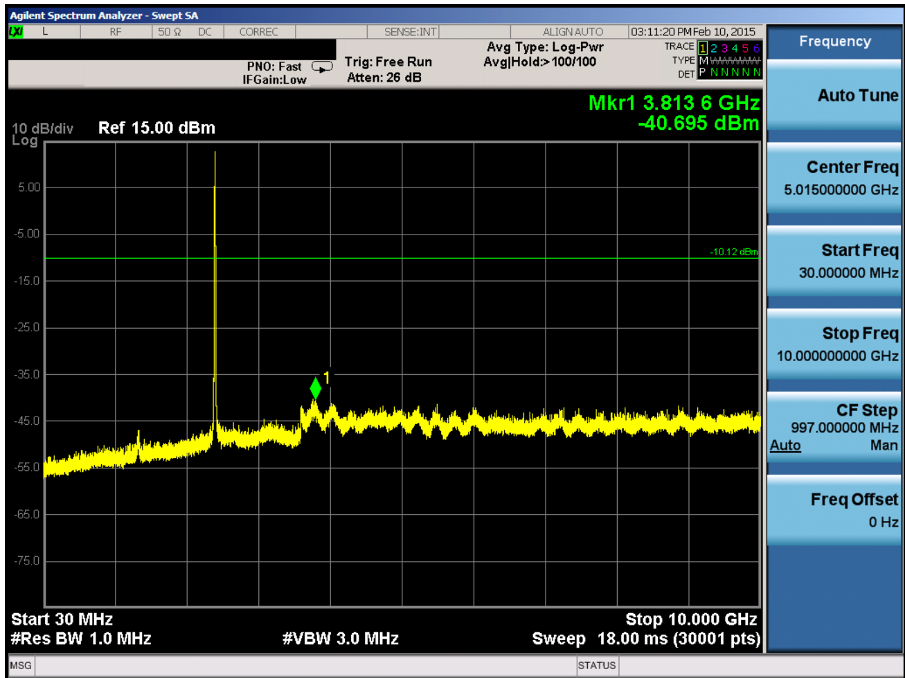
Plot 6-25. Conducted Spurious Plot (802.11b – Ch. 1)
