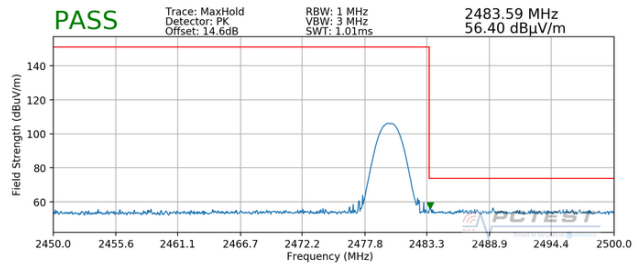
Plot 7-49. Radiated Restricted Upper Band Edge Measurement with WCP (Peak)
