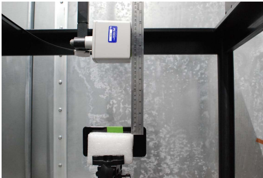
Test Setup Photo 30 E-field, Left edge, 15cm
