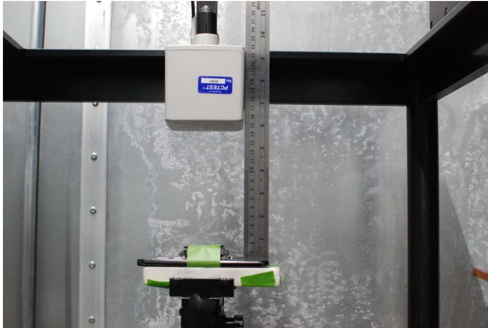
Test Setup Photo 19 H-field, Back side, 15cm
