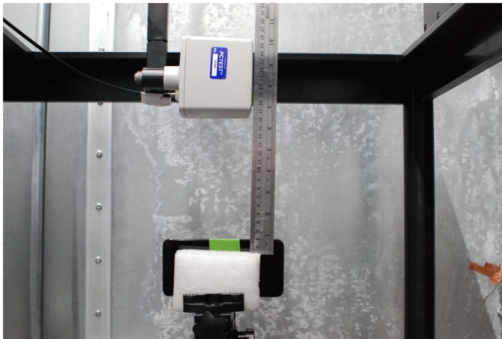
Test Setup Photo 18 E-field, Left edge, 15cm
