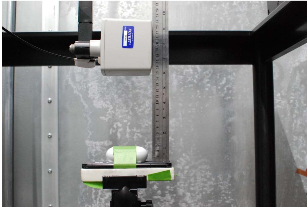
Test Setup Photo 25 E-field, Back side, 15cm
