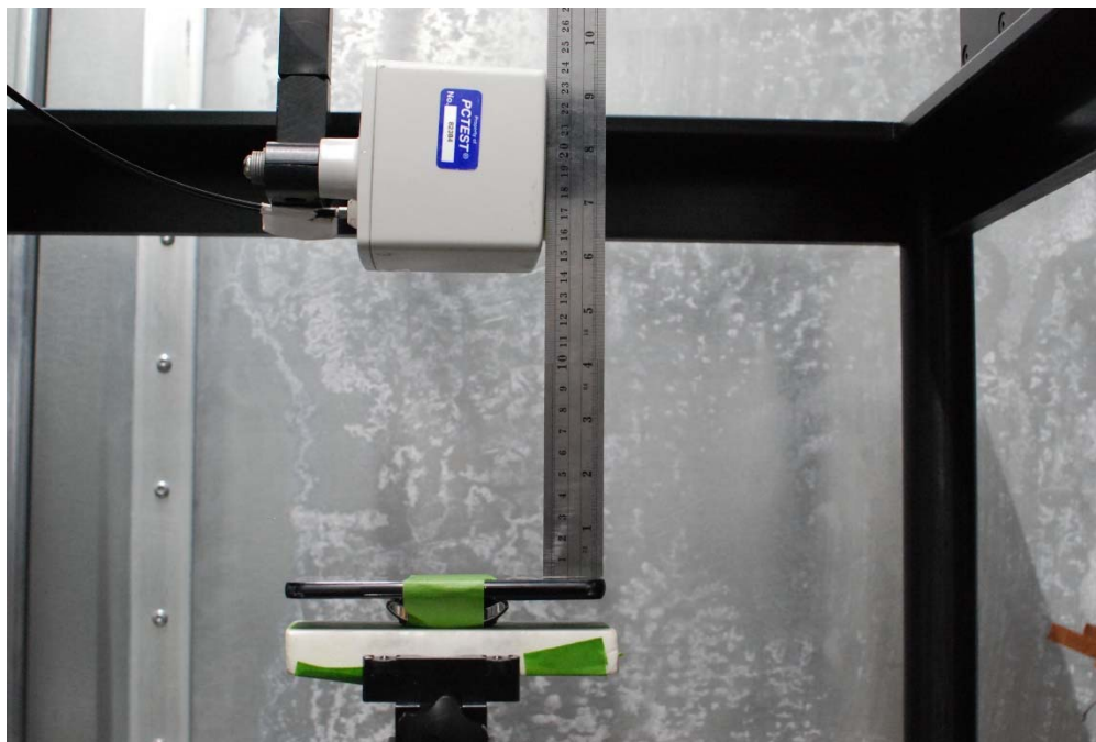
Test Setup Photo 14 E-field, Front side, 15cm
