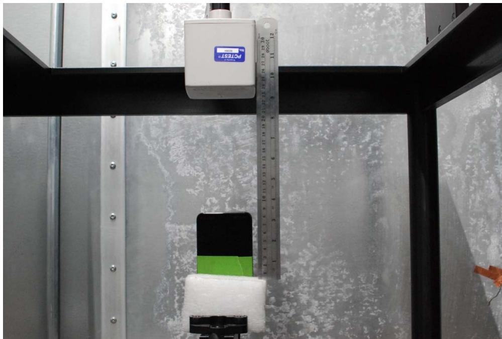
Test Setup Photo 34 H-field, Bottom edge, 15cm
