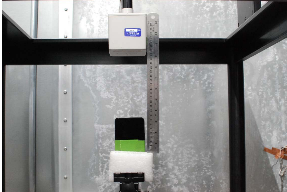
Test Setup Photo 33 H-field, Top edge, 15cm
