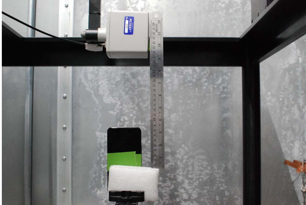
Test Setup Photo 15 E-field, Top edge, 15cm
