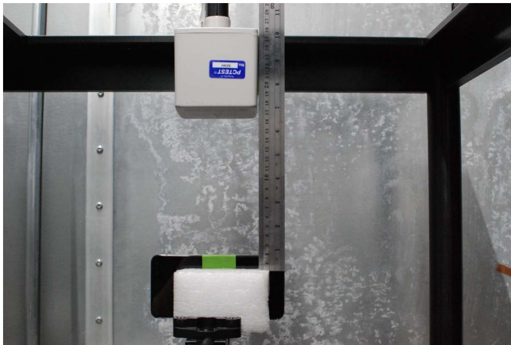
Test Setup Photo 36 H-field, Left edge, 15cm
