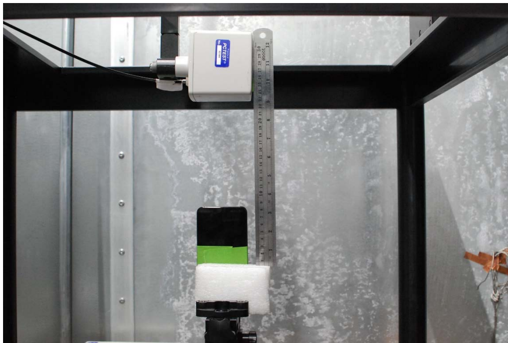
Test Setup Photo 16 E-field, Bottom edge, 15cm
