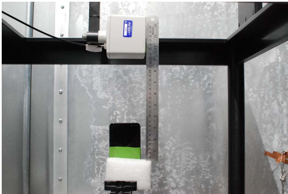
Test Setup Photo 28 E-field, Bottom edge, 15cm
