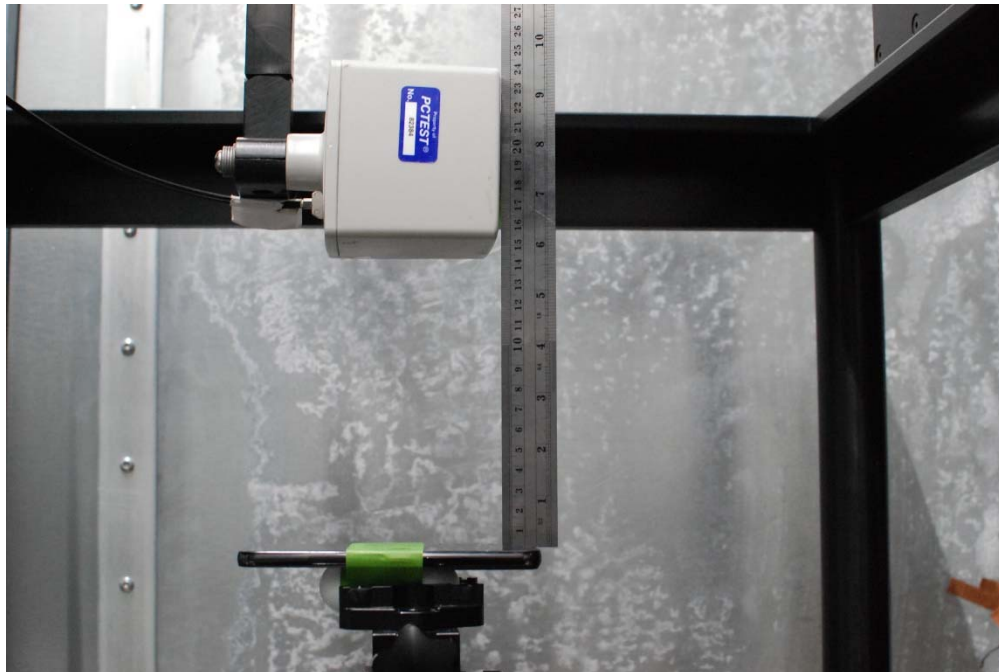
Test Setup Photo 26 E-field, Front side, 15cm
