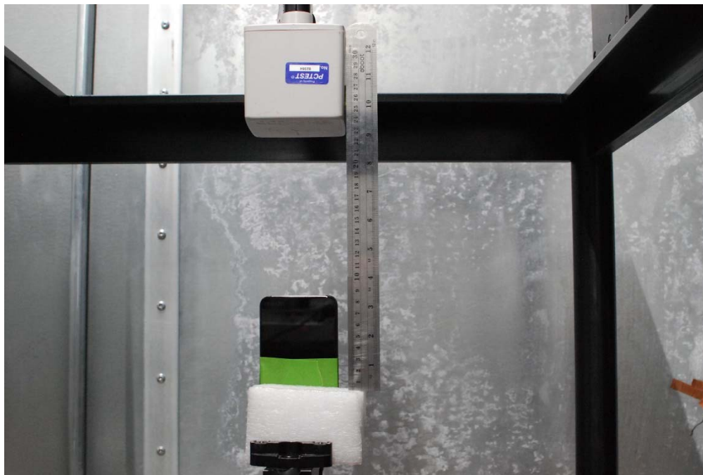
Test Setup Photo 22 H-field, Bottom edge, 15cm
