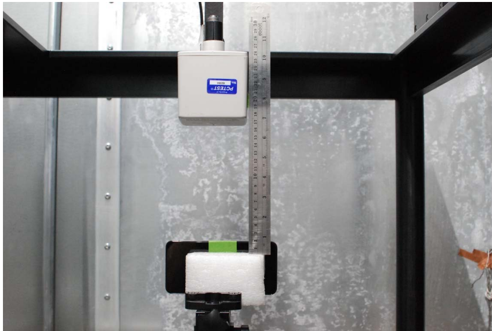
Test Setup Photo 24 H-field, Left edge, 15cm
