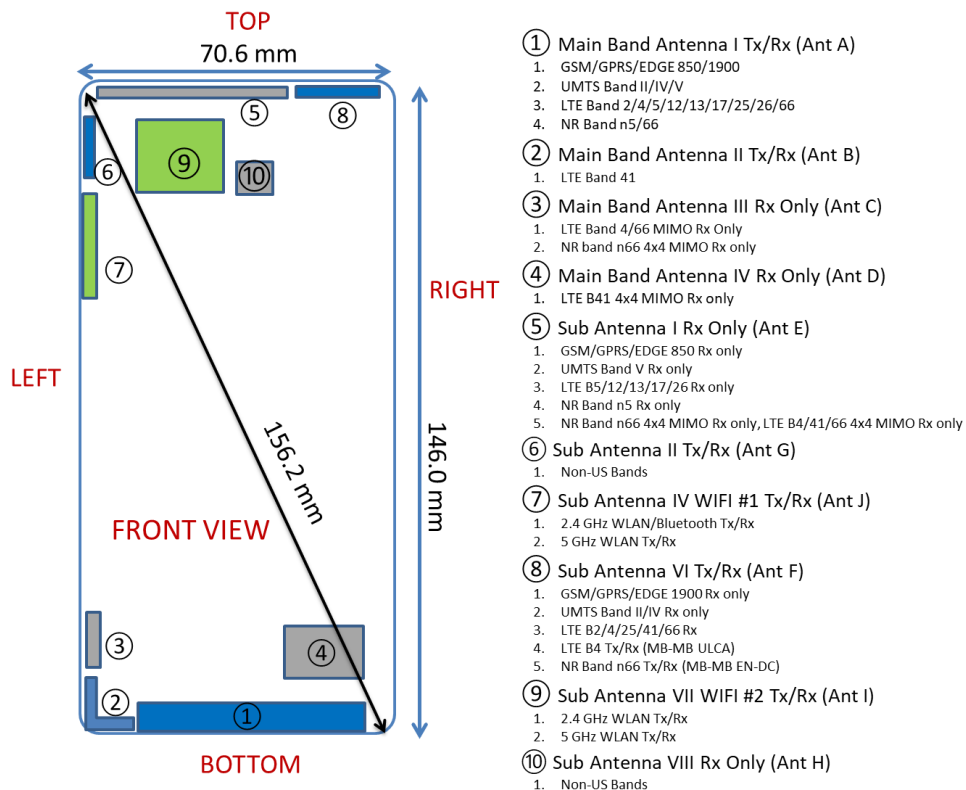
Figure E-1 DUT Antenna Locations
