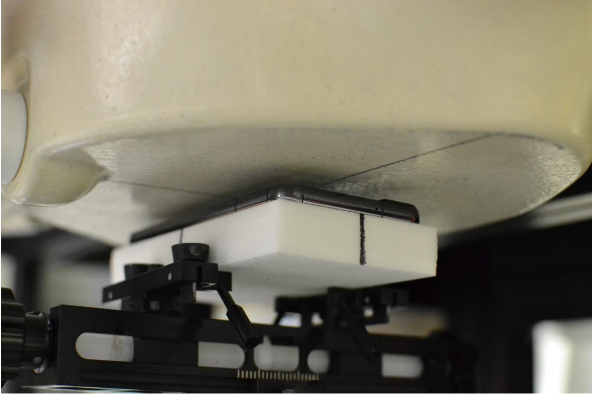
SAR Test Setup Photo 7 – Phablet, Back Side at 9 mm
