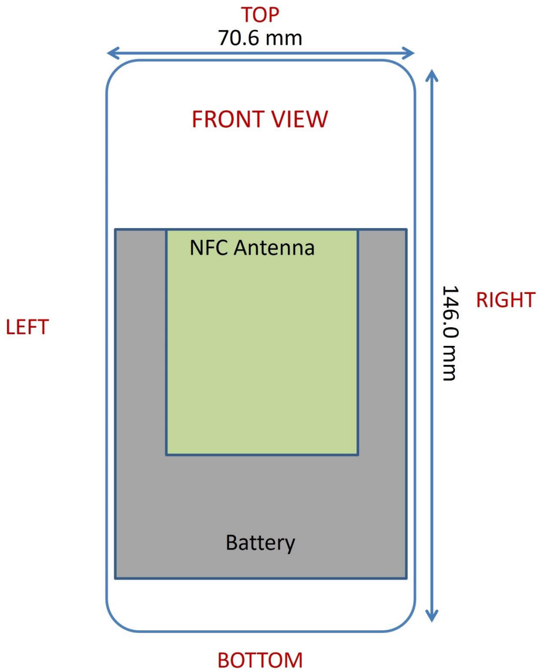
Figure I-2 NFC Antenna Locations
