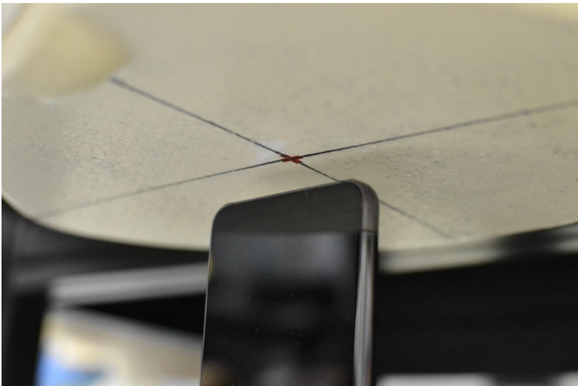
SAR Test Setup Photo 14 – Phablet, Bottom Edge at 13mm
