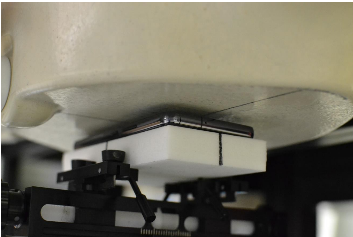
SAR Test Setup Photo 10 – Phablet, Front Side at 7mm
