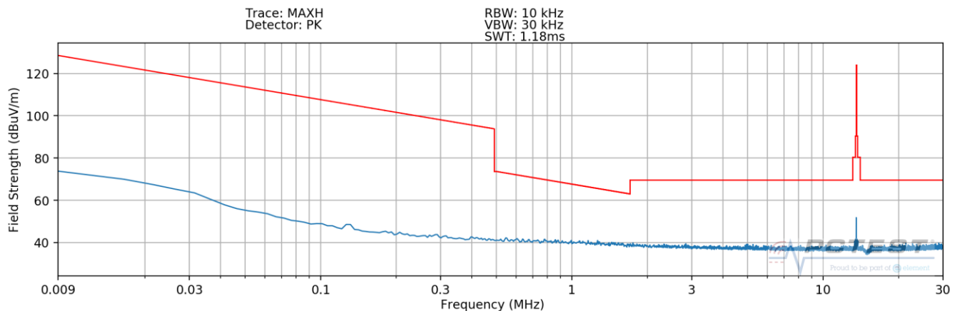
Plot 7-3. Radiated Spurious Plot 9kHz – 30MHz (Pol. Z)
