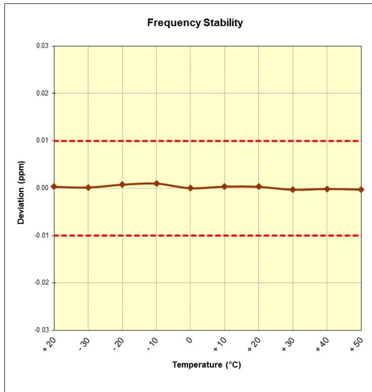
Figure 7-3. Frequency Stability Plot
