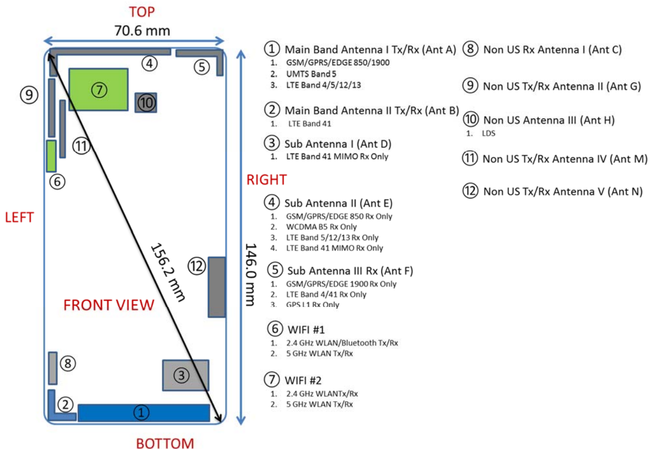
Figure E-1 DUT Antenna Locations
