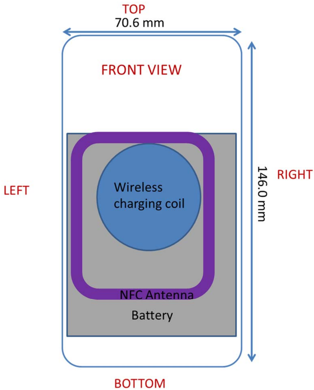
Figure E-2 NFC Antenna Locations
