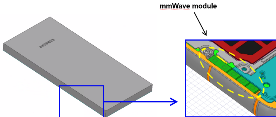
Figure 4. mmWave module (ANT M)
