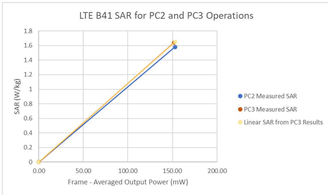
Figure 13-8 LTE Band 41 ULCA Phablet Linearity
