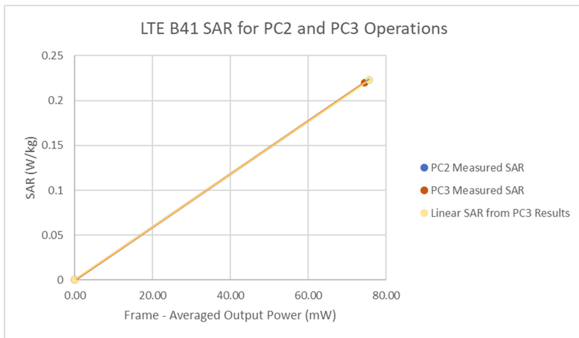
Figure 13-6 LTE Band 41 ULCA Hotspot Linearity
