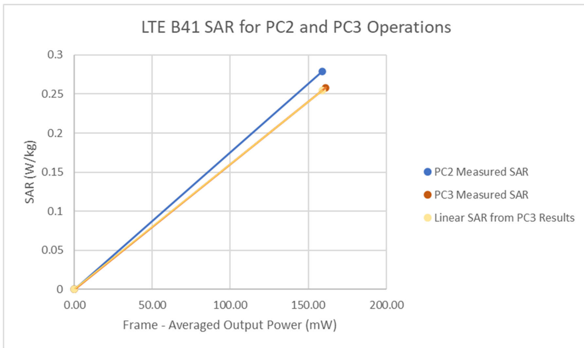
Figure 13-3 LTE Band 41 Body-Worn Linearity
