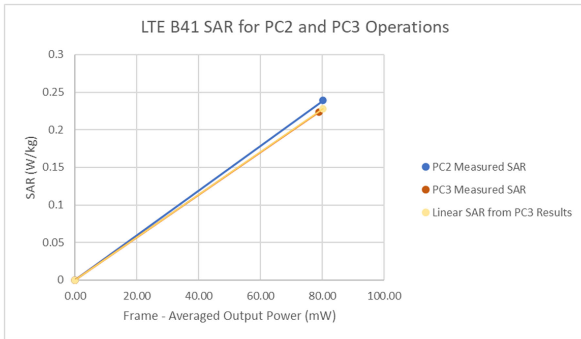
Figure 13-5 LTE Band 41 Hotspot Linearity
