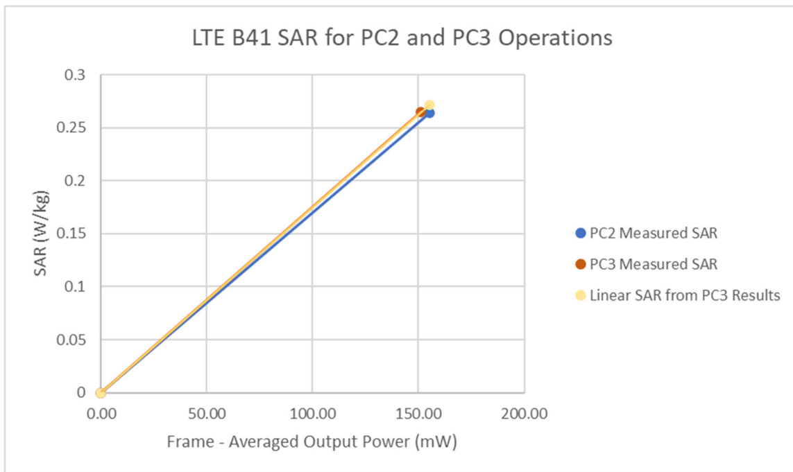
Figure 13-4 LTE Band 41 ULCA Body-Worn Linearity
