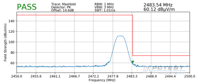
Plot 7-46. Radiated Restricted Upper Band Edge Measurement (Peak)
