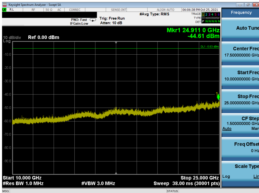
Plot 7-42. Conducted Spurious Plot (Bluetooth (LE), 1Mbps – Ch. 19)
