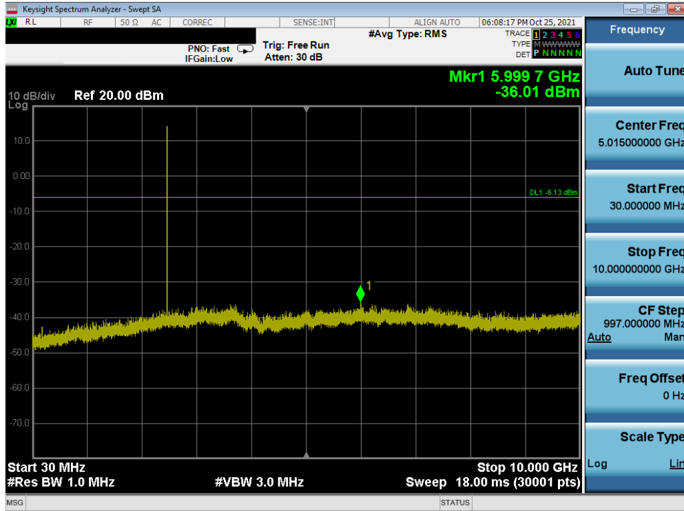
Plot 7-43. Conducted Spurious Plot (Bluetooth (LE), 1Mbps – Ch. 39)
