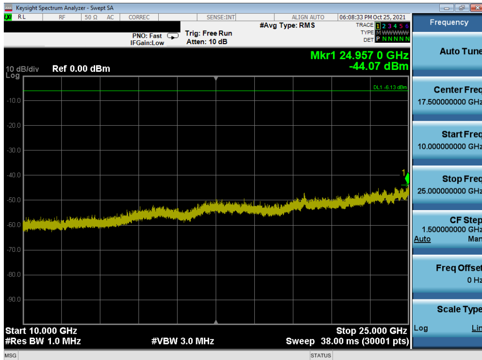
Plot 7-44. Conducted Spurious Plot (Bluetooth (LE), 1Mbps – Ch. 39)
