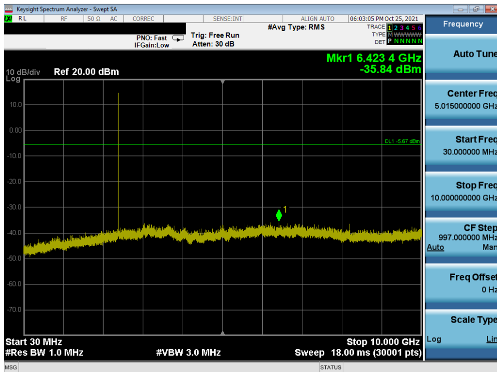
Plot 7-39. Conducted Spurious Plot (Bluetooth (LE), 1Mbps – Ch. 0)
