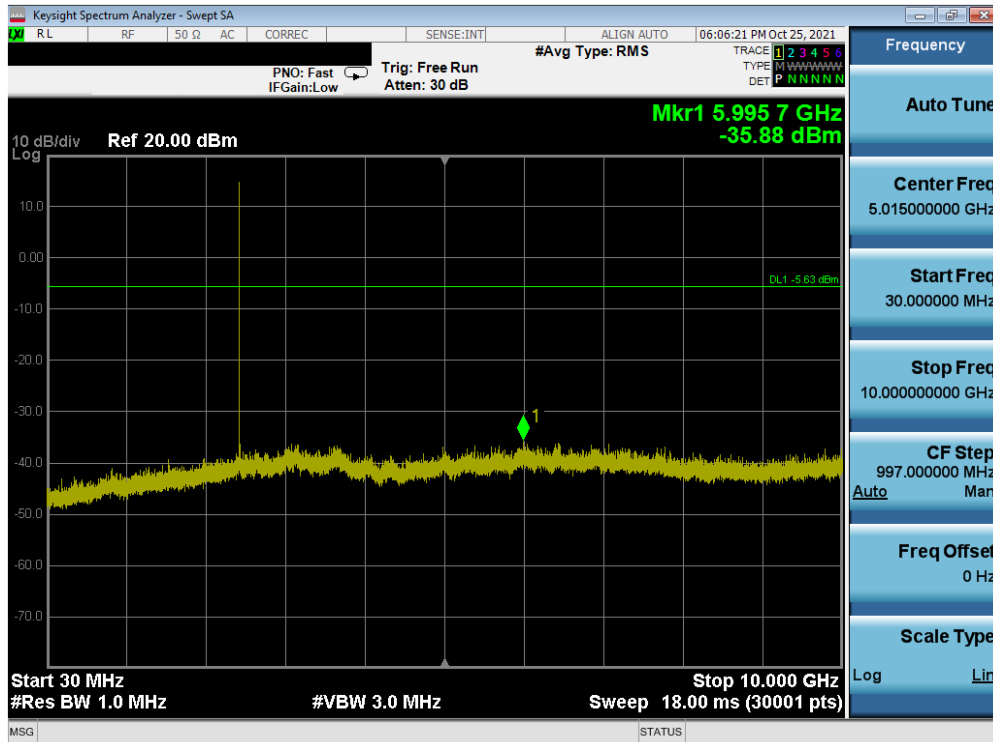
Plot 7-41. Conducted Spurious Plot (Bluetooth (LE), 1Mbps – Ch. 19)
