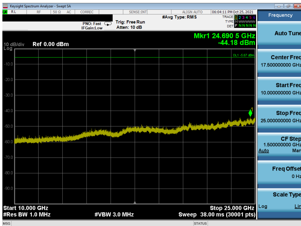
Plot 7-40. Conducted Spurious Plot (Bluetooth (LE), 1Mbps – Ch. 0)
