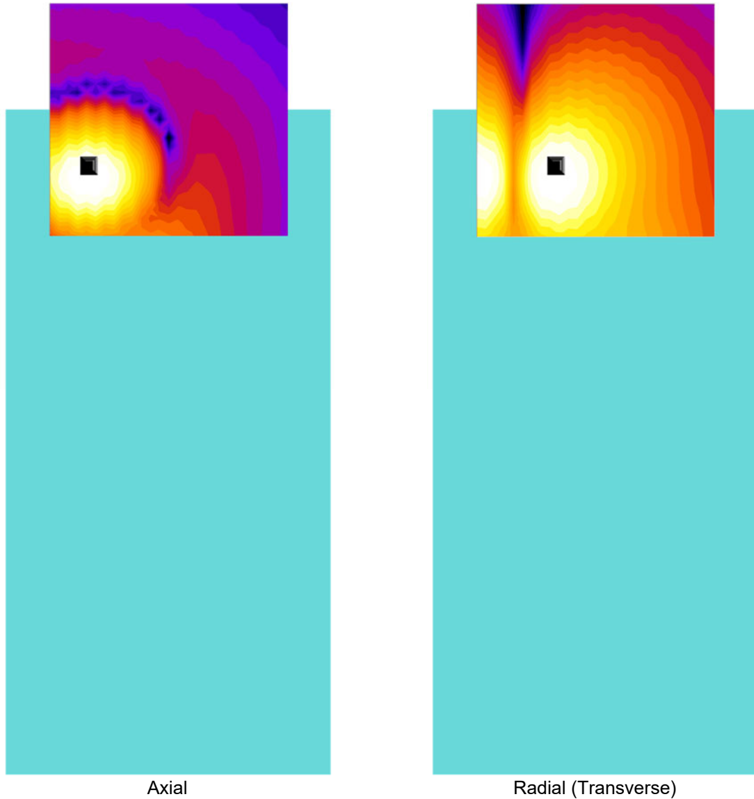
Figure 10-1 T-Coil Scan Overlay Magnetic Field Distributions
