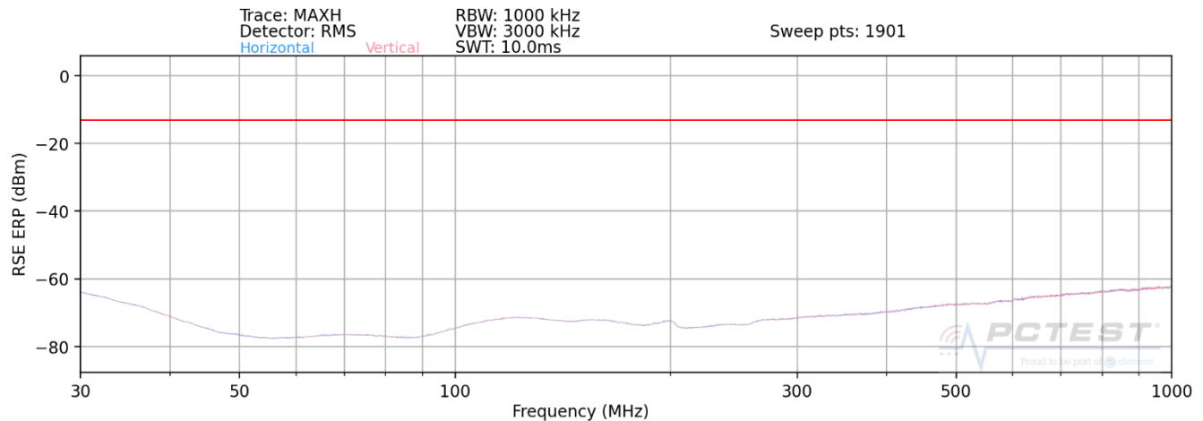
Plot 7-33. Ant 1- n258-R1 Radiated Spurious Plot (1CC QPSK Mid Channel 2Tx – EN-DC Anchor Band 2)
