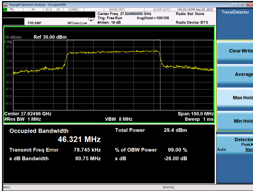
Plot 7-3. Ant 2 Occupied Bandwidth Plot (50MHz-1CC – QPSK – Mid Channel)
