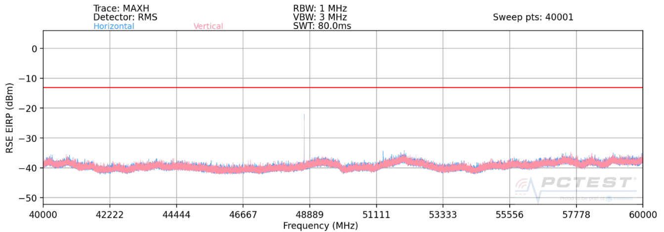
Plot 7-37. Ant 1-n258-R1 Radiated Spurious Plot (1CC QPSK Mid Channel 2Tx – EN-DC Anchor B2)
