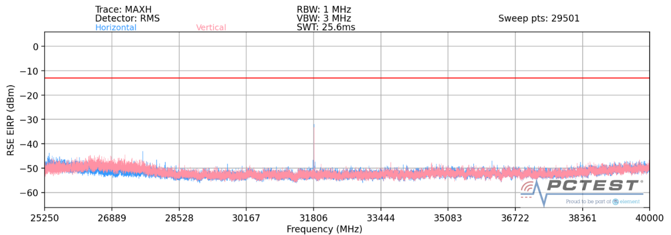
Plot 7-36. Ant 1-n258-R1 Radiated Spurious Plot (1CC QPSK Mid Channel 2Tx – EN-DC Anchor B2)
