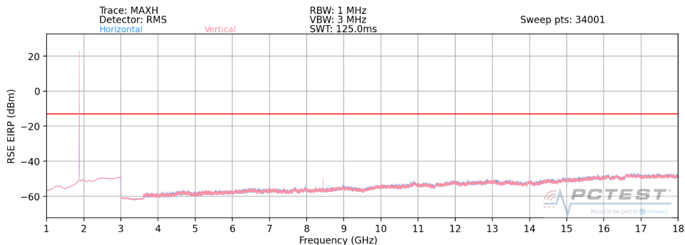
Plot 7-34. Ant 1-n258-R1 Radiated Spurious Plot (1CC QPSK Mid Channel 2Tx – EN-DC Anchor Band 2)
