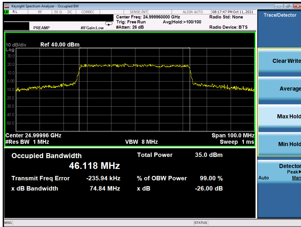
Plot 7-2. Ant 2 Occupied Bandwidth Plot (50MHz-1CC – QPSK – Mid Channel)
