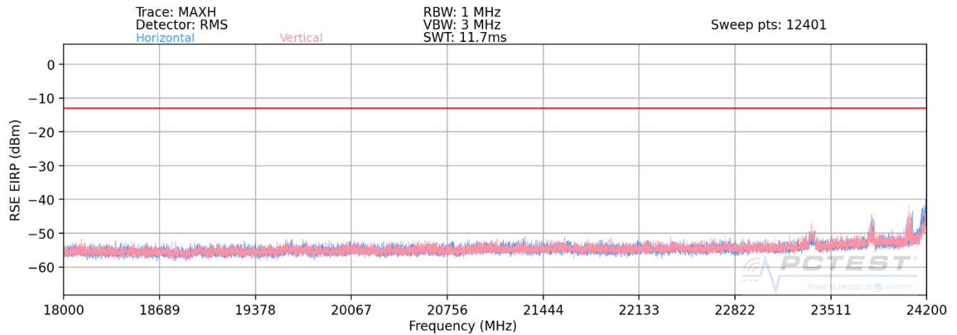
Plot 7-35. Ant 1-n258-R1 Radiated Spurious Plot (1CC QPSK Mid Channel 2Tx – EN-DC Anchor B2)
