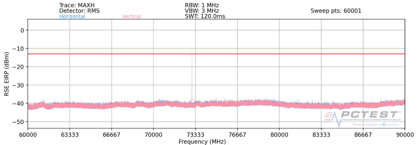
Plot 7-38. Ant 1-n258-R1 Radiated Spurious Plot (1CC QPSK Mid Channel 2Tx – EN-DC Anchor B2)
