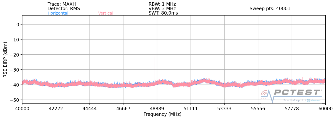
Plot 7-37. Ant 2-n258-R1 Radiated Spurious Plot (1CC QPSK Mid Channel 2Tx – EN-DC Anchor B2)
