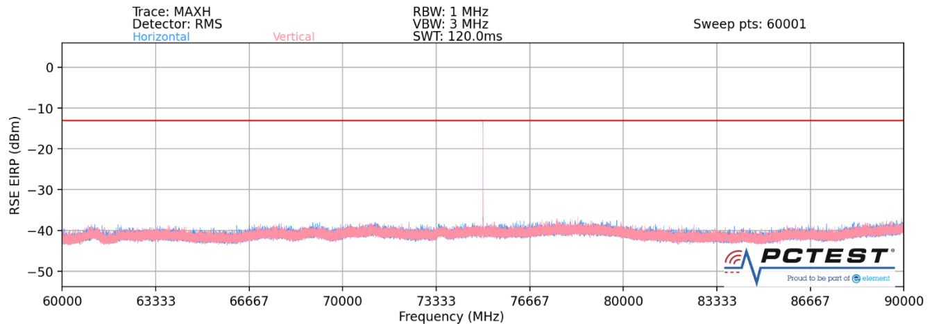
Plot 7-38. Ant 1-n258-R2 Radiated Spurious Plot (1CC QPSK Mid Channel 2Tx – EN-DC Anchor B2)
