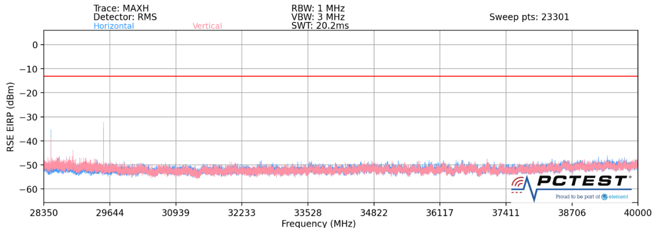
Plot 7-43. Ant 1-n261 Radiated Spurious Plot (1CC QPSK Mid Channel 2Tx – EN-DC Anchor B2)
