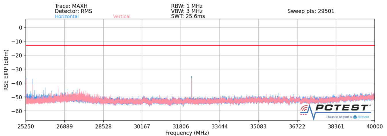
Plot 7-36. Ant 1-n258-R2 Radiated Spurious Plot (1CC QPSK Mid Channel 2Tx – EN-DC Anchor B2)
