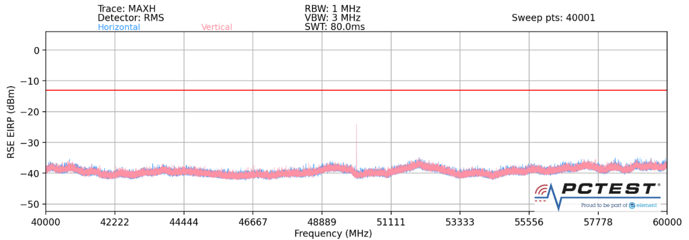
Plot 7-37. Ant 1-n258-R2 Radiated Spurious Plot (1CC QPSK Mid Channel 2Tx – EN-DC Anchor B2)
