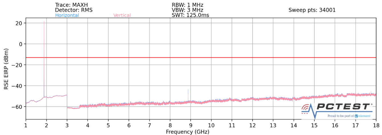
Plot 7-34. Ant 2-n258-R2 Radiated Spurious Plot (1CC QPSK Mid Channel 2Tx – EN-DC Anchor Band 2)
