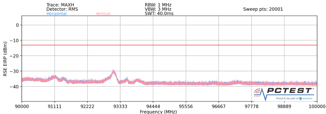
Plot 7-39. Ant 2-n258-R2 Radiated Spurious Plot (1CC QPSK Mid Channel 2Tx – EN-DC Anchor B2)
