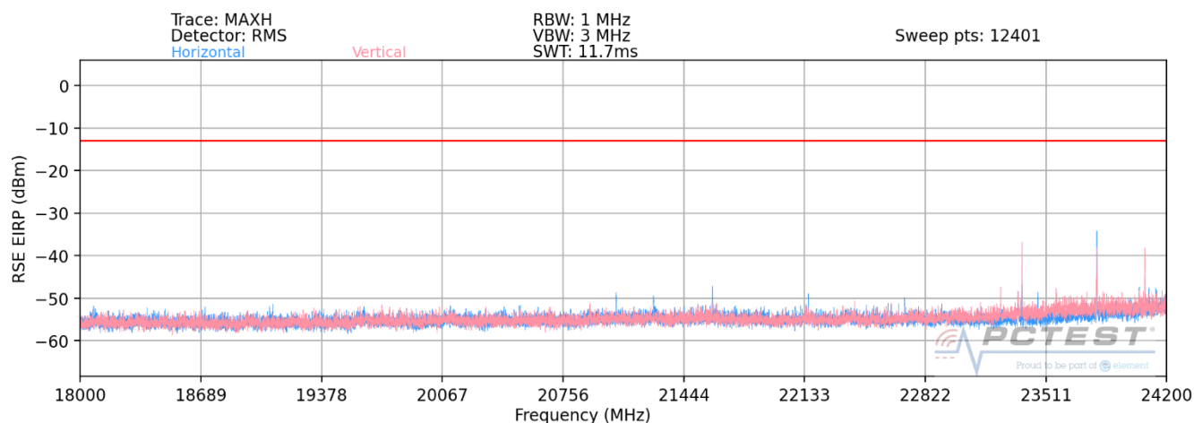
Plot 7-35. Ant 2-n258-R1 Radiated Spurious Plot (1CC QPSK Mid Channel 2Tx – EN-DC Anchor B2)
