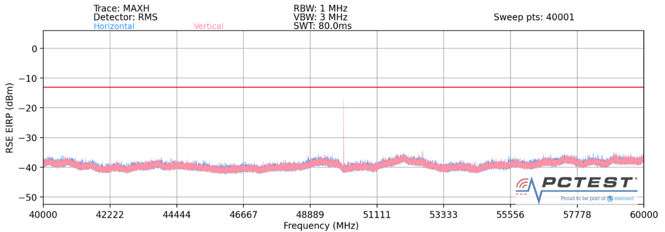
Plot 7-37. Ant 2-n258-R2 Radiated Spurious Plot (1CC QPSK Mid Channel 2Tx – EN-DC Anchor B2)
