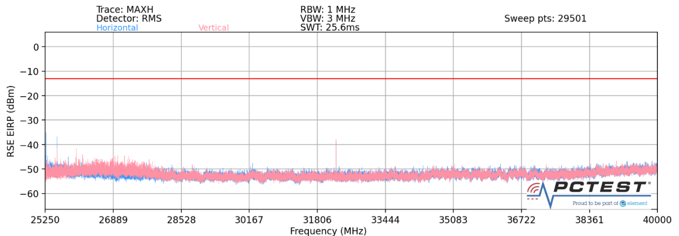
Plot 7-36. Ant 2-n258-R2 Radiated Spurious Plot (1CC QPSK Mid Channel 2Tx – EN-DC Anchor B2)
