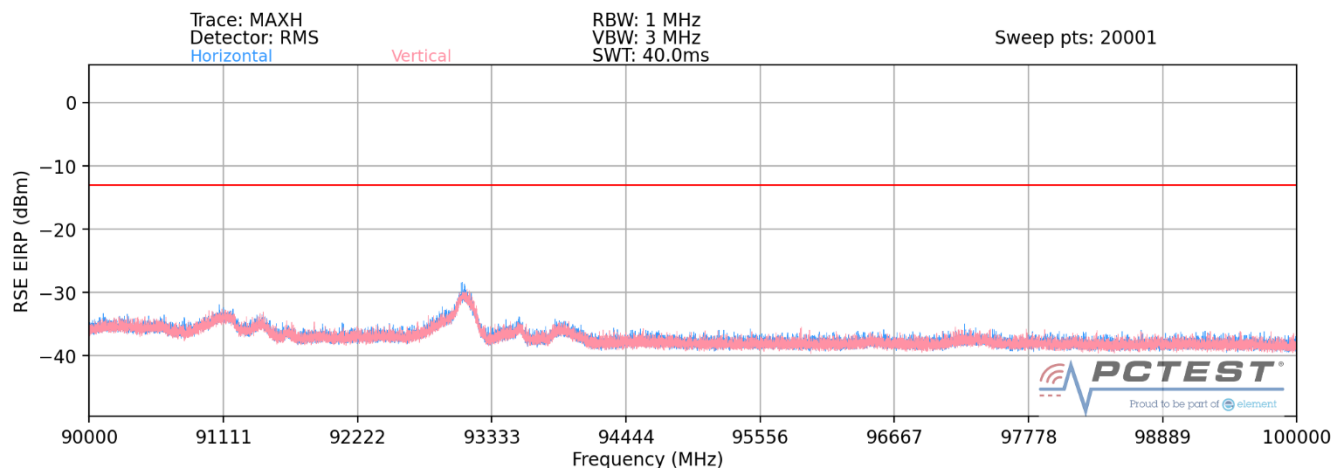
Plot 7-39. Ant 2-n258-R1 Radiated Spurious Plot (1CC QPSK Mid Channel 2Tx – EN-DC Anchor B2)
