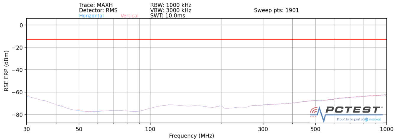
Plot 7-33. Ant 2- n258-R2 Radiated Spurious Plot (1CC QPSK Mid Channel 2Tx – EN-DC Anchor Band 2)
