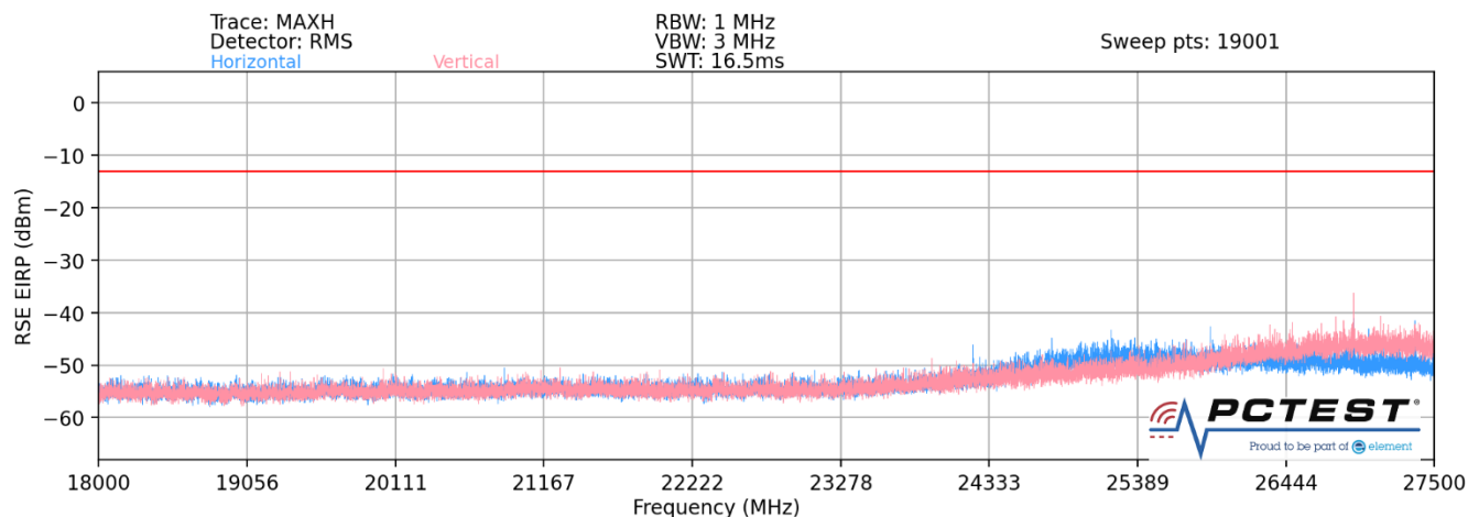
Plot 7-42. Ant 1-n261 Radiated Spurious Plot (1CC QPSK Mid Channel 2Tx – EN-DC Anchor B2)
