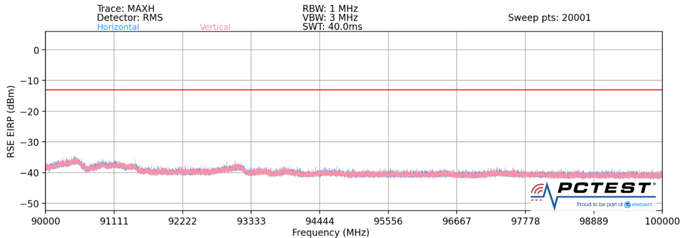
Plot 7-46. Ant 1-n261 Radiated Spurious Plot (1CC QPSK Mid Channel 2Tx – EN-DC Anchor B2)
