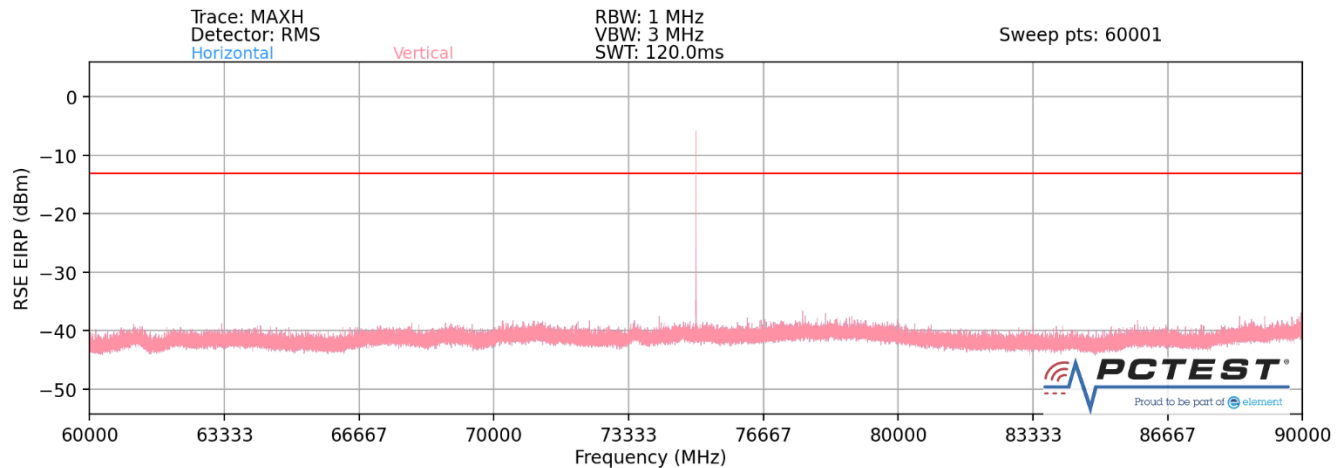
Plot 7-38. Ant 2-n258-R2 Radiated Spurious Plot (1CC QPSK Mid Channel 2Tx – EN-DC Anchor B2)
