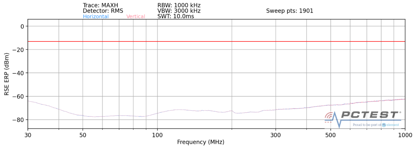
Plot 7-33. Ant 1- n258-R2 Radiated Spurious Plot (1CC QPSK Mid Channel 2Tx – EN-DC Anchor Band 2)
