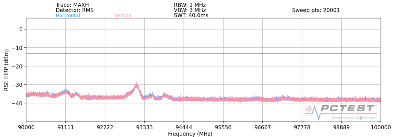
Plot 7-39. Ant 1-n258-R1 Radiated Spurious Plot (1CC QPSK Mid Channel 2Tx – EN-DC Anchor B2)
