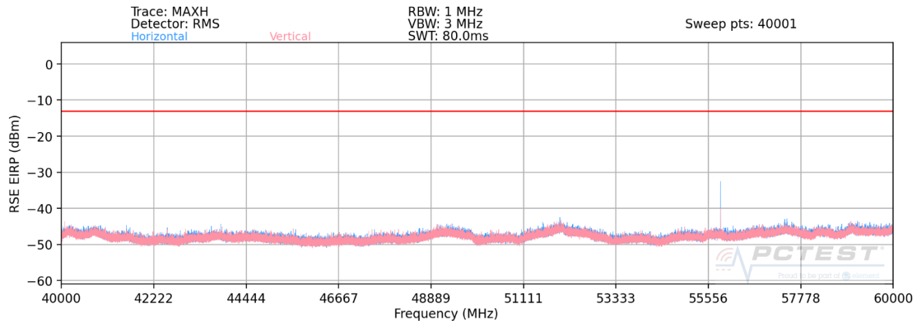
Plot 7-44. Ant 1-n261 Radiated Spurious Plot (1CC QPSK Mid Channel 2Tx – EN-DC Anchor B2)
