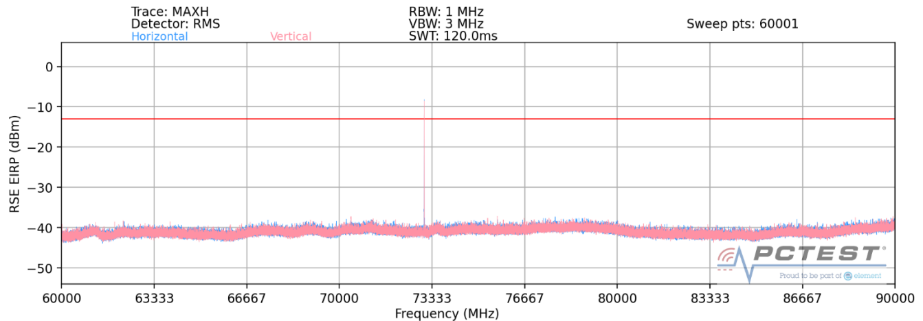
Plot 7-38. Ant 2-n258-R1 Radiated Spurious Plot (1CC QPSK Mid Channel 2Tx – EN-DC Anchor B2)
