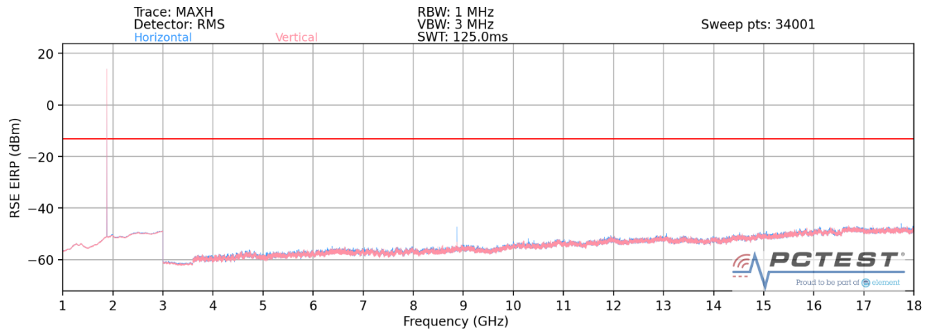
Plot 7-34. Ant 1-n258-R2 Radiated Spurious Plot (1CC QPSK Mid Channel 2Tx – EN-DC Anchor Band 2)
