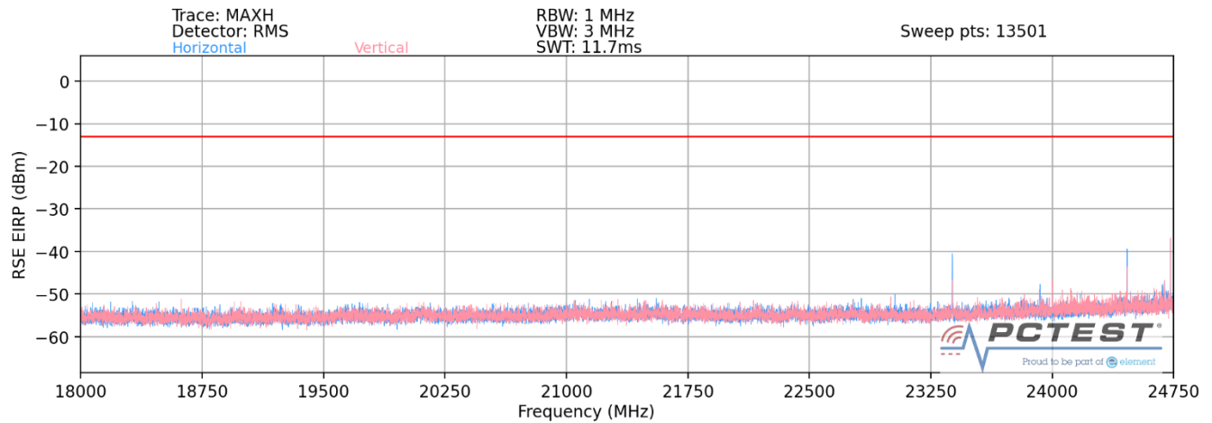
Plot 7-35. Ant 2-n258-R2 Radiated Spurious Plot (1CC QPSK Mid Channel 2Tx – EN-DC Anchor B2)
