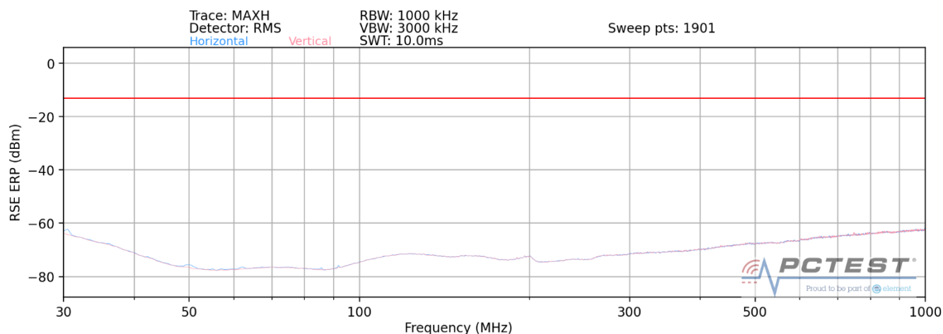
Plot 7-33. Ant 2- n258-R1 Radiated Spurious Plot (1CC QPSK Mid Channel 2Tx – EN-DC Anchor Band 2)
