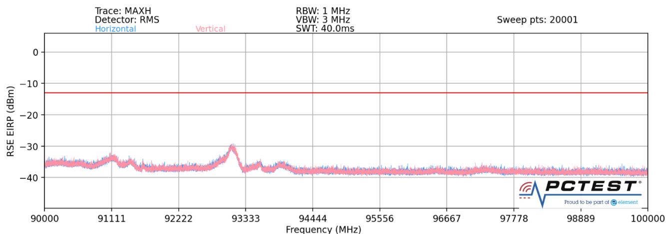
Plot 7-39. Ant 1-n258-R2 Radiated Spurious Plot (1CC QPSK Mid Channel 2Tx – EN-DC Anchor B2)
