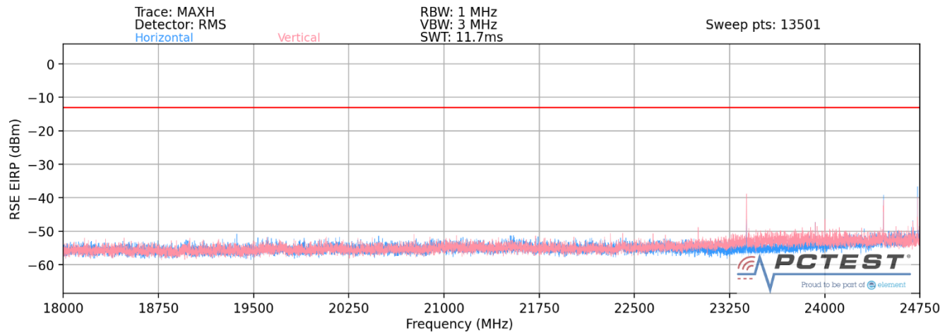
Plot 7-35. Ant 1-n258-R2 Radiated Spurious Plot (1CC QPSK Mid Channel 2Tx – EN-DC Anchor B2)
