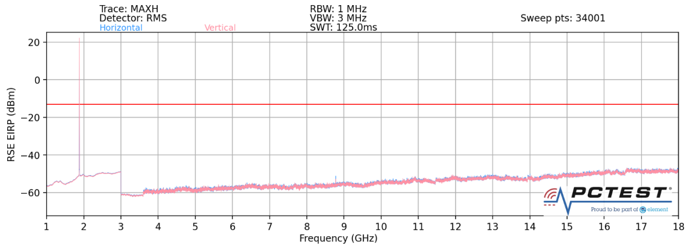
Plot 7-41. Ant 1-n261 Radiated Spurious Plot (1CC QPSK Mid Channel 2Tx – EN-DC Anchor Band 2)
