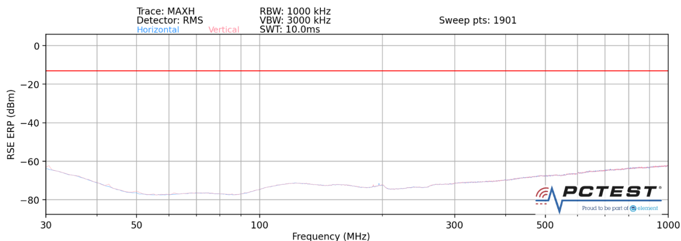
Plot 7-40. Ant 1-n261 Radiated Spurious Plot (1CC QPSK Mid Channel 2Tx – EN-DC Anchor Band 2)
