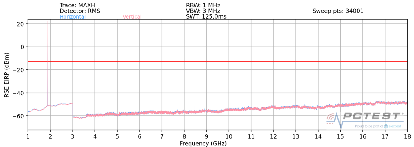
Plot 7-34. Ant 2-n258-R1 Radiated Spurious Plot (1CC QPSK Mid Channel 2Tx – EN-DC Anchor Band 2)
