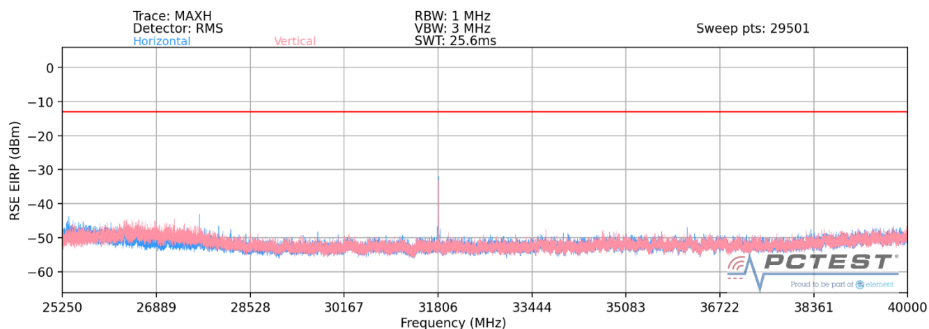
Plot 7-36. Ant 2-n258-R1 Radiated Spurious Plot (1CC QPSK Mid Channel 2Tx – EN-DC Anchor B2)
