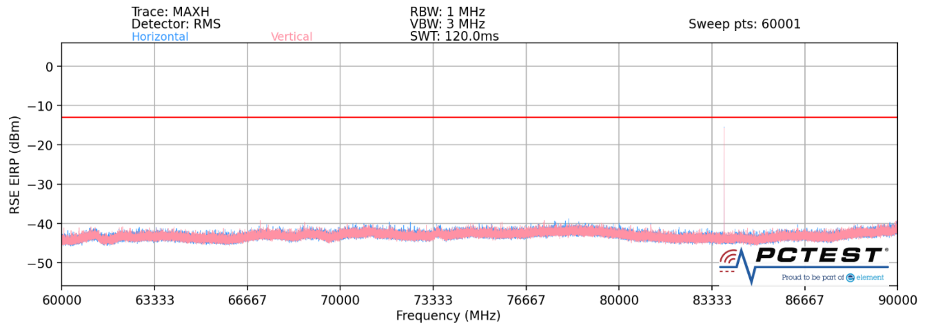
Plot 7-45. Ant 1-n261 Radiated Spurious Plot (1CC QPSK Mid Channel 2Tx – EN-DC Anchor B2)
