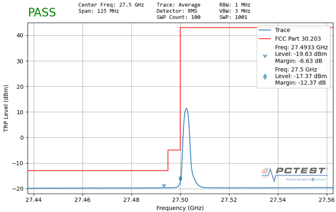
Plot 7-79. Ant 2 Lower Band Edge- TRP (50MHz-1CC – QPSK 1 RB)
