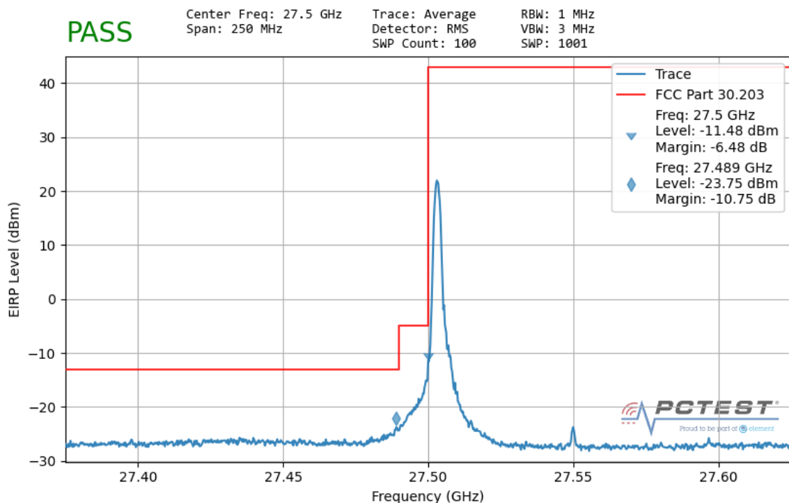
Plot 7-91. Ant 1 Lower Band Edge (100MHz-1CC – QPSK 1 RB)
