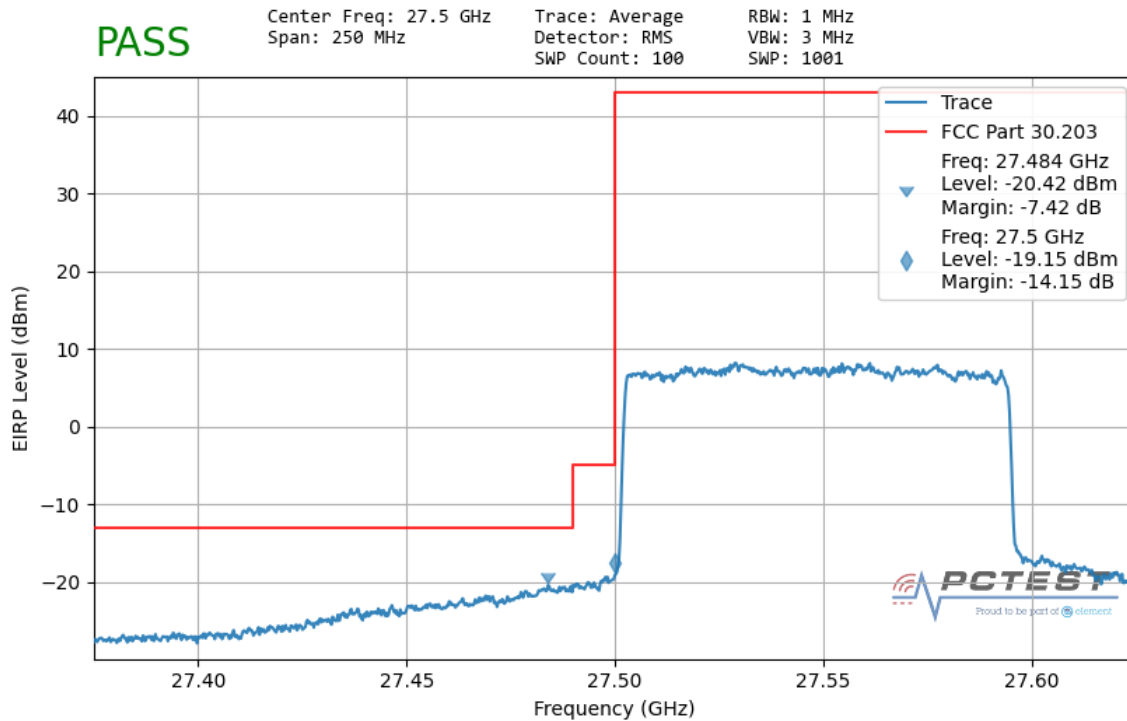
Plot 7-83. Ant 2 Lower Band Edge (100MHz-1CC – pi/2-BPSK Full RB)
