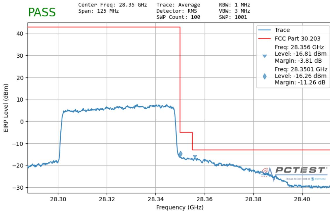
Plot 7-81. Ant 2 Upper Band Edge (50MHz-1CC – QPSK Full RB)
