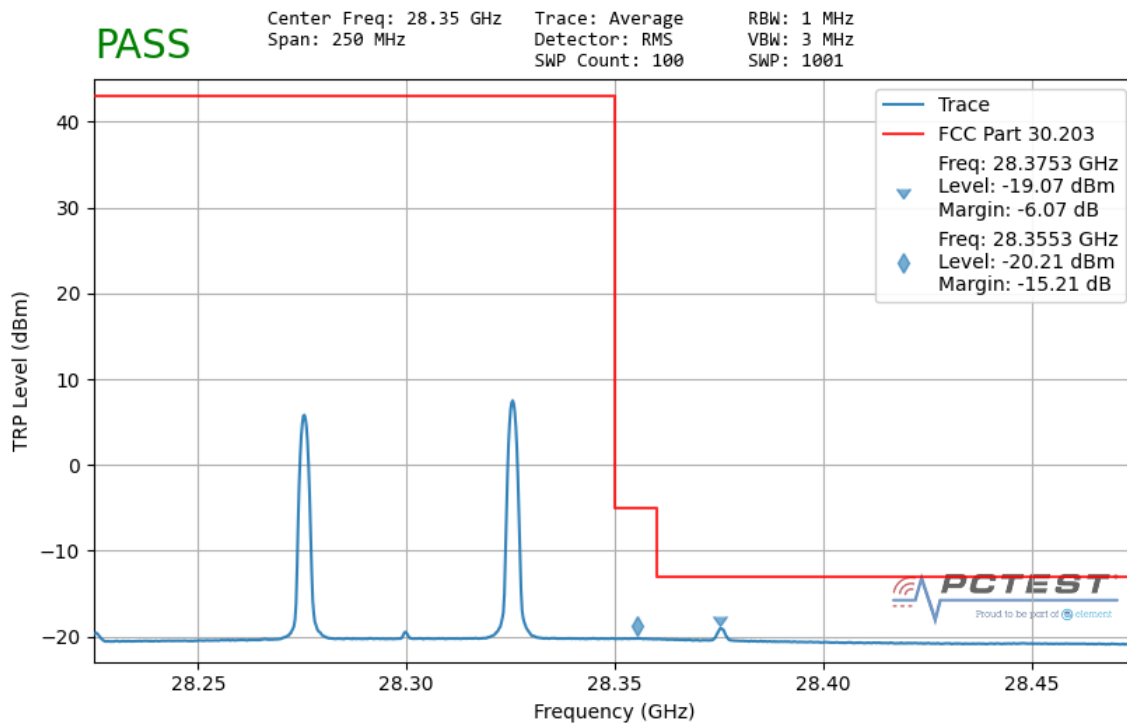
Plot 7-82. Ant 2 Upper Band Edge- TRP (50MHz-2CC – QPSK 1 RB)
