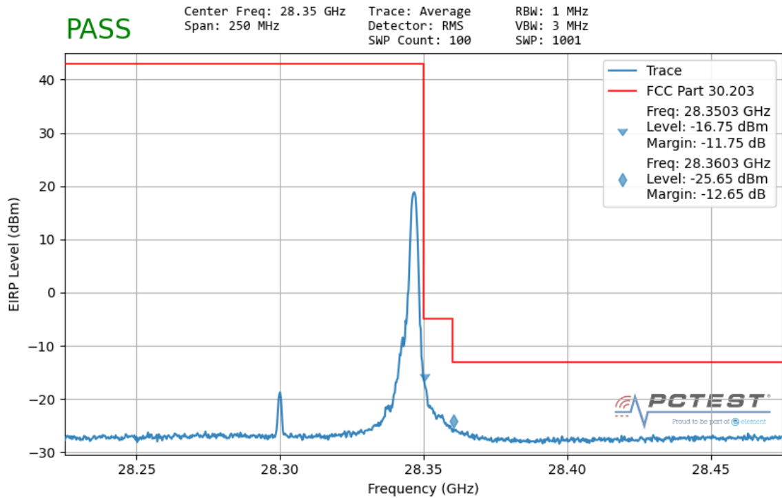
Plot 7-93. Ant 1 Upper Band Edge (100MHz-1CC – QPSK 1 RB)
