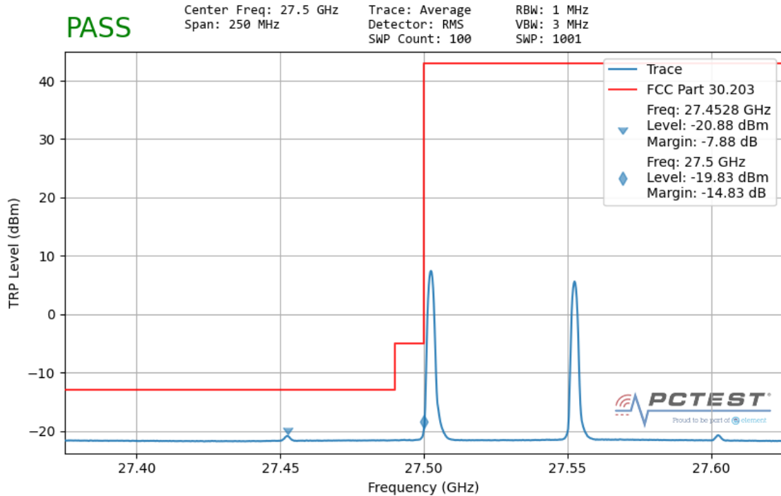
Plot 7-80. Ant 2 Lower Band Edge – TRP (50MHz-2CC – QPSK 1 RB)
