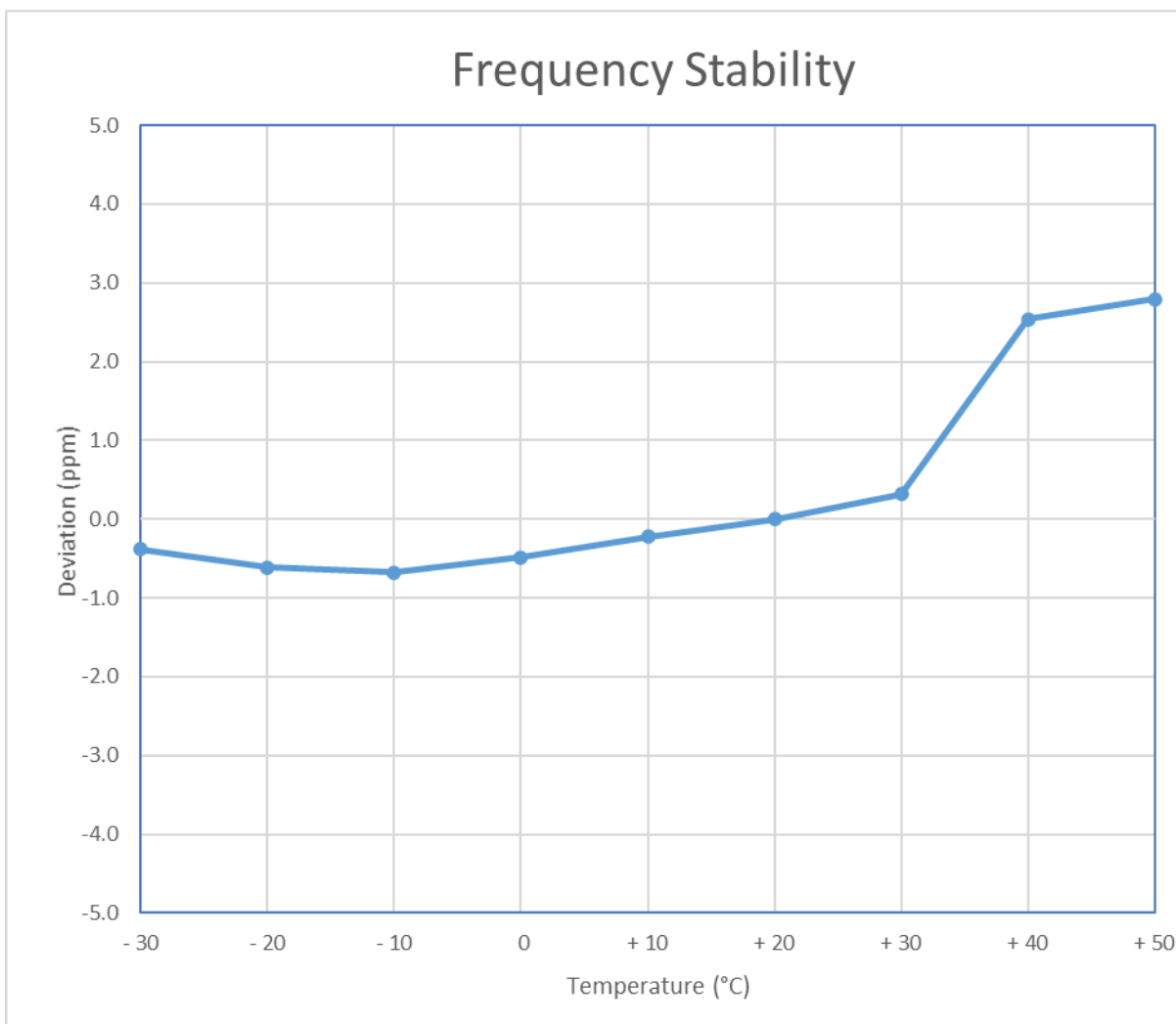
Figure 7-1. Frequency Stability Graph (n258-R2)
