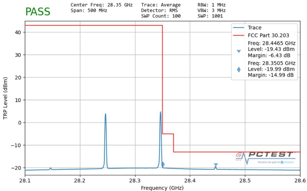
Plot 7-86. Ant 2 Upper Band Edge – TRP (100MHz-2CC – QPSK 1 RB)
