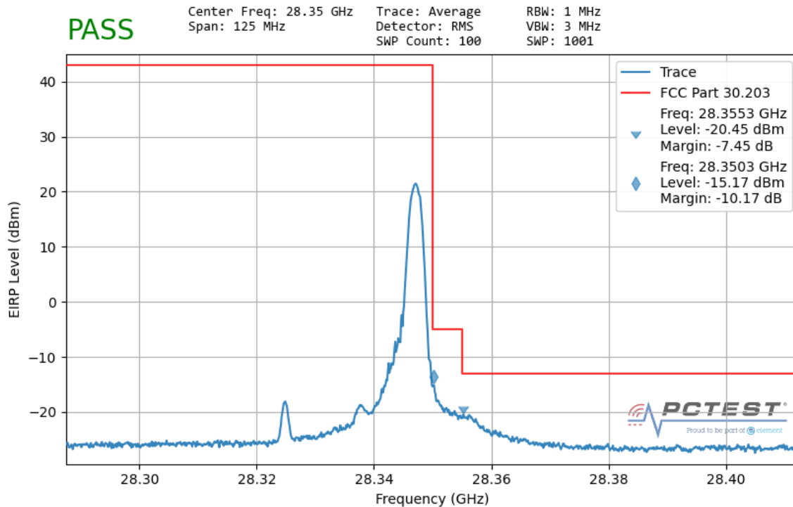
Plot 7-89. Ant 1 Upper Band Edge (50MHz-1CC – QPSK 1 RB)
