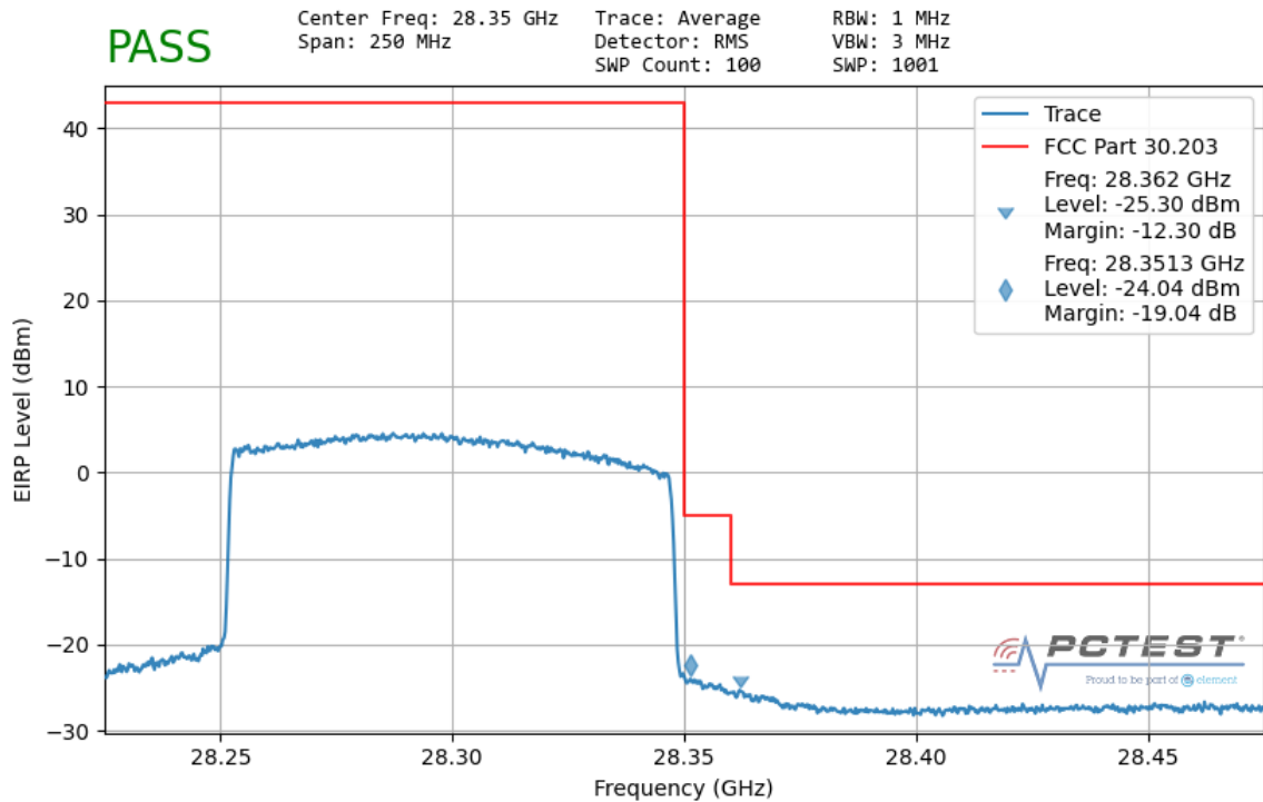
Plot 7-85. Ant 2 Upper Band Edge (100MHz-1CC – QPSK Full RB)
