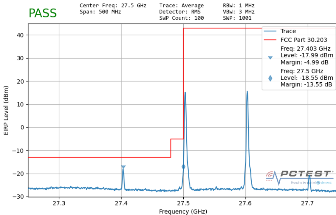
Plot 7-84. Ant 2 Lower Band Edge (100MHz-2CC – QPSK 1 RB)
