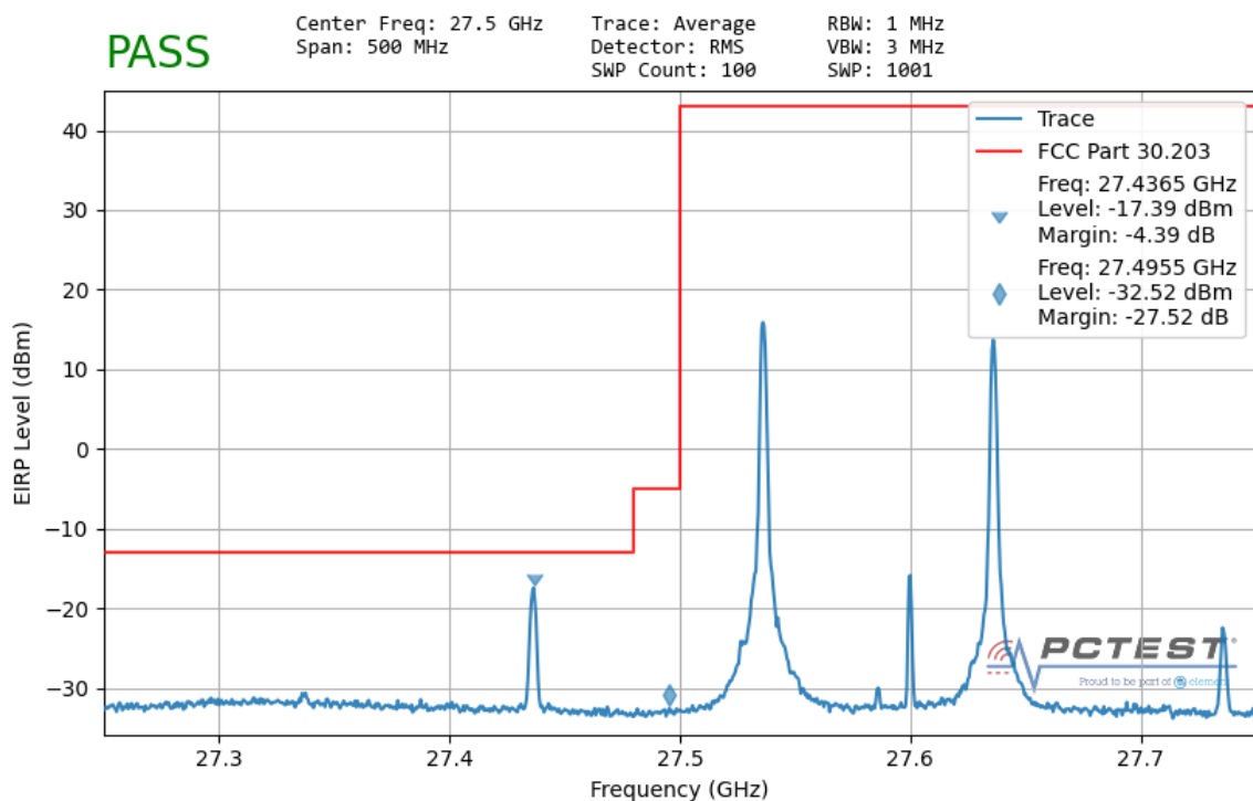
Plot 7-92. Ant 1 Lower Band Edge – TRP (100MHz-2CC – QPSK 1 RB)
