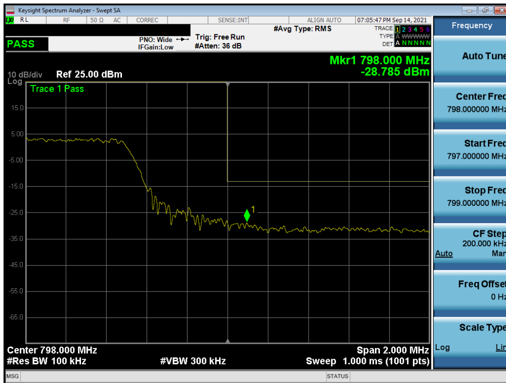
Plot 7-23. Upper Band Edge Plot (LTE Band 14, 10MHz QPSK - RB Size 50)
