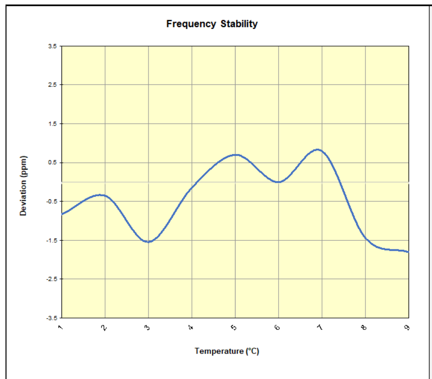
Plot 7-39. LTE Band 14 Frequency Stability Chart
