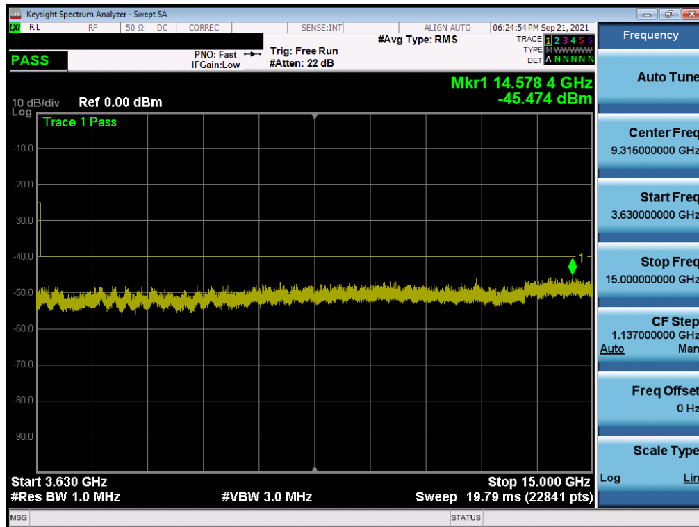
Plot 7-30. Conducted Spurious Plot (ULCA LB48 - 20+20MHz QPSK - Low Channel)
