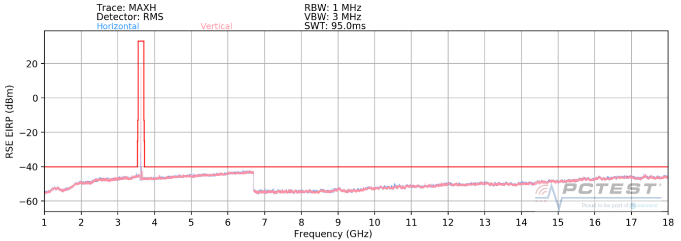
Plot 7-56. Radiated Spurious Plot (LTE Band 48, 1 – 18GHz)
