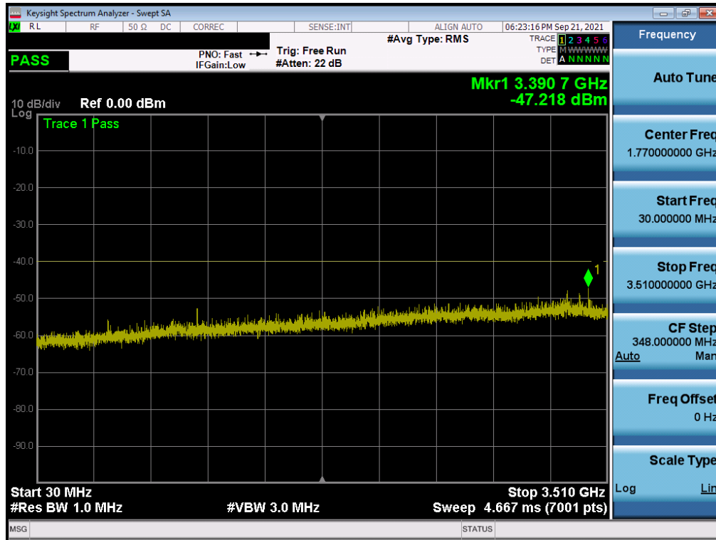
Plot 7-29. Conducted Spurious Plot (ULCA LB48 - 20+20MHz QPSK - Low Channel)
