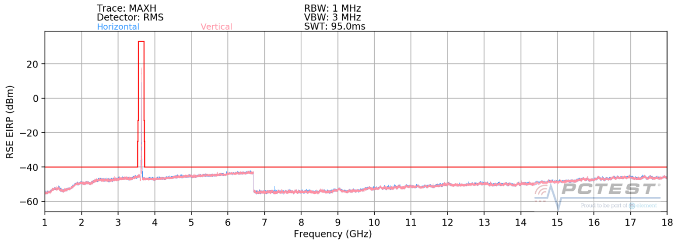
Plot 7-60. Radiated Spurious Plot (ULCA LB48– Mid Channel )
