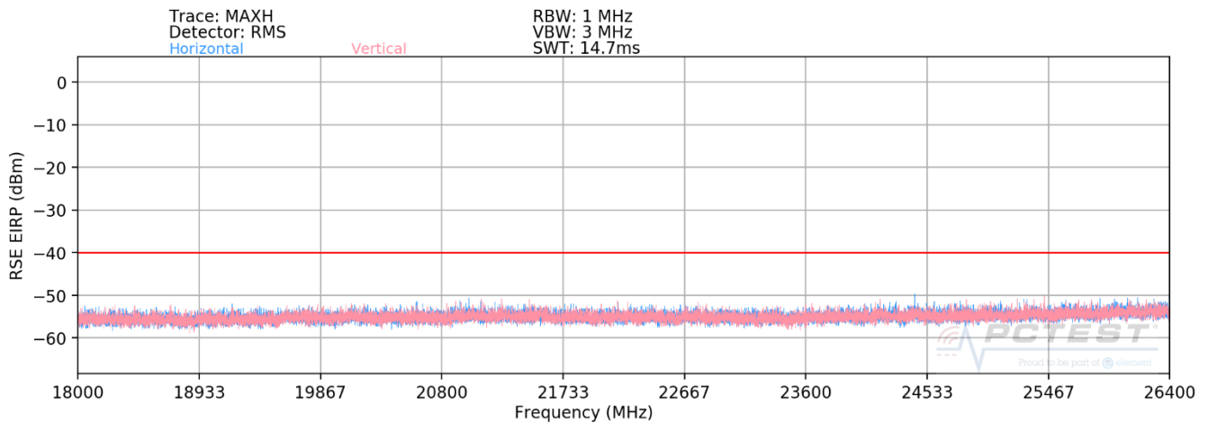
Plot 7-57. Radiated Spurious Plot (LTE Band 48, 18 – 26.5GHz)
