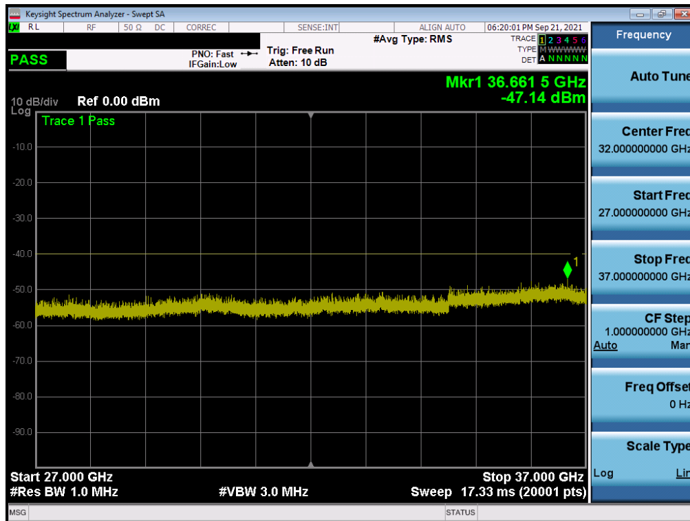
Plot 7-36. Conducted Spurious Plot (ULCA LB48 - 20+20MHz QPSK - Mid Channel)
