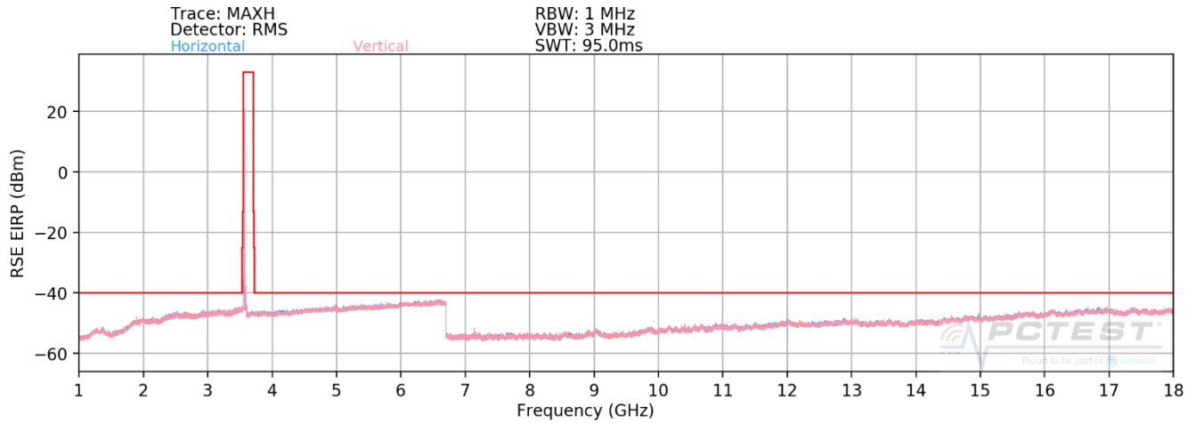
Plot 7-59. Radiated Spurious Plot (ULCA LB48 – Low Channel)
