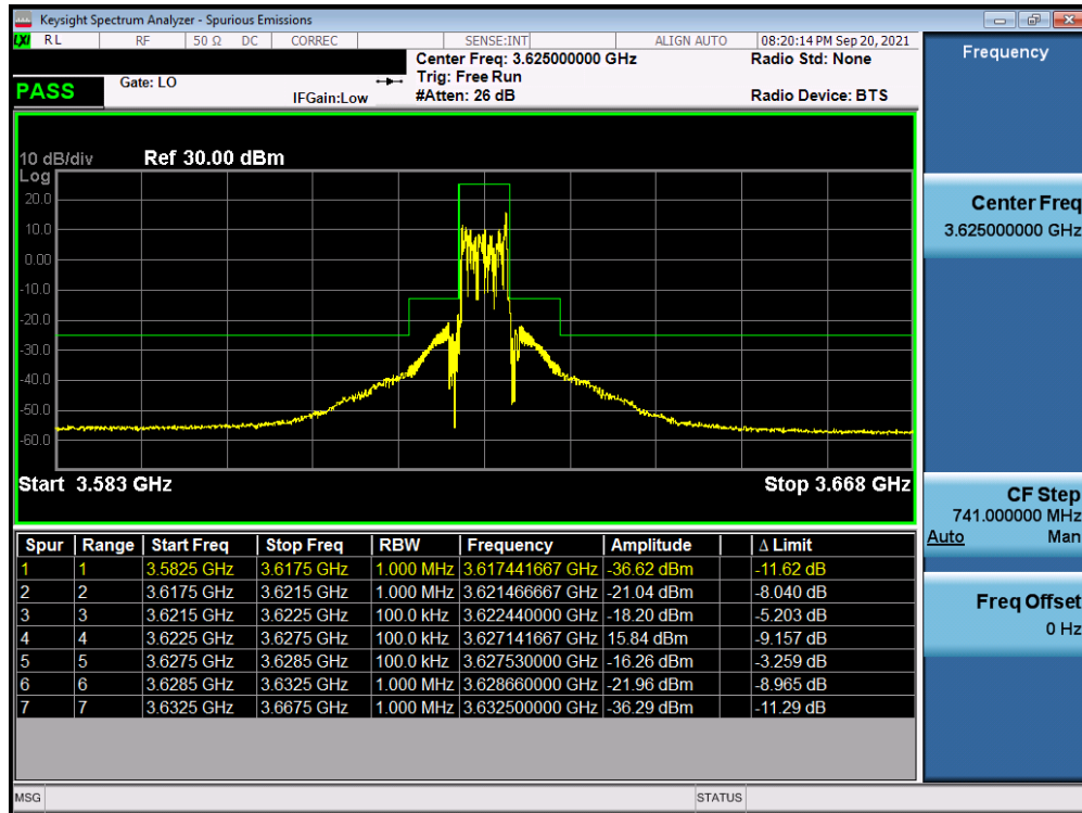
Plot 7-51. Channel Edge Plot (LTE Band 48 - 5MHz QPSK - Mid Channel)
