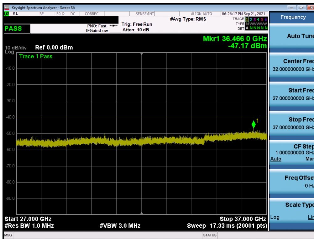
Plot 7-32. Conducted Spurious Plot (ULCA LB48 - 20+20MHz QPSK - Low Channel)
