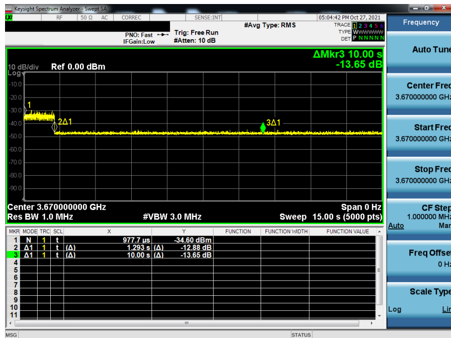
Plot 7-66. Run#2 End User Device Discontinues Operations within 10s
