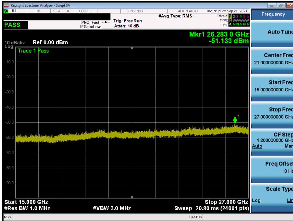
Plot 7-35. Conducted Spurious Plot (ULCA LB48 - 20+20MHz QPSK - Mid Channel)
