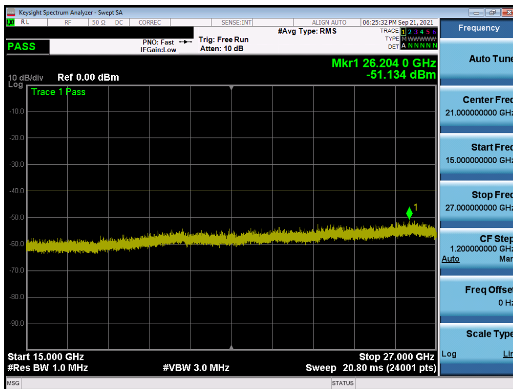
Plot 7-31. Conducted Spurious Plot (ULCA LB48 - 20+20MHz QPSK - Low Channel)
