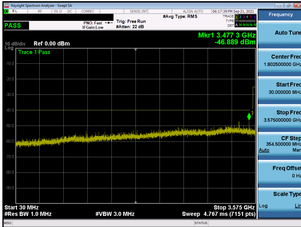
Plot 7-33. Conducted Spurious Plot (ULCA LB48 - 20+20MHz QPSK - Mid Channel)
