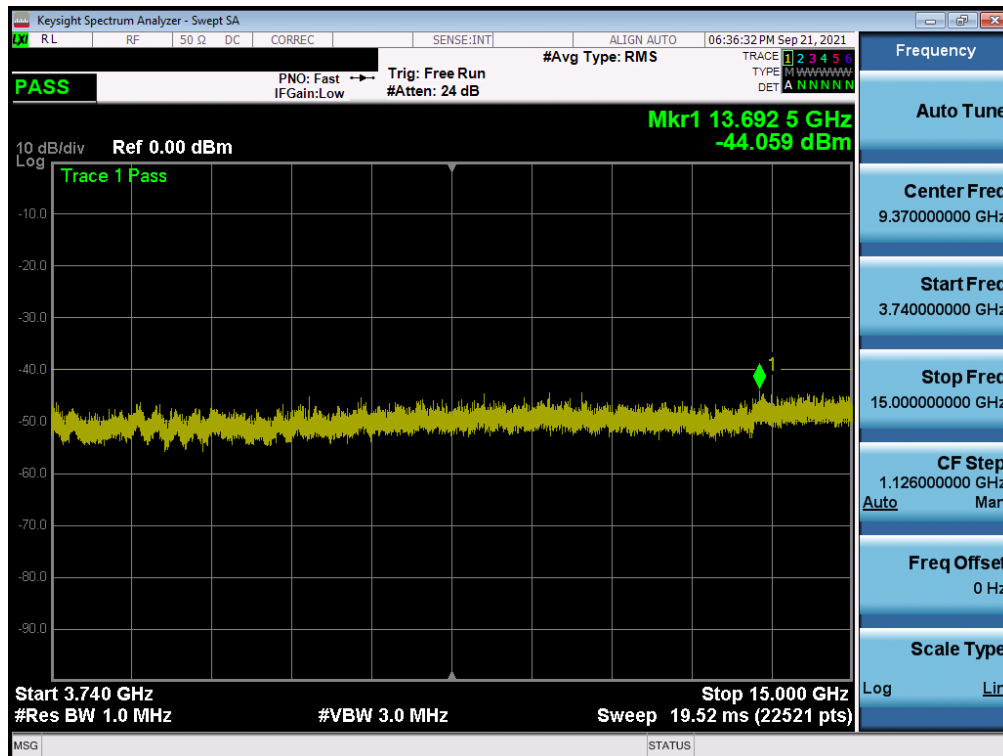
Plot 7-38. Conducted Spurious Plot (ULCA LB48 - 20+20MHz QPSK - High Channel)
