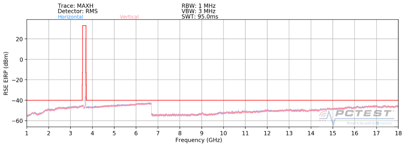
Plot 7-61. Radiated Spurious Plot (ULCA LB48 – High Channel)
