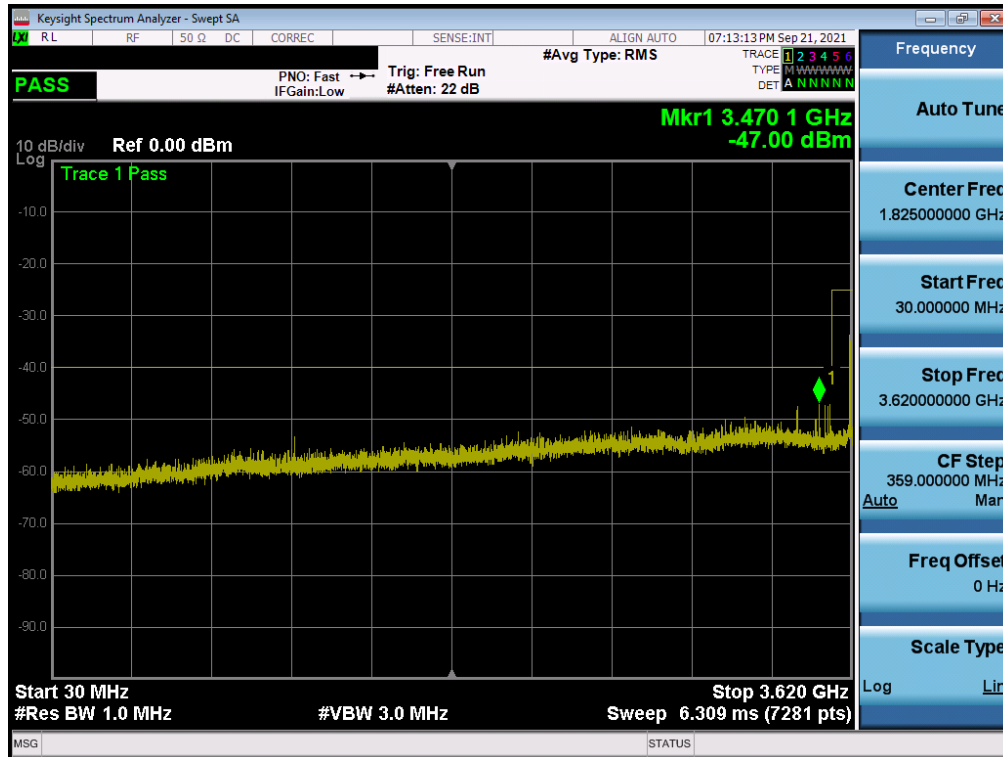
Plot 7-37. Conducted Spurious Plot (ULCA LB48 - 20+20MHz QPSK - High Channel)
