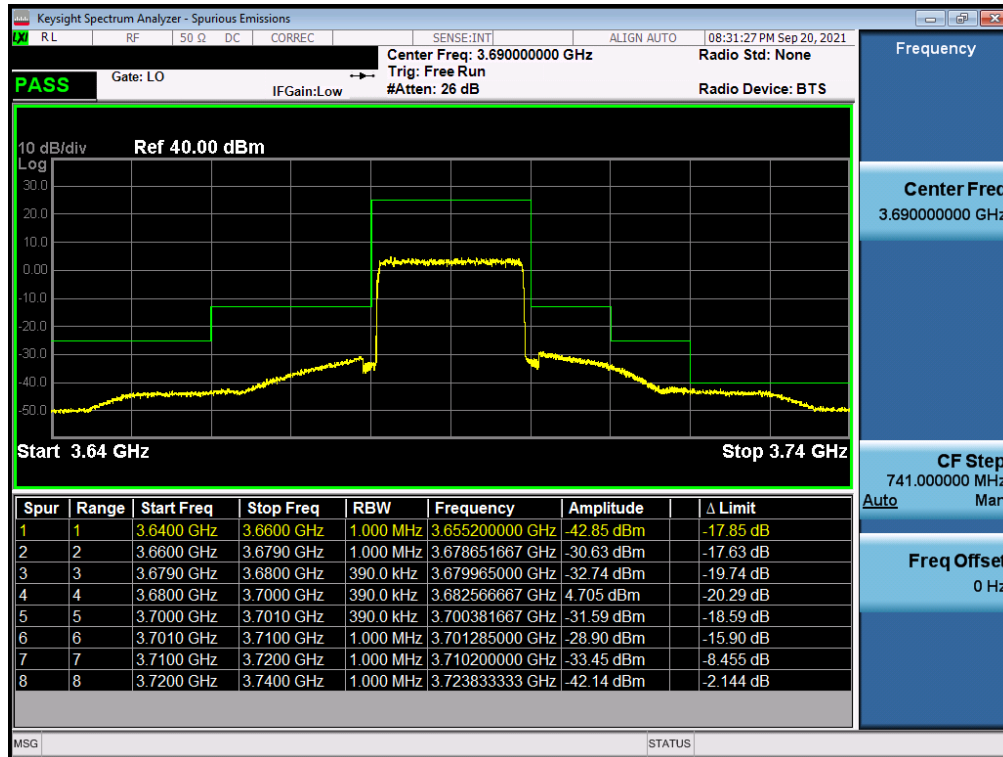
Plot 7-43. Channel Edge Plot (LTE Band 48 - 20MHz QPSK - High Channel)
