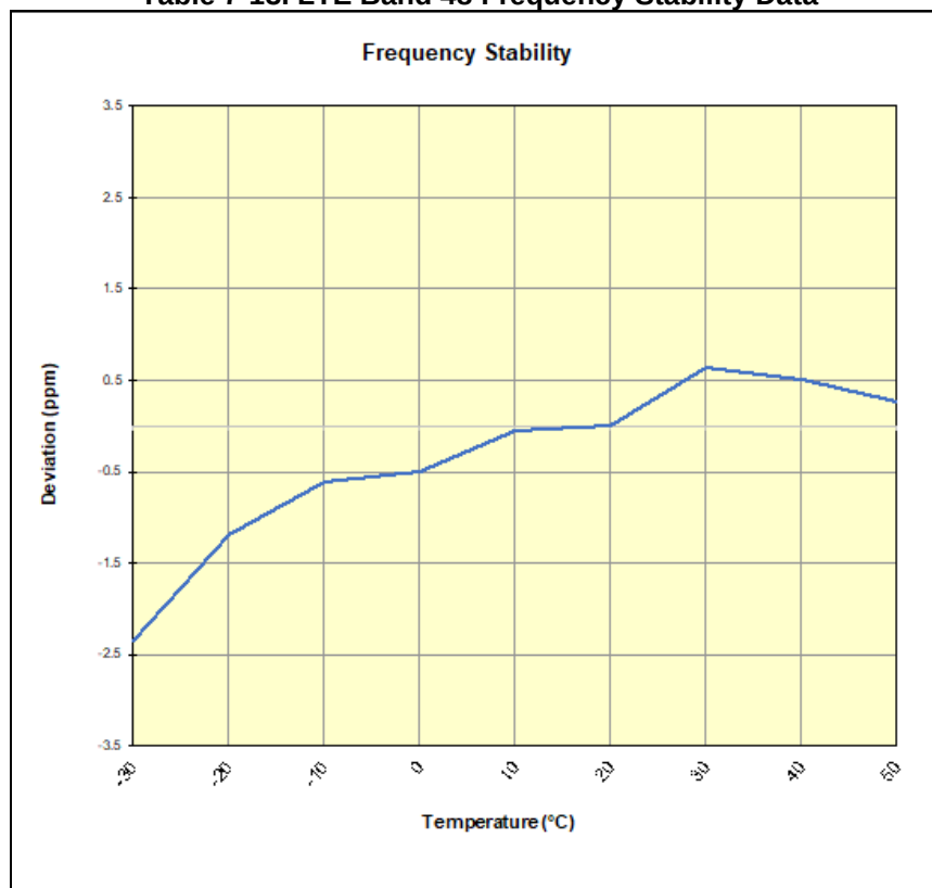
Plot 7-62. LTE Band 48 Frequency Stability Chart
