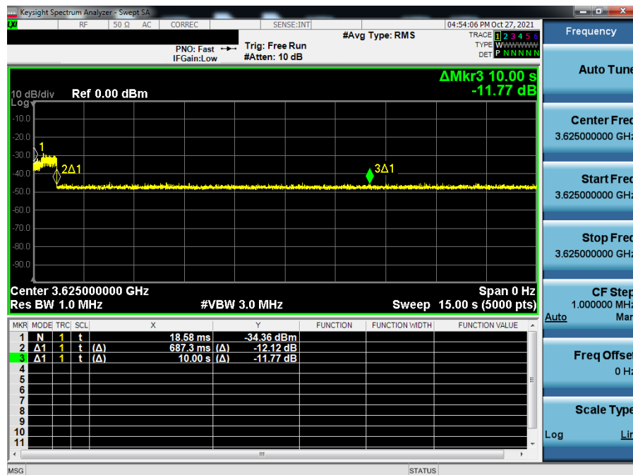
Plot 7-64. Run#1 End User Device Discontinues Operations within 10s
