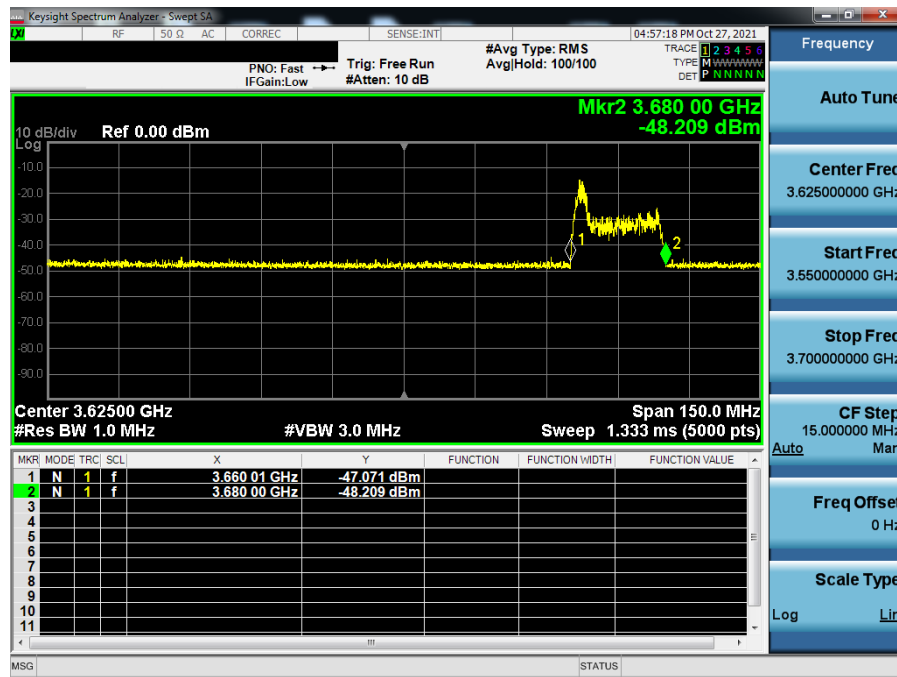
Plot 7-65. Run#2 End User Device Frequency of Operations
