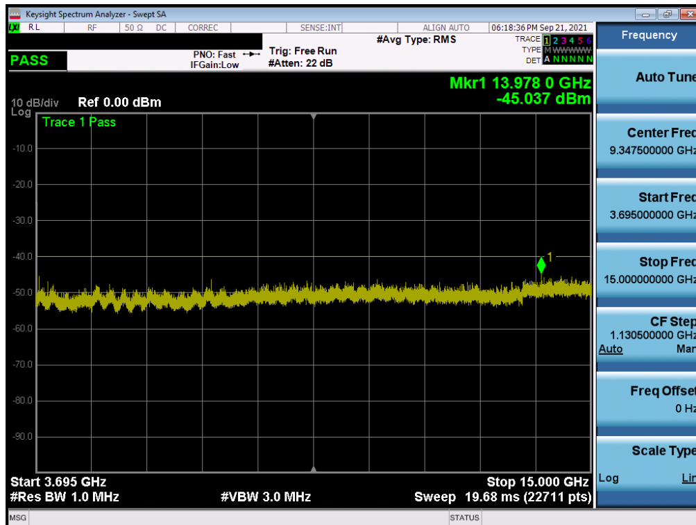
Plot 7-34. Conducted Spurious Plot (ULCA LB48 - 20+20MHz QPSK - Mid Channel)
