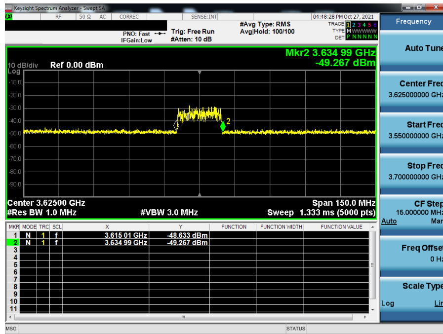
Plot 7-63. Run#1 End User Device Frequency of Operations
