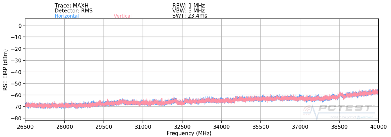
Plot 7-58. Radiated Spurious Plot (LTE Band 48, 26.5 – 40GHz)
