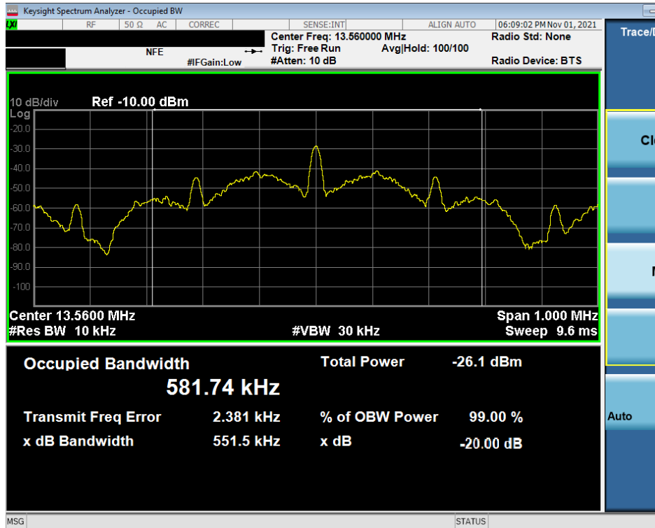
Figure 7-2. Occupied Bandwidth Plot
