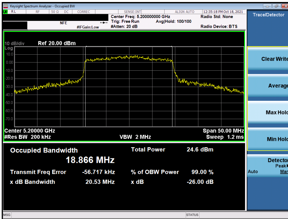
Plot 7-59. 26dB Bandwidth Plot SISO ANT2 (20MHz BW 802.11ax (UNII Band 1) – Ch. 40)
