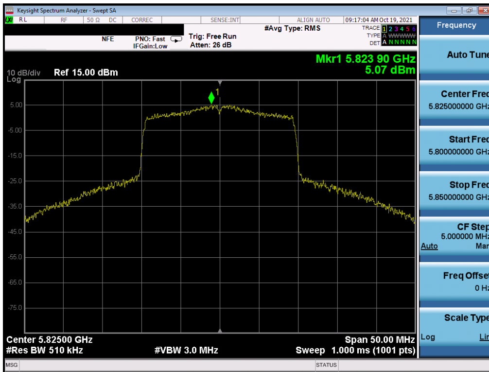
Plot 7-220. Power Spectral Density Plot SISO ANT1 (20MHz BW 802.11ax (UNII Band 3) – Ch. 165)
