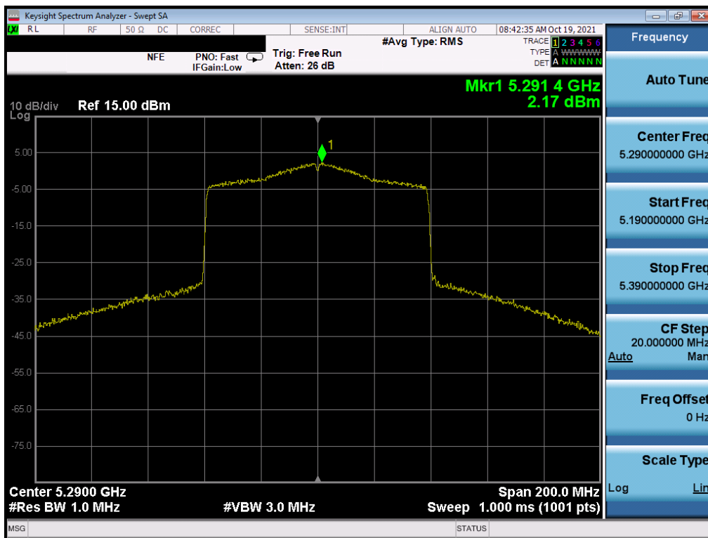
Plot 7-190. Power Spectral Density Plot SISO ANT1 (80MHz BW 802.11ax (UNII Band 2A) – Ch. 58)
