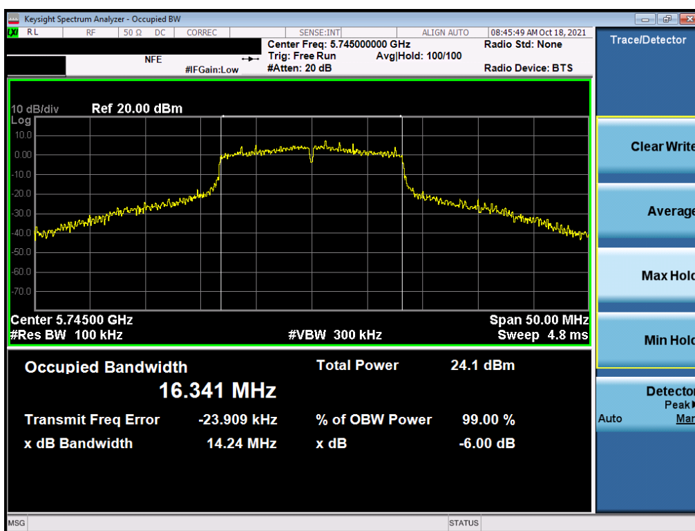
Plot 7-132. 6dB Bandwidth Plot SISO ANT2 (802.11a (UNII Band 3) – Ch. 149)
