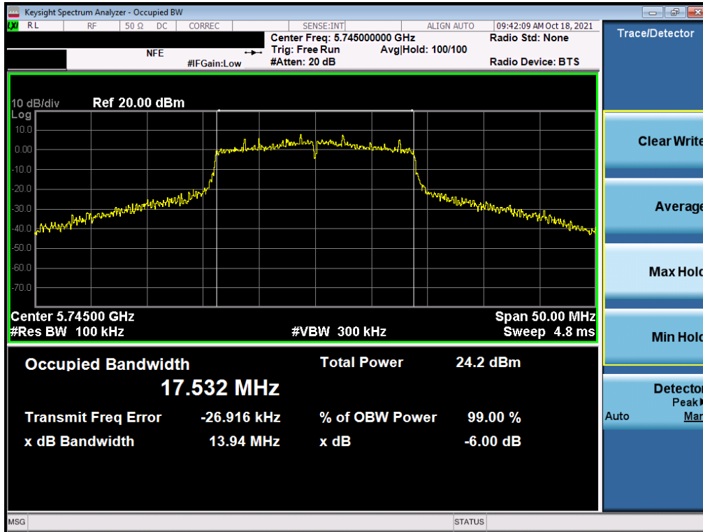
Plot 7-135. 6dB Bandwidth Plot SISO ANT2 (20MHz BW 802.11n (UNII Band 3) – Ch. 149)
