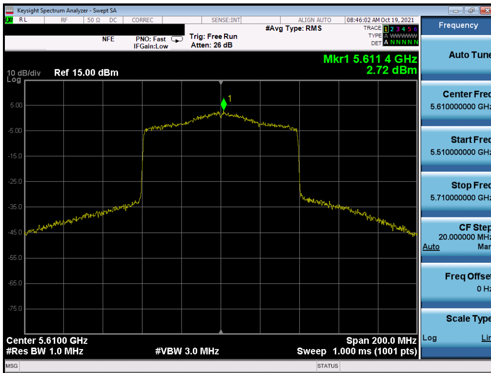
Plot 7-210. Power Spectral Density Plot SISO ANT1 (80MHz BW 802.11ax (UNII Band 2C) – Ch. 122)
