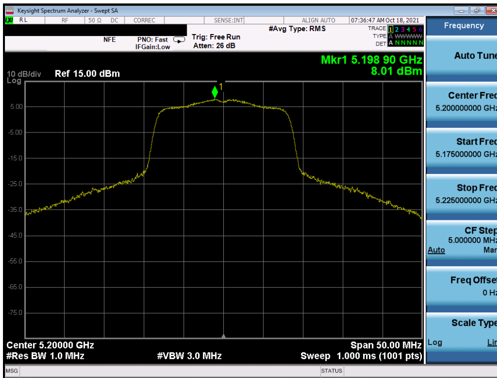
Plot 7-168. Power Spectral Density Plot SISO ANT1 (20MHz BW 802.11ax (UNII Band 1) – Ch. 40)
