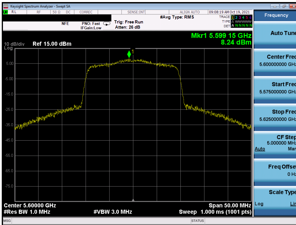
Plot 7-198. Power Spectral Density Plot SISO ANT1 (20MHz BW 802.11ax (UNII Band 2C) – Ch. 120)
