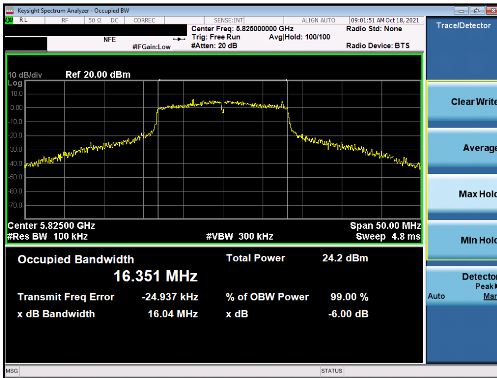
Plot 7-134. 6dB Bandwidth Plot SISO ANT2 (802.11a (UNII Band 3) – Ch. 165)
