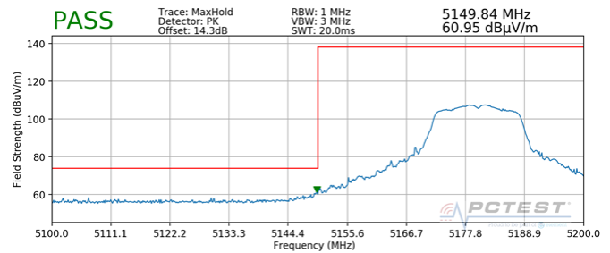
Plot 7-379. Radiated Lower Band Edge Plot SISO ANT2 (Peak – UNII Band 1)
