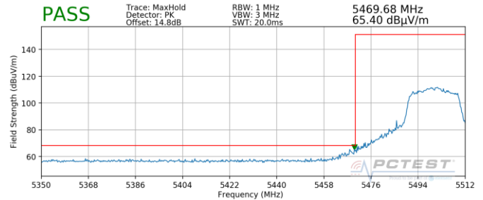
Plot 7-356. Radiated Lower Band Edge Plot SISO ANT1 (Peak – UNII Band 2C)
