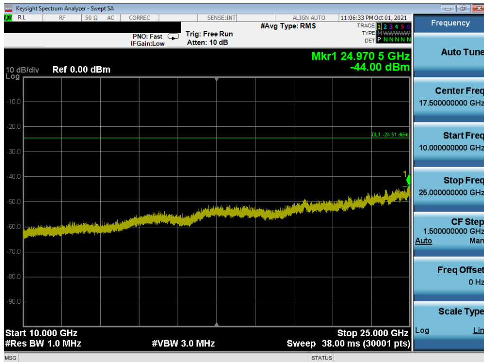
Plot 7-54. Conducted Spurious Plot SISO ANT2 (802.11ax OFDMA – 242 Tones – Ch. 1)
