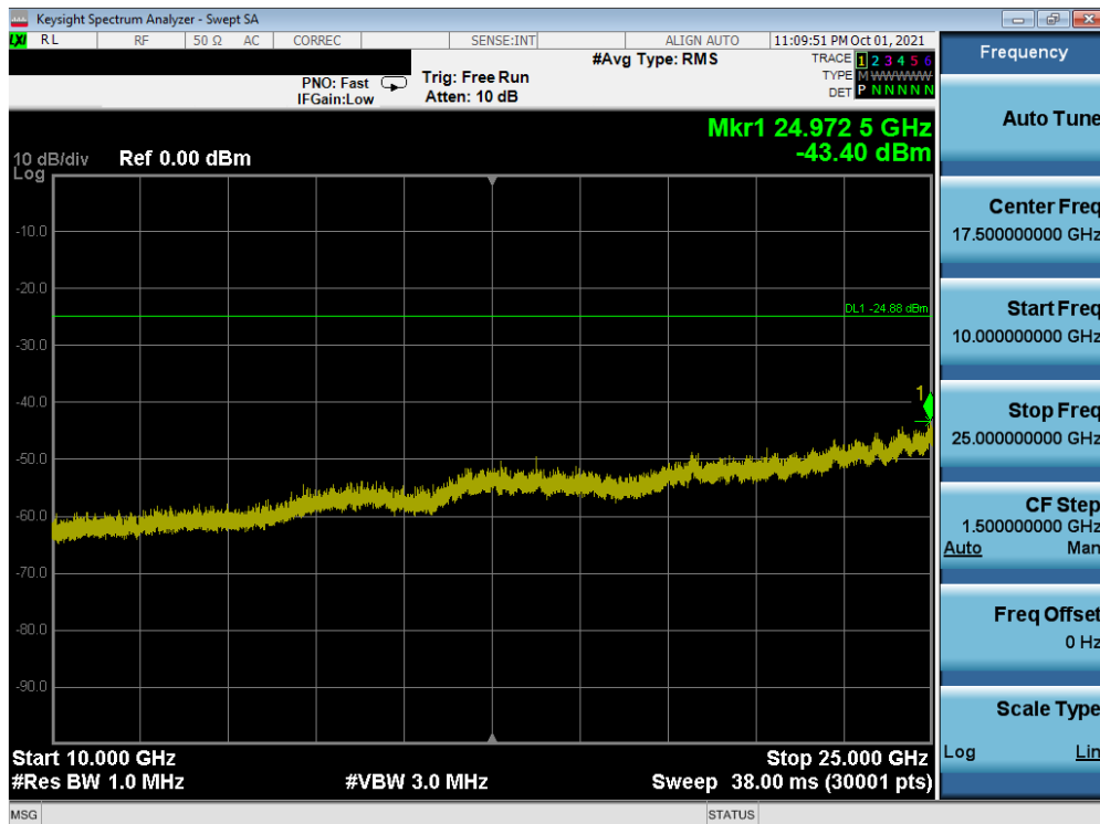
Plot 7-56. Conducted Spurious Plot SISO ANT2 (802.11ax OFDMA – 242 Tones – Ch. 6)
