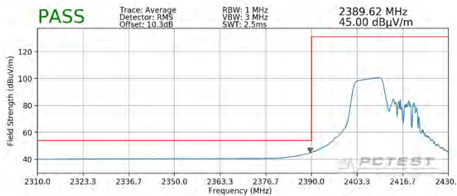
Plot 7-83. Radiated Restricted Lower Band Edge Measurement SISO ANT1 (Average – 106 Tones)
