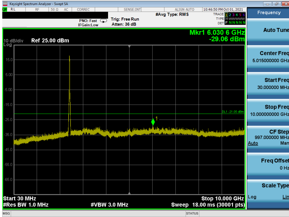
Plot 7-43. Conducted Spurious Plot SISO ANT1 (802.11ax OFDMA – 242 Tones – Ch. 6)
