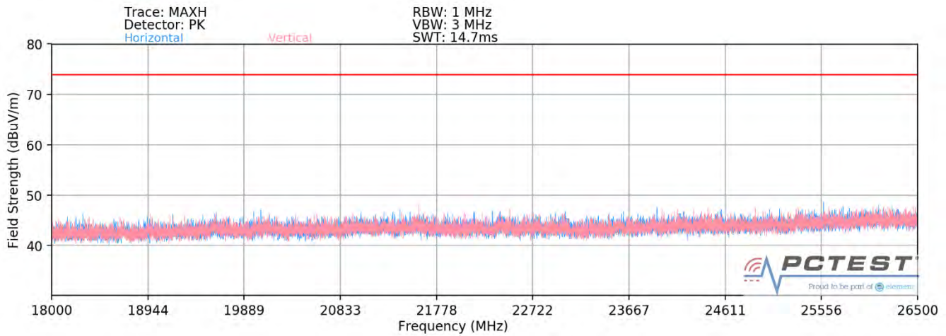
Plot 7-73. Radiated Spurious Plot above 18GHz SISO ANT2 (802.11ax OFDMA – 106 Tones)
