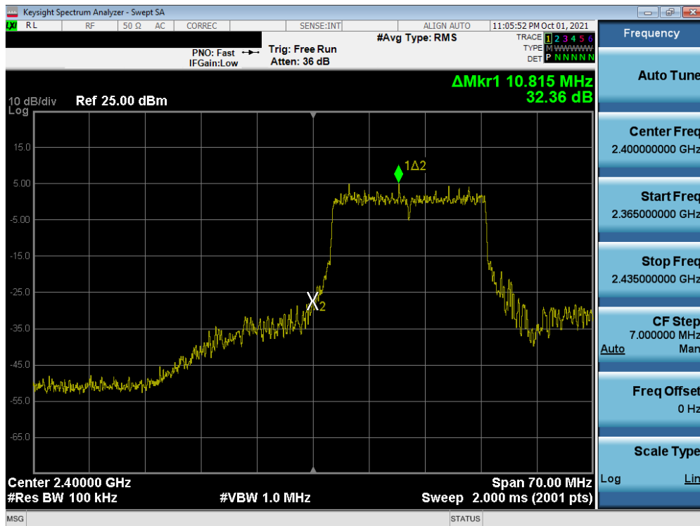
Plot 7-32. Band Edge Plot SISO ANT2 (802.11ax OFDMA – 242 Tones – Ch. 1)
