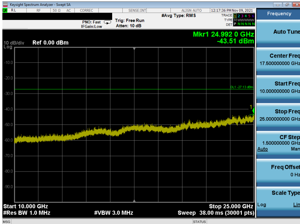
Plot 7-58. Conducted Spurious Plot SISO ANT2 (802.11ax OFDMA – 242 Tones – Ch. 11)
