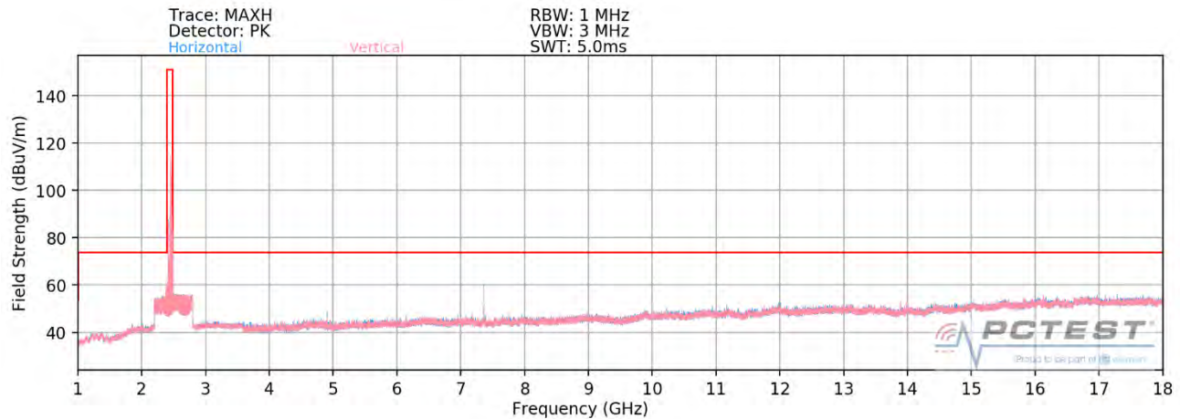
Plot 7-77. Radiated Spurious Plot above 1GHz MIMO (802.11ax OFDMA – 106 Tones – Ch. 11)
