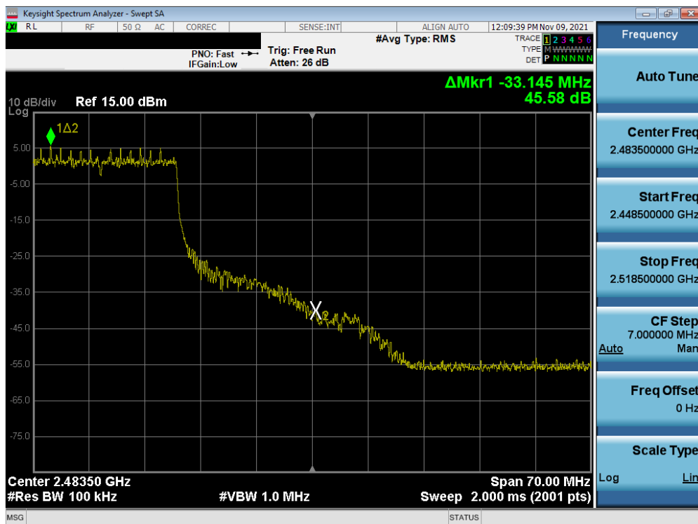
Plot 7-33. Band Edge Plot SISO ANT2 (802.11ax OFDMA – 242 Tones – Ch. 10)
