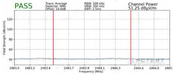
Plot 7-101. Radiated Restricted Upper Band Edge Measurement SISO ANT2 (Average – 242 Tones)
