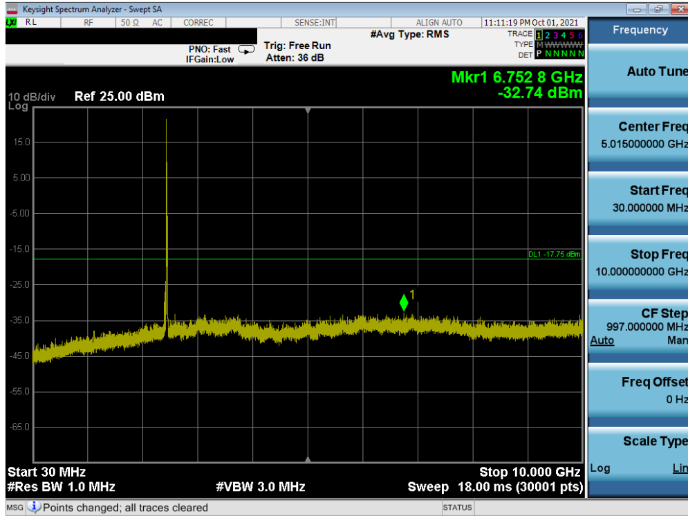
Plot 7-51. Conducted Spurious Plot SISO ANT2 (802.11ax OFDMA – 26 Tones – Ch. 11)
