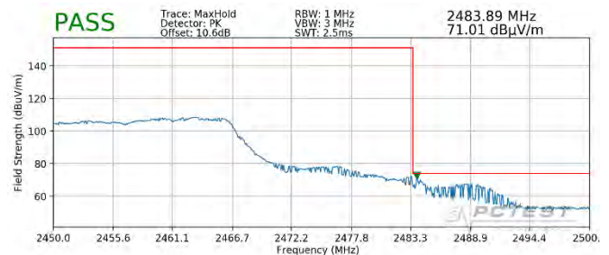
Plot 7-90. Radiated Restricted Upper Band Edge Measurement SISO ANT1 (Peak – 242 Tones)
