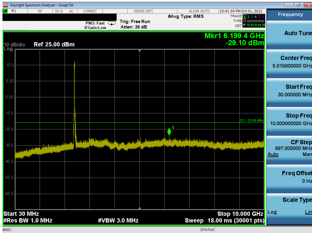
Plot 7-41. Conducted Spurious Plot SISO ANT1 (802.11ax OFDMA – 242 Tones – Ch. 1)
