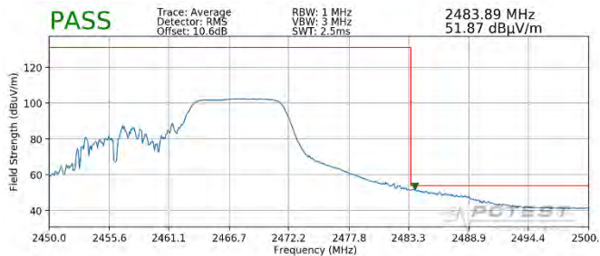
Plot 7-105. Radiated Restricted Upper Band Edge Measurement MIMO (Average – 106 Tones)
