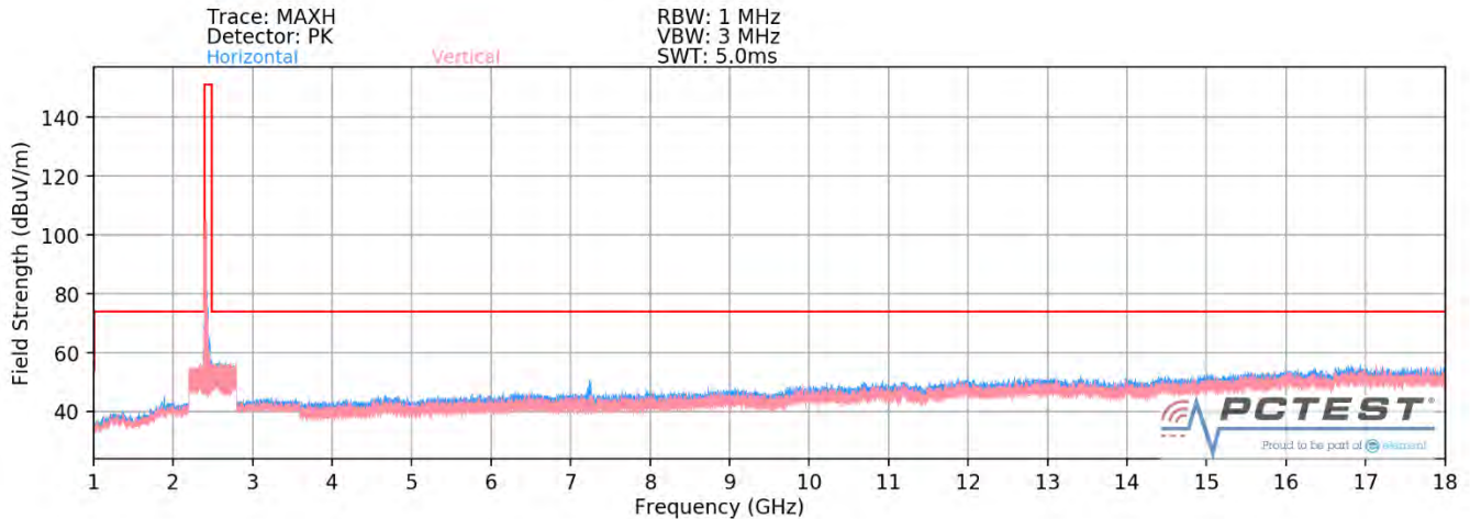
Plot 7-78. Radiated Spurious Plot above 1GHz MIMO (802.11ax OFDMA – 242 Tones – Ch. 1)
