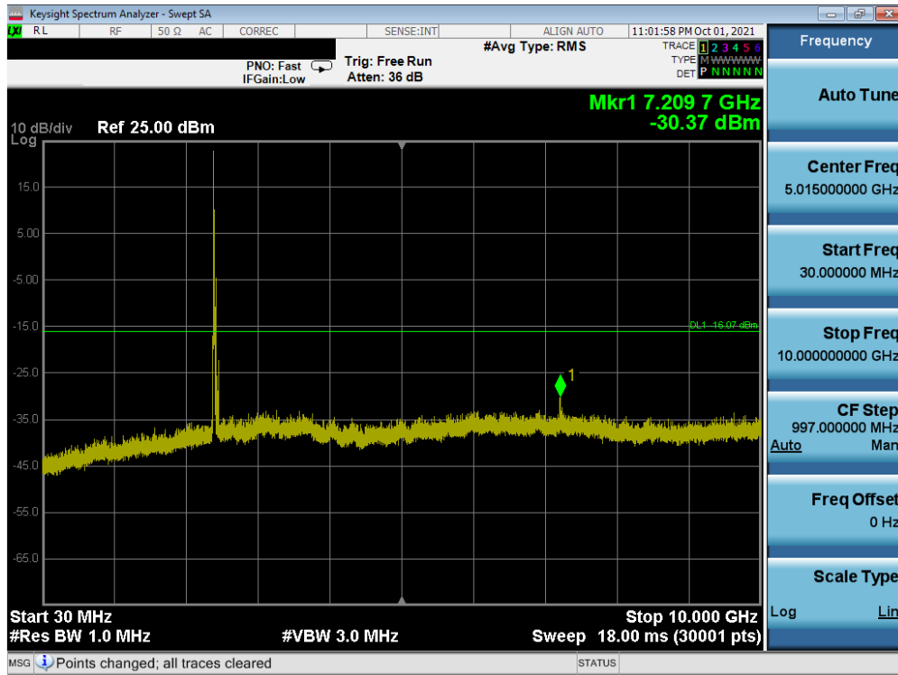
Plot 7-47. Conducted Spurious Plot SISO ANT2 (802.11ax OFDMA – 26 Tones – Ch. 1)
