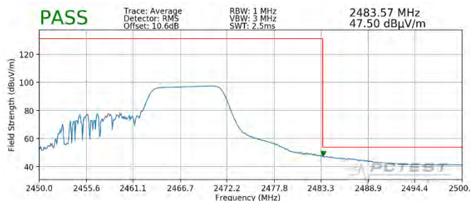
Plot 7-95. Radiated Restricted Upper Band Edge Measurement SISO ANT2 (Average – 106 Tones)
