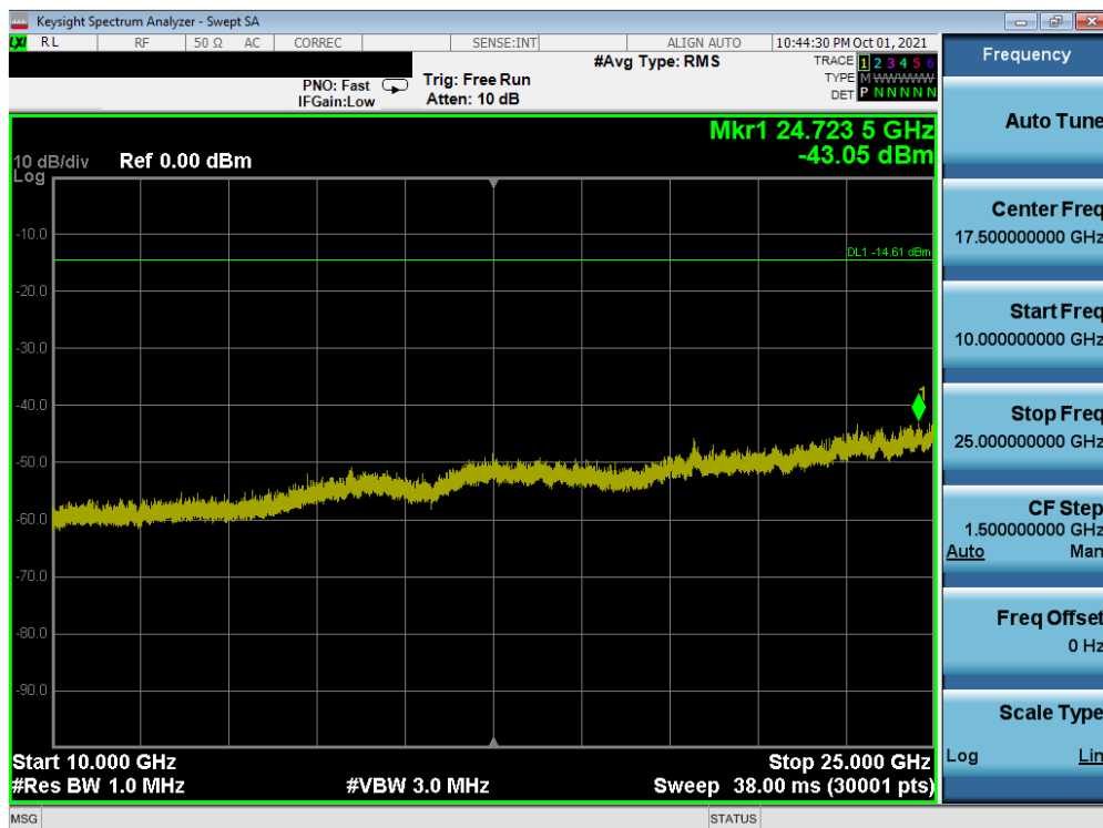
Plot 7-38. Conducted Spurious Plot SISO ANT1 (802.11ax OFDMA – 26 Tones – Ch. 6)
