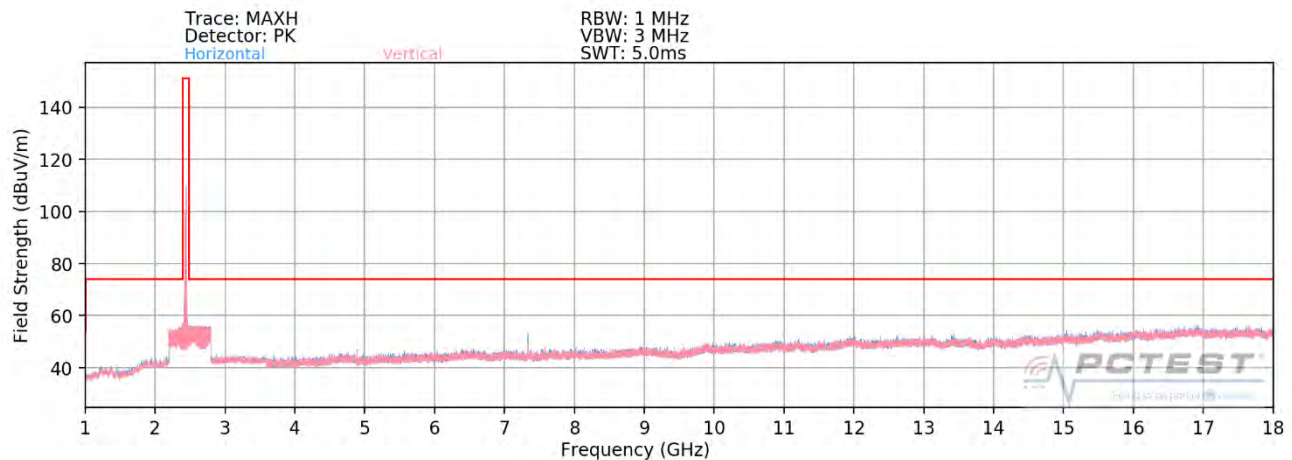
Plot 7-68. Radiated Spurious Plot above 1GHz SISO ANT2 (802.11ax OFDMA – 106 Tones – Ch. 6)
