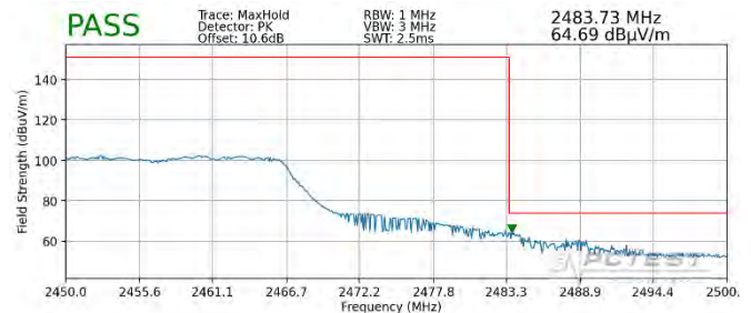
Plot 7-100. Radiated Restricted Upper Band Edge Measurement SISO ANT2 (Peak – 242 Tones)
