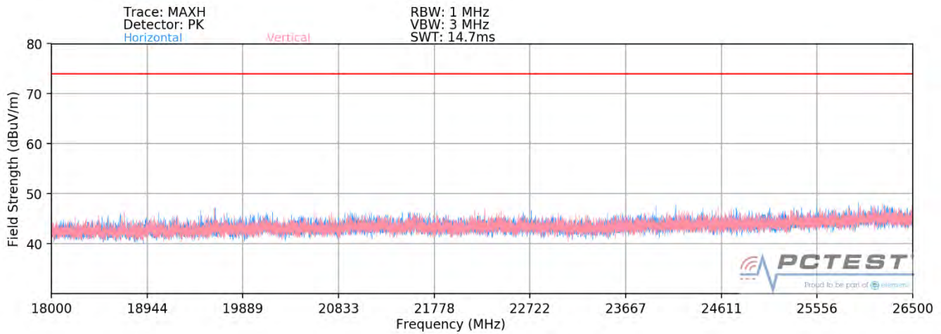
Plot 7-65. Radiated Spurious Plot above 18GHz SISO ANT1 (802.11ax OFDMA – 106 Tones)
