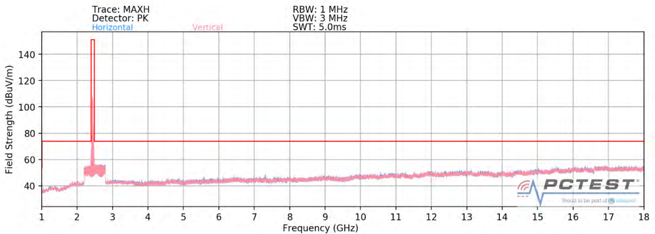
Plot 7-79. Radiated Spurious Plot above 1GHz MIMO (802.11ax OFDMA – 242 Tones – Ch. 6)
