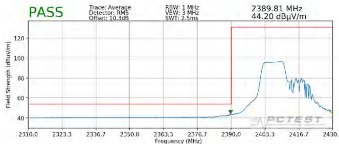
Plot 7-93. Radiated Restricted Lower Band Edge Measurement SISO ANT2 (Average – 106 Tones)
