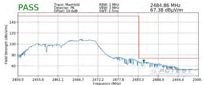
Plot 7-96. Radiated Restricted Upper Band Edge Measurement SISO ANT2 (Peak – 106 Tones)
