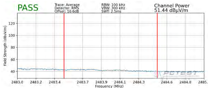
Plot 7-89. Radiated Restricted Upper Band Edge Measurement SISO ANT1 (Average – 242 Tones)
