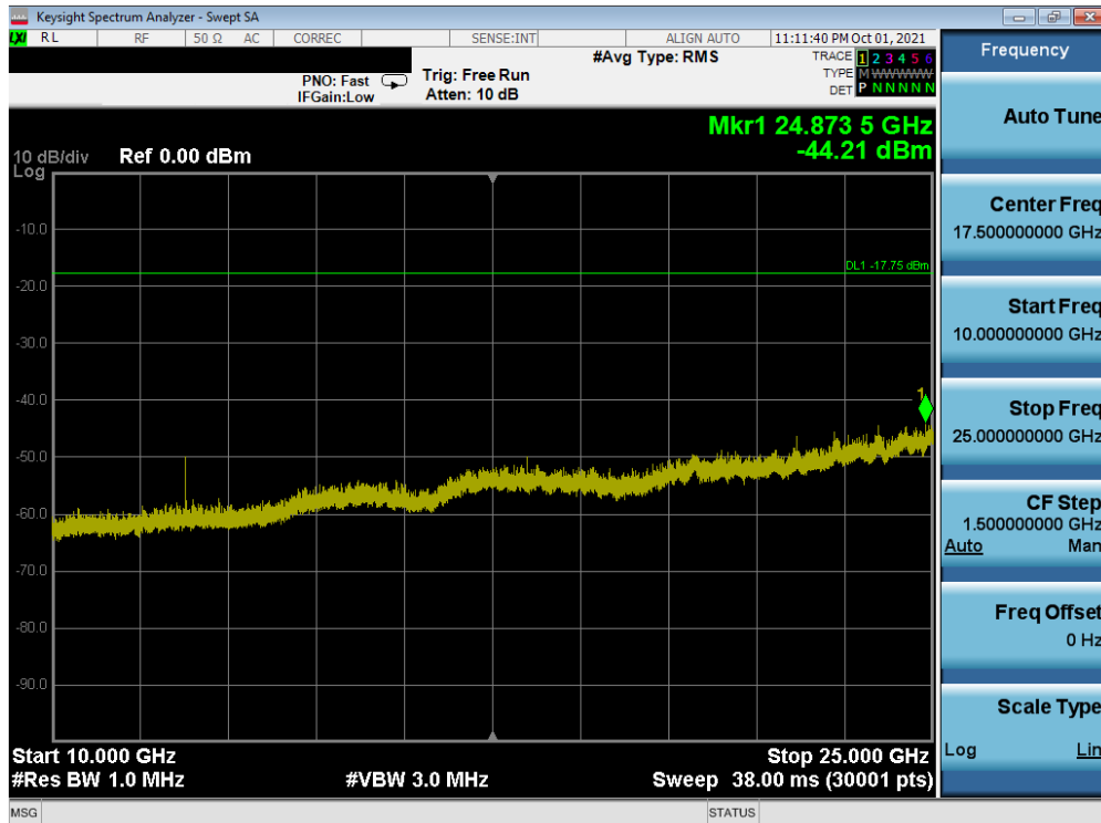
Plot 7-52. Conducted Spurious Plot SISO ANT2 (802.11ax OFDMA – 26 Tones – Ch. 11)
