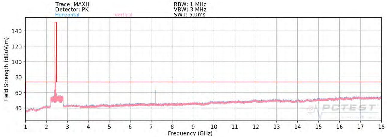
Plot 7-75. Radiated Spurious Plot above 1GHz MIMO (802.11ax OFDMA – 106 Tones – Ch. 1)
