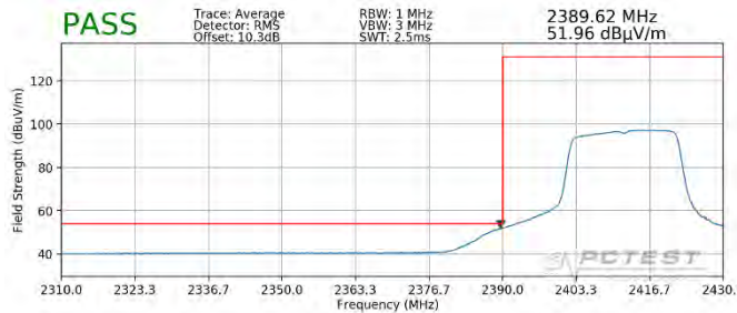
Plot 7-87. Radiated Restricted Lower Band Edge Measurement SISO ANT1 (Average – 242 Tones)
