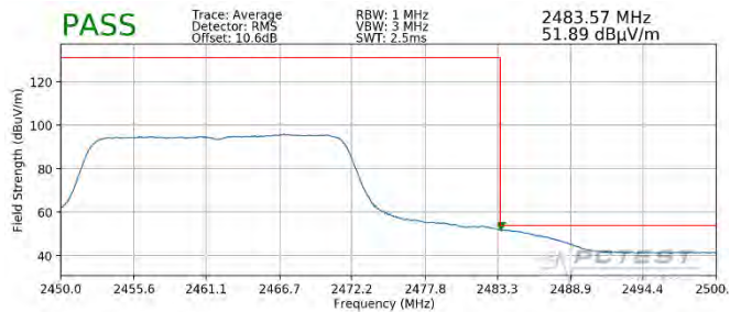
Plot 7-111. Radiated Restricted Upper Band Edge Measurement MIMO (Average – 242 Tones)
