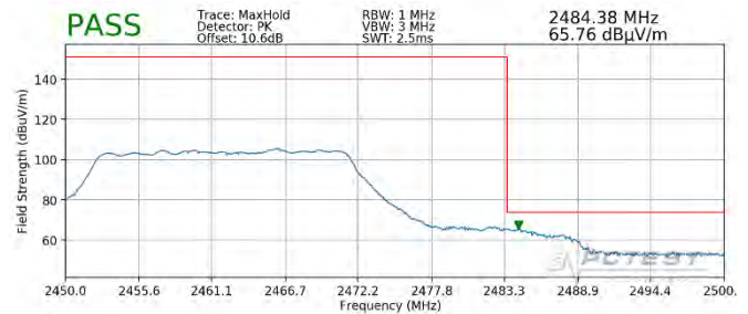
Plot 7-112. Radiated Restricted Upper Band Edge Measurement MIMO (Peak – 242 Tones)
