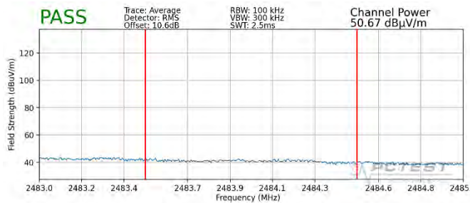
Plot 7-109. Radiated Restricted Upper Band Edge Measurement MIMO (Average – 242 Tones)
