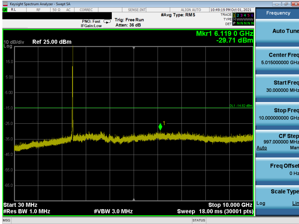
Plot 7-39. Conducted Spurious Plot SISO ANT1 (802.11ax OFDMA – 26 Tones – Ch. 11)
