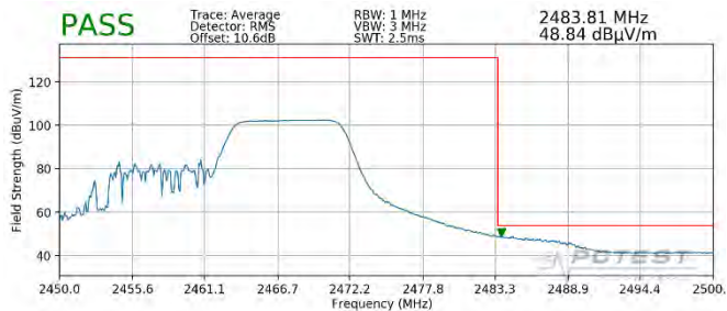
Plot 7-85. Radiated Restricted Upper Band Edge Measurement SISO ANT1 (Average – 106 Tones)
