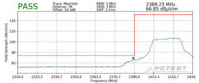
Plot 7-88. Radiated Restricted Lower Band Edge Measurement SISO ANT1 (Peak – 242 Tones)
