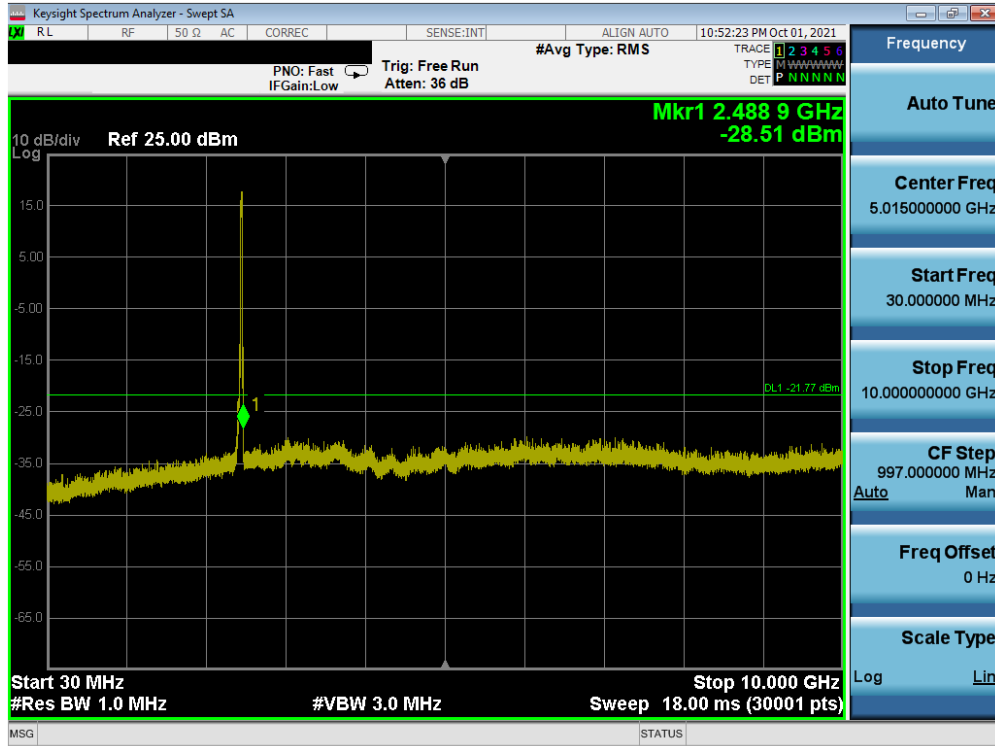
Plot 7-45. Conducted Spurious Plot SISO ANT1 (802.11ax OFDMA – 242 Tones – Ch. 11)
