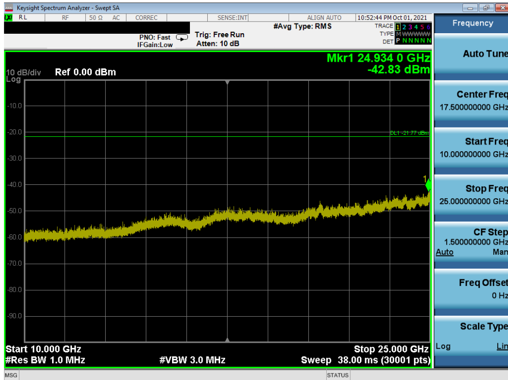
Plot 7-46. Conducted Spurious Plot SISO ANT1 (802.11ax OFDMA – 242 Tones – Ch. 11)
