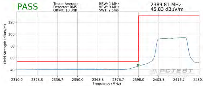
Plot 7-97. Radiated Restricted Lower Band Edge Measurement SISO ANT2 (Average – 242 Tones)
