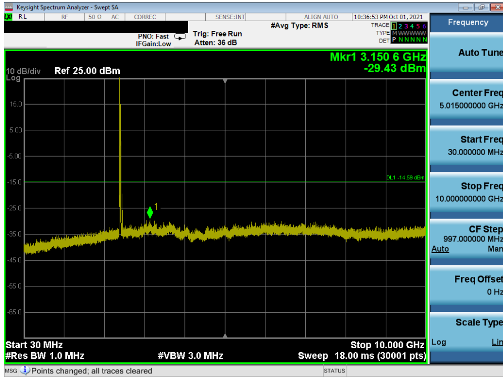
Plot 7-35. Conducted Spurious Plot SISO ANT1 (802.11ax OFDMA – 26 Tones – Ch. 1)
