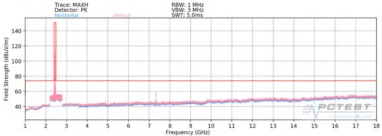
Plot 7-76. Radiated Spurious Plot above 1GHz MIMO (802.11ax OFDMA – 106 Tones – Ch. 6)
