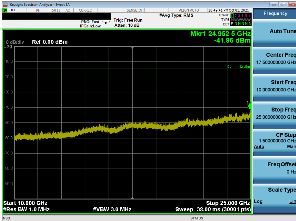
Plot 7-40. Conducted Spurious Plot SISO ANT1 (802.11ax OFDMA – 26 Tones – Ch. 11)
