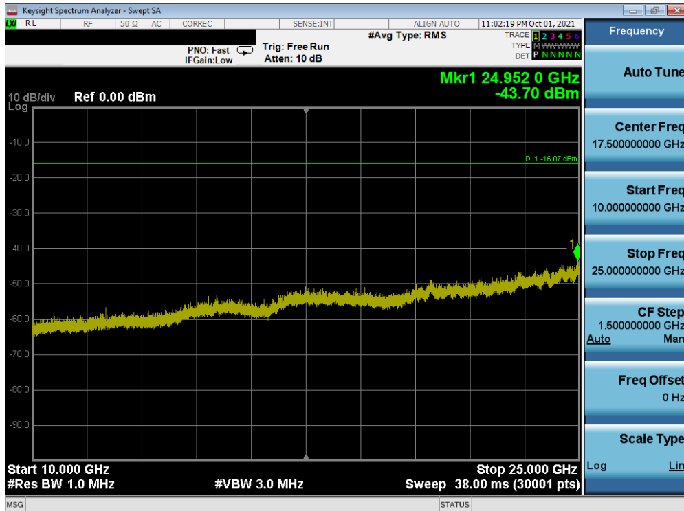
Plot 7-48. Conducted Spurious Plot SISO ANT2 (802.11ax OFDMA – 26 Tones – Ch. 1)
