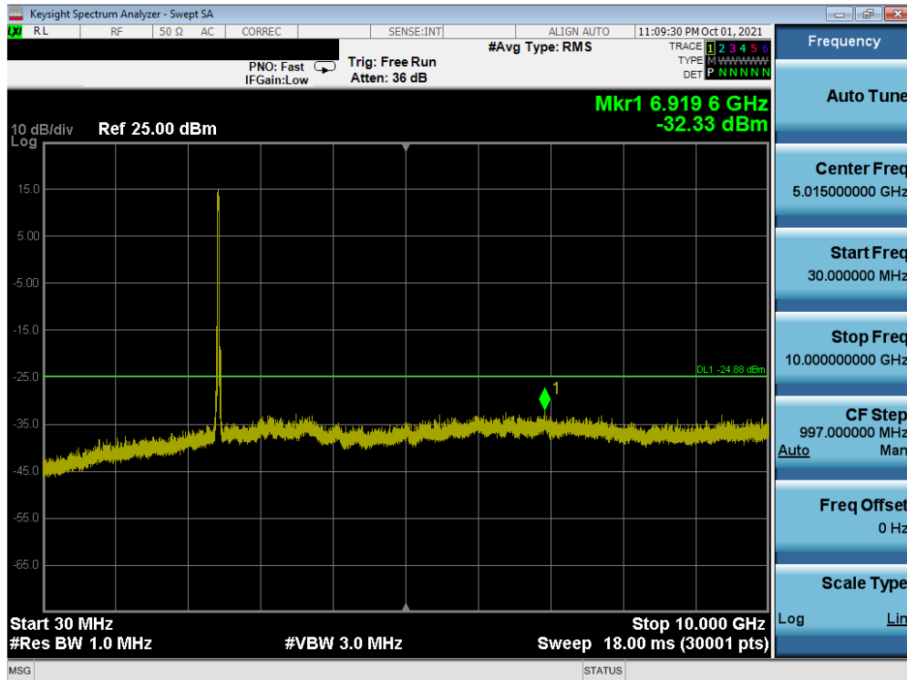
Plot 7-55. Conducted Spurious Plot SISO ANT2 (802.11ax OFDMA – 242 Tones – Ch. 6)
