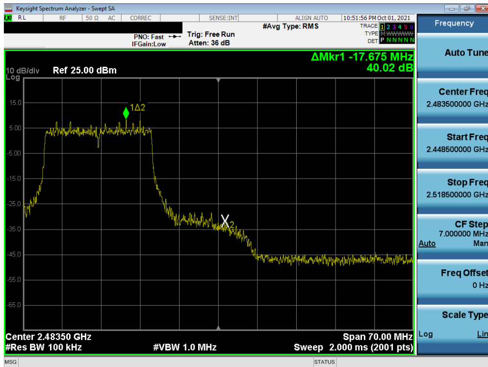
Plot 7-29. Band Edge Plot SISO ANT1 (802.11ax OFDMA – 242 Tones – Ch. 11)
