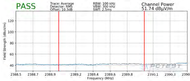
Plot 7-107. Radiated Restricted Lower Band Edge Measurement MIMO (Average – 242 Tones)
