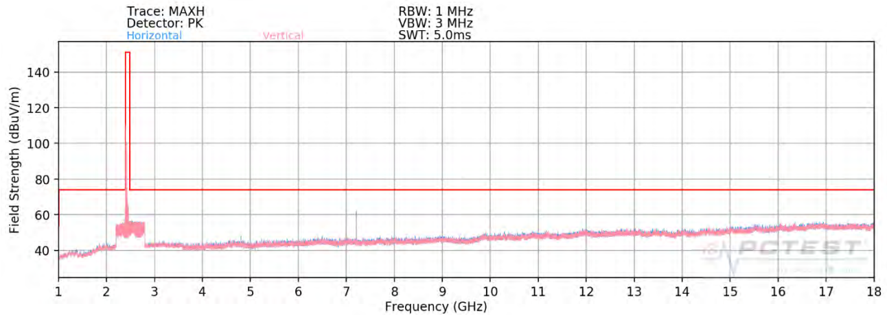
Plot 7-67. Radiated Spurious Plot above 1GHz SISO ANT2 (802.11ax OFDMA – 106 Tones – Ch. 1)
