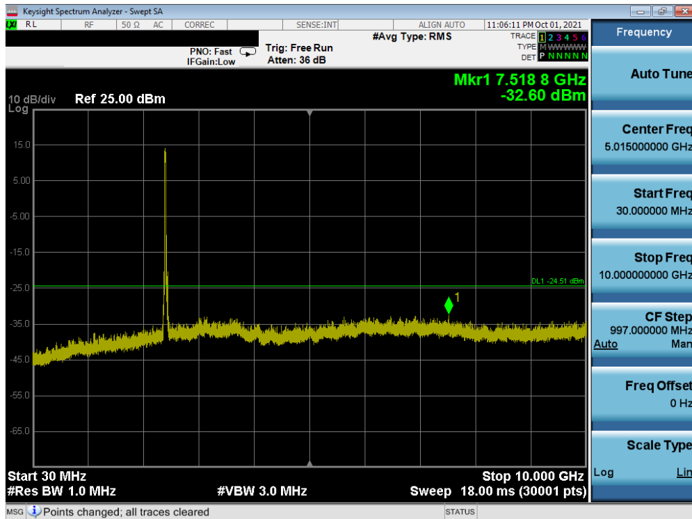
Plot 7-53. Conducted Spurious Plot SISO ANT2 (802.11ax OFDMA – 242 Tones – Ch. 1)
