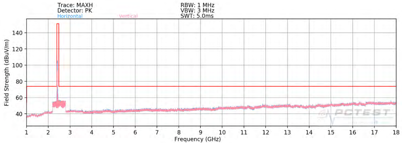
Plot 7-59. Radiated Spurious Plot above 1GHz SISO ANT1 (802.11ax OFDMA – 106 Tones – Ch. 1)
