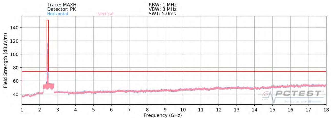
Plot 7-60. Radiated Spurious Plot above 1GHz SISO ANT1 (802.11ax OFDMA – 106 Tones – Ch. 6)
