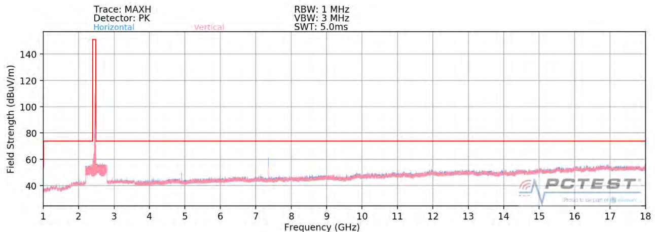
Plot 7-69. Radiated Spurious Plot above 1GHz SISO ANT2 (802.11ax OFDMA – 106 Tones – Ch. 11)
