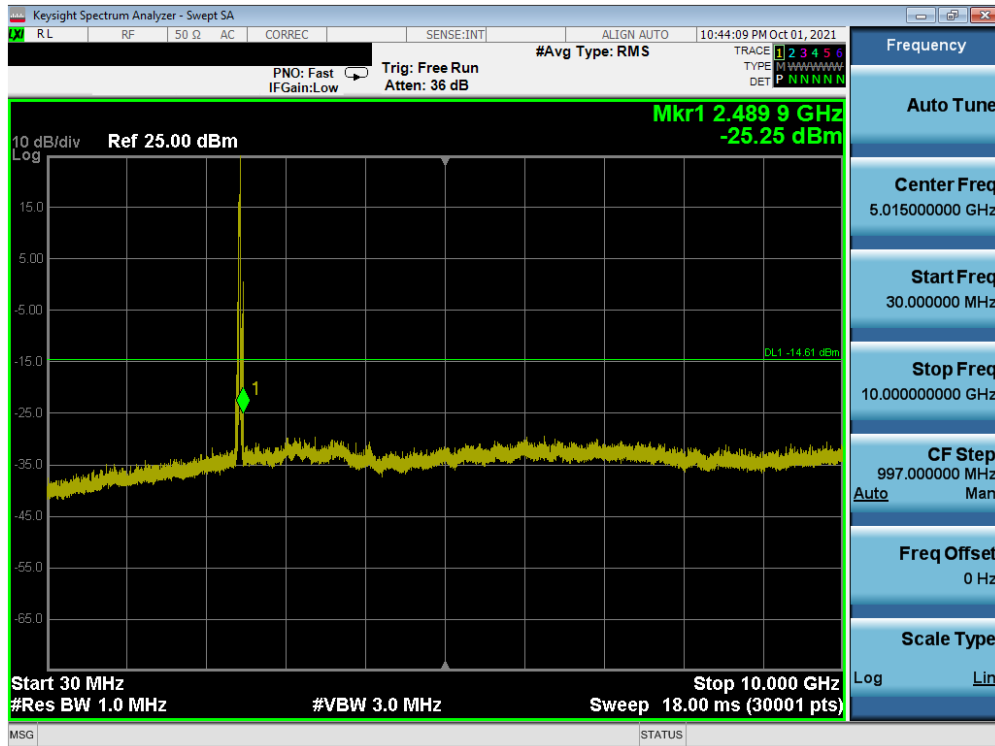
Plot 7-37. Conducted Spurious Plot SISO ANT1 (802.11ax OFDMA – 26 Tones – Ch. 6)
