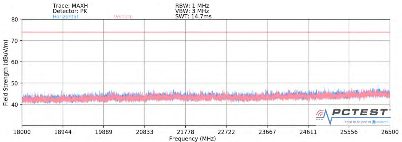
Plot 7-74. Radiated Spurious Plot above 18GHz SISO ANT2 (802.11ax OFDMA – 242 Tones)
