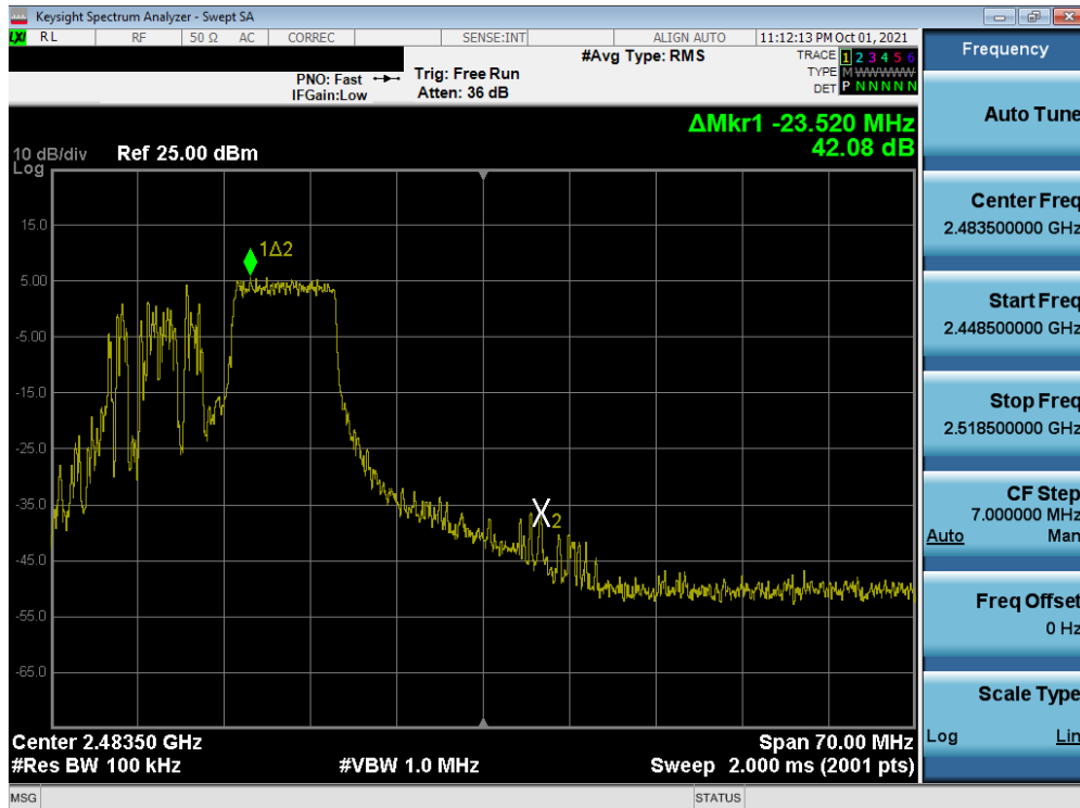
Plot 7-31. Band Edge Plot SISO ANT2 (802.11ax OFDMA – 106 Tones – Ch. 11)
