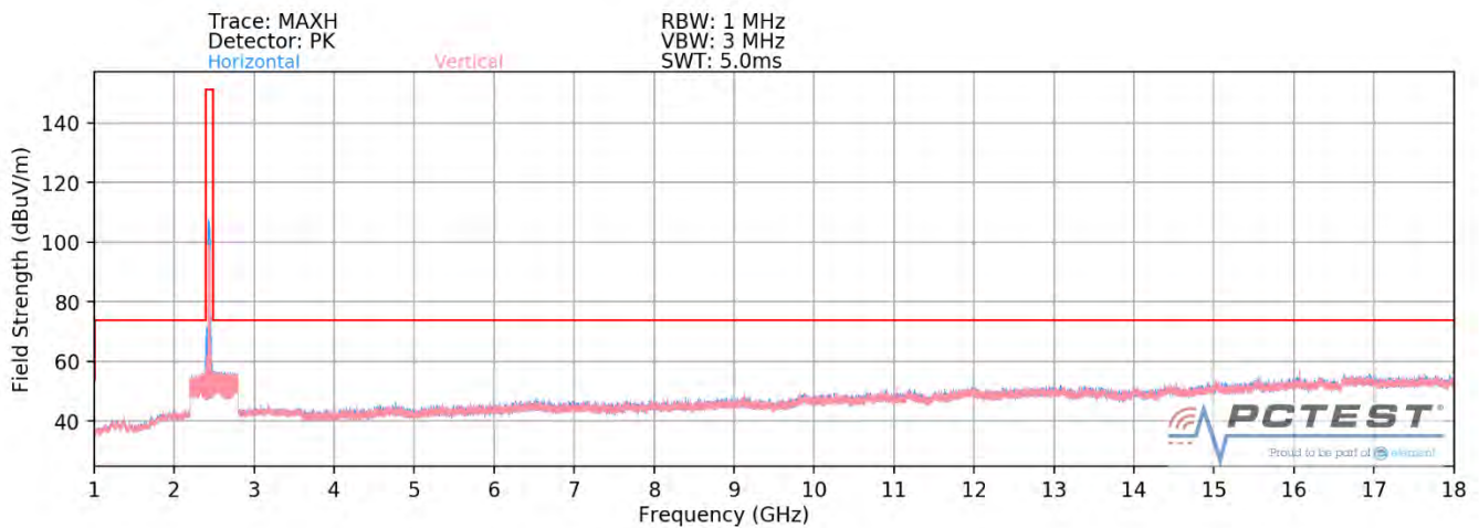
Plot 7-71. Radiated Spurious Plot above 1GHz SISO ANT2 (802.11ax OFDMA – 242 Tones – Ch. 6)
