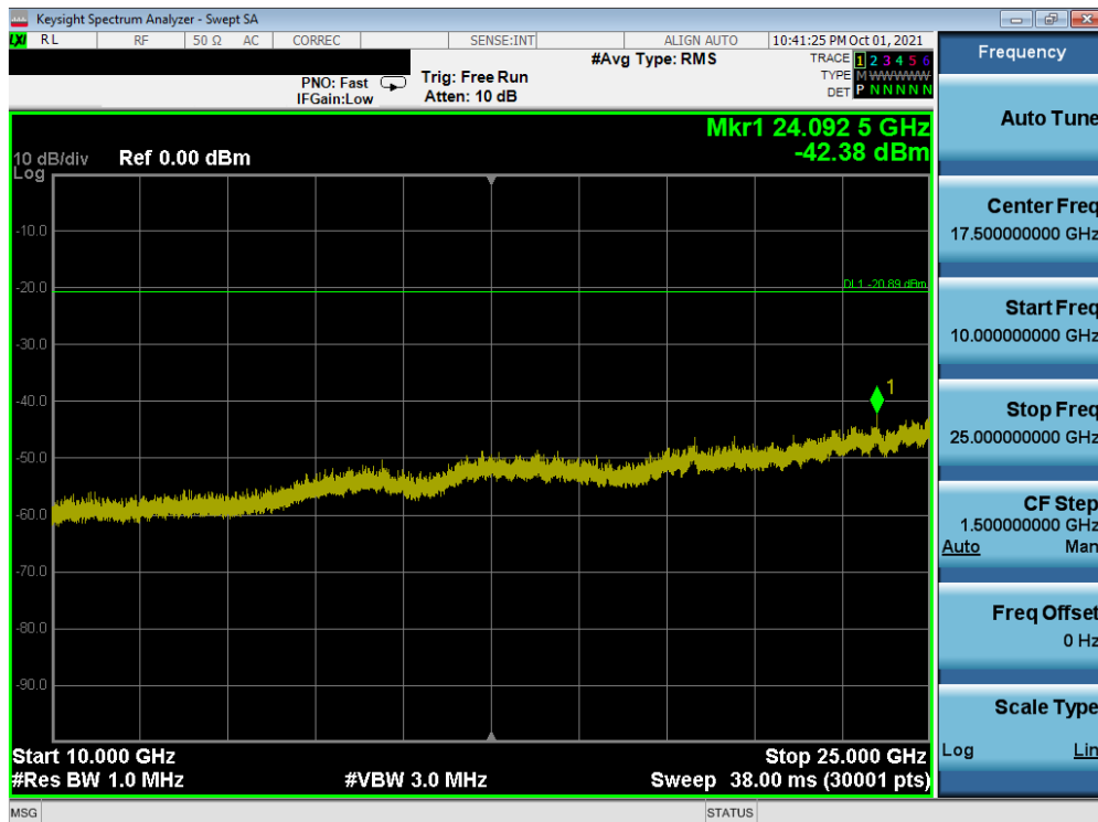
Plot 7-42. Conducted Spurious Plot SISO ANT1 (802.11ax OFDMA – 242 Tones – Ch. 1)
