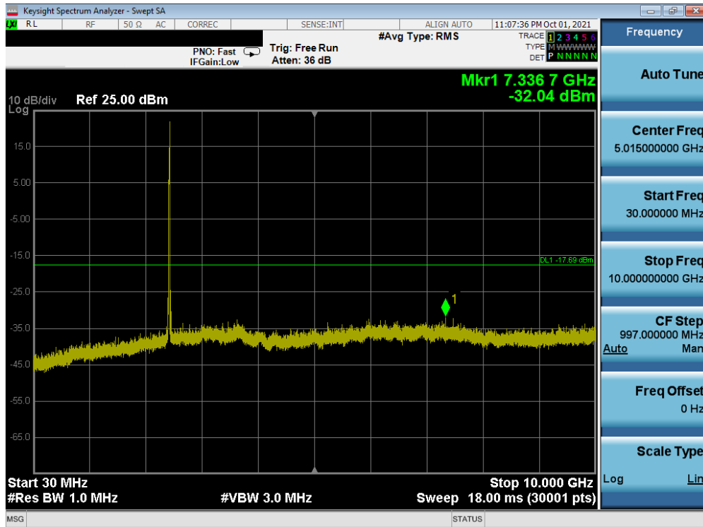
Plot 7-49. Conducted Spurious Plot SISO ANT2 (802.11ax OFDMA – 26 Tones – Ch. 6)
