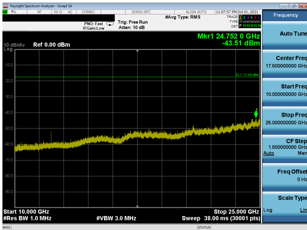
Plot 7-50. Conducted Spurious Plot SISO ANT2 (802.11ax OFDMA – 26 Tones – Ch. 6)
