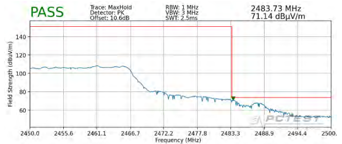
Plot 7-110. Radiated Restricted Upper Band Edge Measurement MIMO (Peak – 242 Tones)
