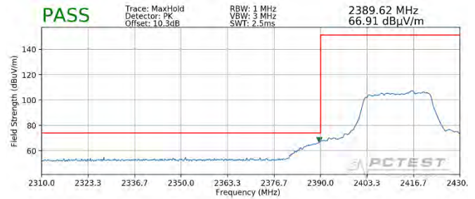
Plot 7-108. Radiated Restricted Lower Band Edge Measurement MIMO (Peak – 242 Tones)
