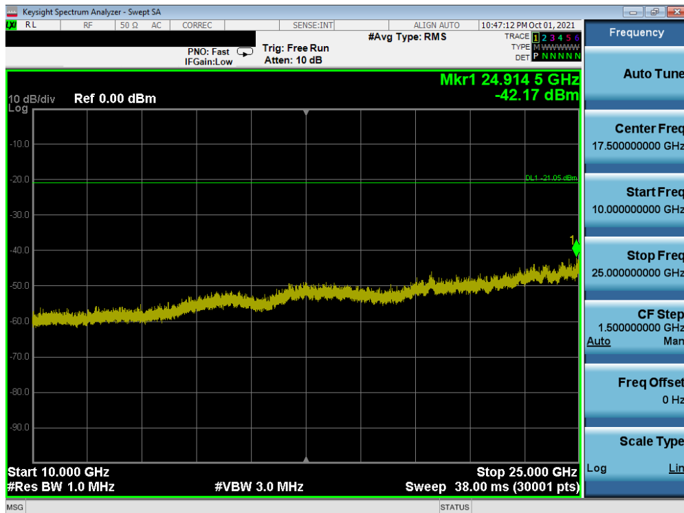
Plot 7-44. Conducted Spurious Plot SISO ANT1 (802.11ax OFDMA – 242 Tones – Ch. 6)
