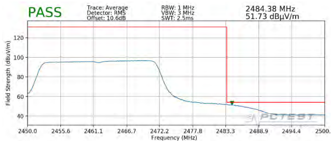
Plot 7-91. Radiated Restricted Upper Band Edge Measurement SISO ANT1 (Average – 242 Tones)
