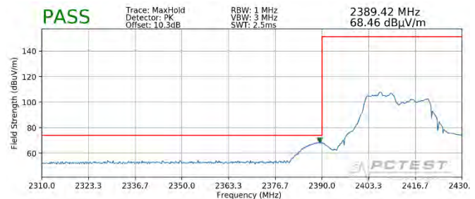
Plot 7-94. Radiated Restricted Lower Band Edge Measurement SISO ANT2 (Peak – 106 Tones)
