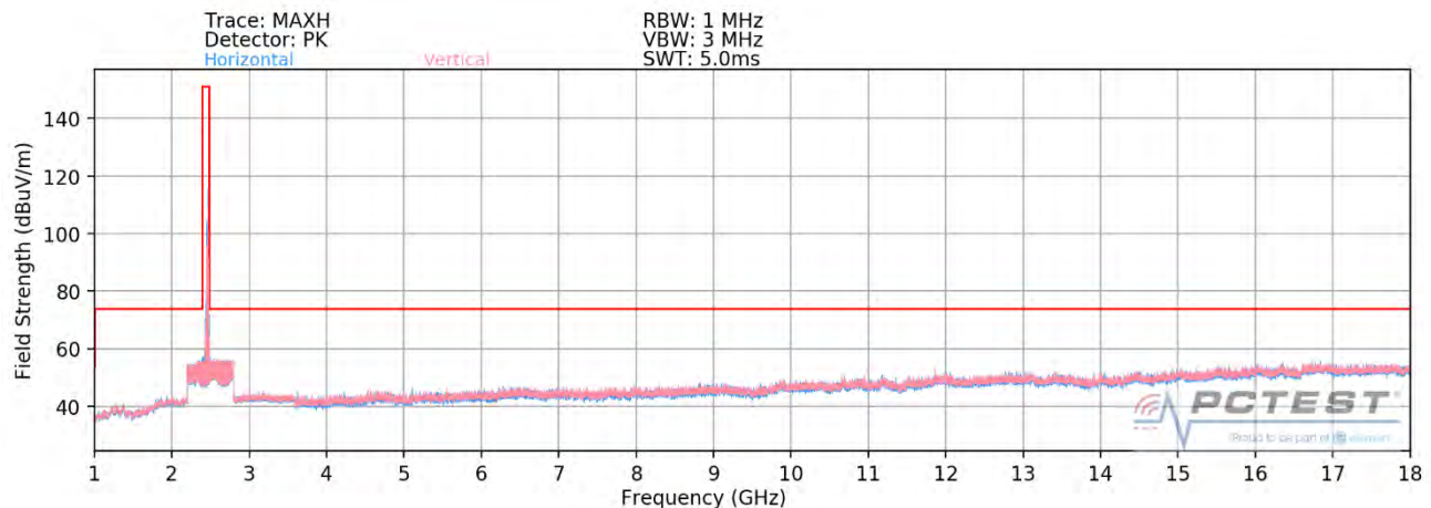
Plot 7-61. Radiated Spurious Plot above 1GHz SISO ANT1 (802.11ax OFDMA – 106 Tones – Ch. 11)
