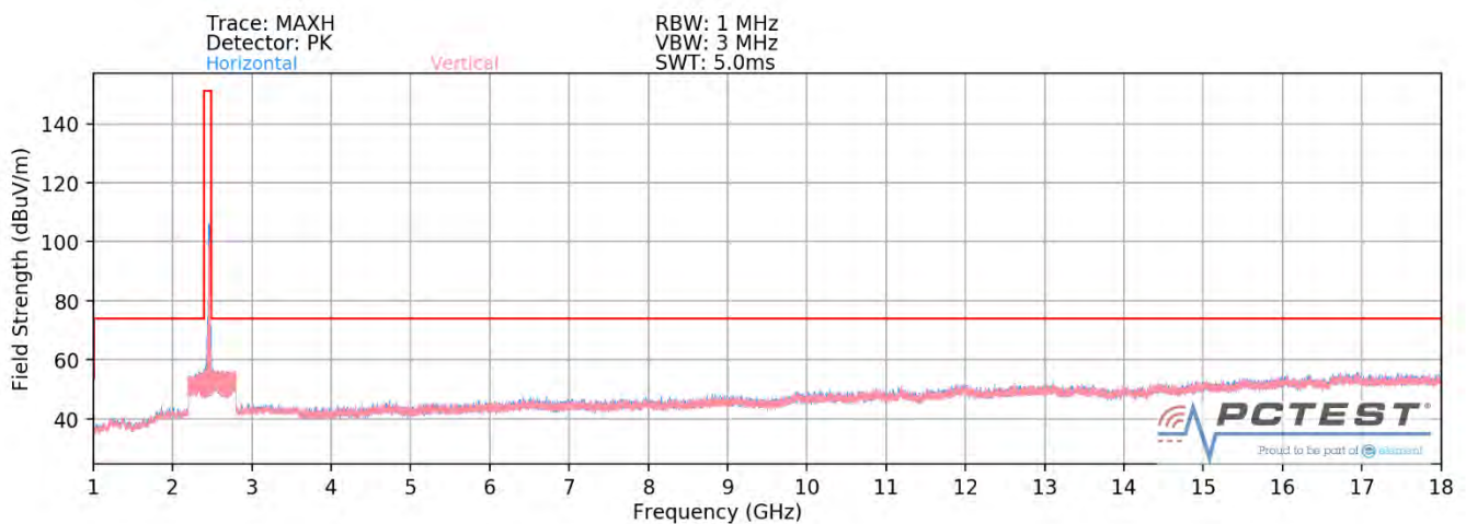
Plot 7-64. Radiated Spurious Plot above 1GHz SISO ANT1 (802.11ax OFDMA – 242 Tones – Ch. 11)
