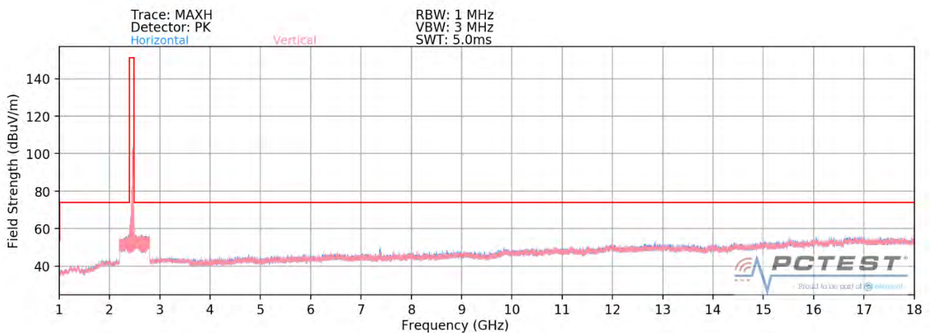
Plot 7-72. Radiated Spurious Plot above 1GHz SISO ANT2 (802.11ax OFDMA – 242 Tones – Ch. 11)
