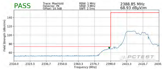
Plot 7-104. Radiated Restricted Lower Band Edge Measurement MIMO (Peak – 106 Tones)
