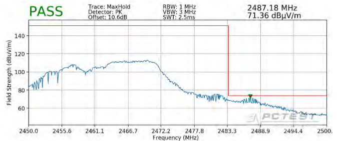
Plot 7-106. Radiated Restricted Upper Band Edge Measurement MIMO (Peak – 106 Tones)
