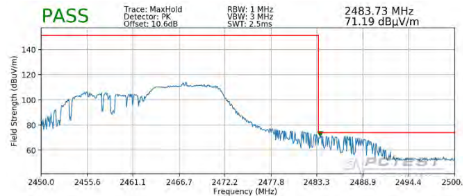
Plot 7-86. Radiated Restricted Upper Band Edge Measurement SISO ANT1 (Peak – 106 Tones)
