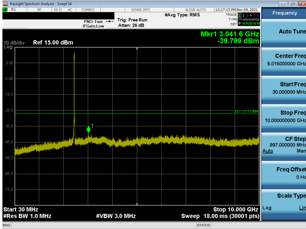
Plot 7-57. Conducted Spurious Plot SISO ANT2 (802.11ax OFDMA – 242 Tones – Ch. 11)
