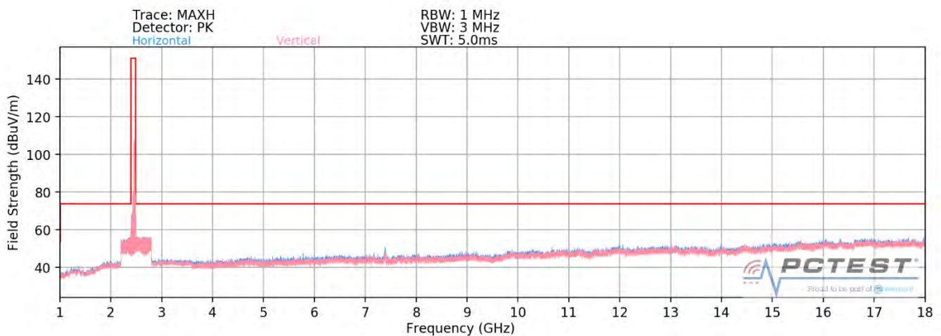
Plot 7-80. Radiated Spurious Plot above 1GHz MIMO (802.11ax OFDMA – 242 Tones – Ch. 11)
