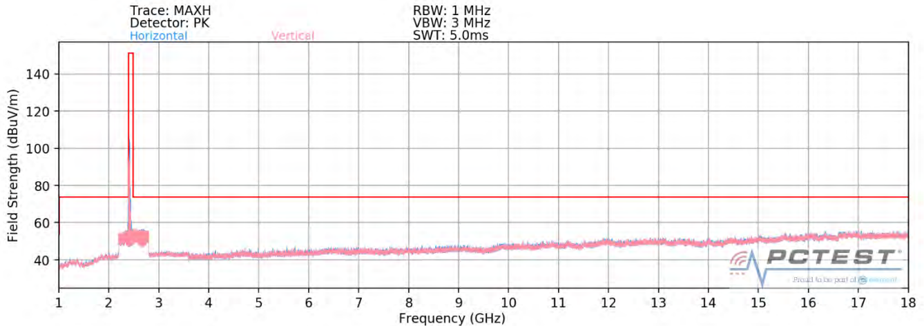
Plot 7-62. Radiated Spurious Plot above 1GHz SISO ANT1 (802.11ax OFDMA – 242 Tones – Ch. 1)
