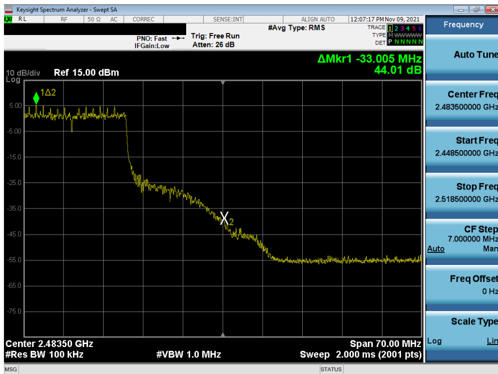
Plot 7-28. Band Edge Plot SISO ANT1 (802.11ax OFDMA – 242 Tones – Ch. 10)
