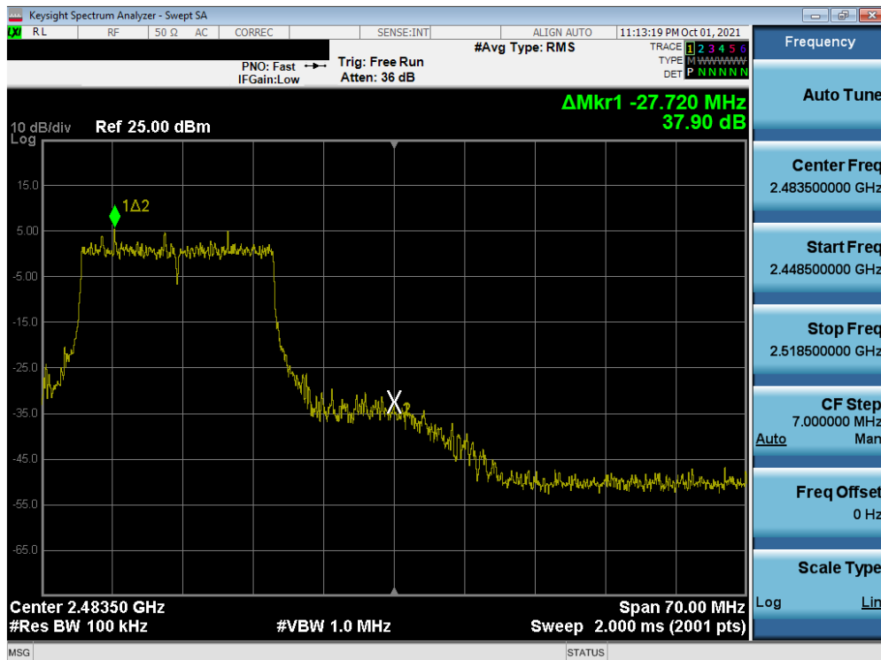
Plot 7-34. Band Edge Plot SISO ANT2 (802.11ax OFDMA – 242 Tones – Ch. 11)
