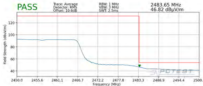
Plot 7-99. Radiated Restricted Upper Band Edge Measurement SISO ANT2 (Average – 242 Tones)
