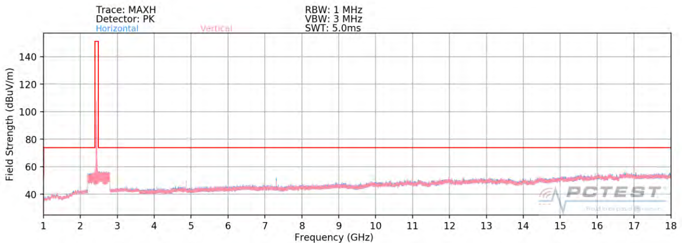
Plot 7-114. Radiated Spurious Plot above 1GHz MIMO/CDD (802.11g – Ch. 6)
