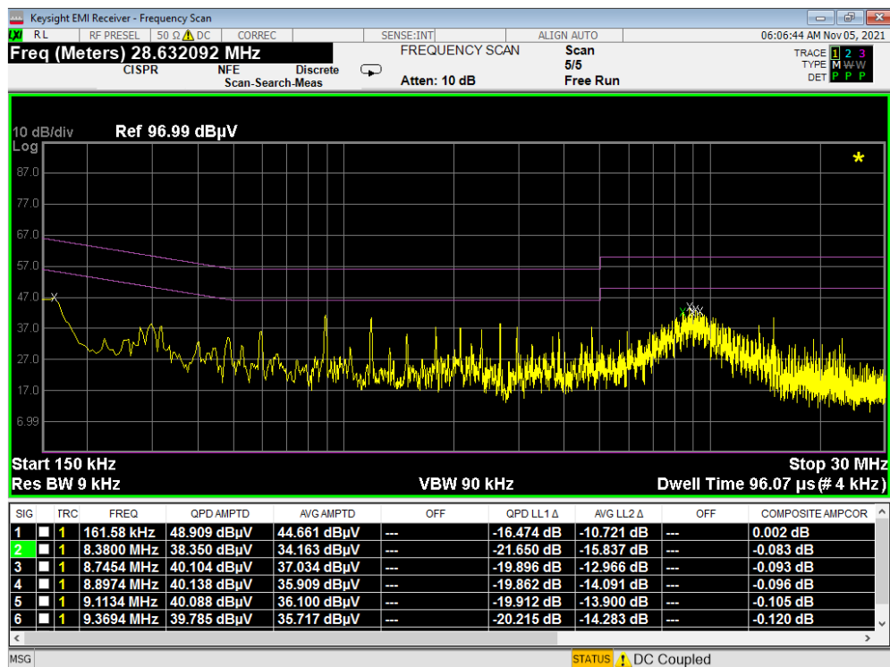
Plot 7-139. Line Conducted Plot with 802.11b (N) - WCP
