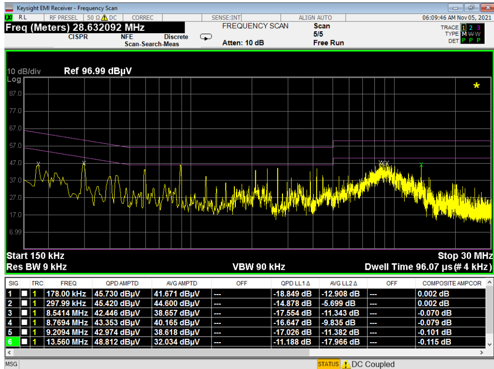
Plot 7-138. Line Conducted Plot with 802.11b (L1) - WCP
