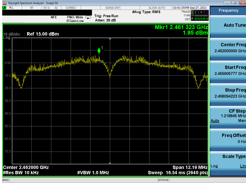
Plot 7-51. Power Spectral Density Plot MIMO ANT1 (802.11b (2.4GHz) – Ch. 11)
