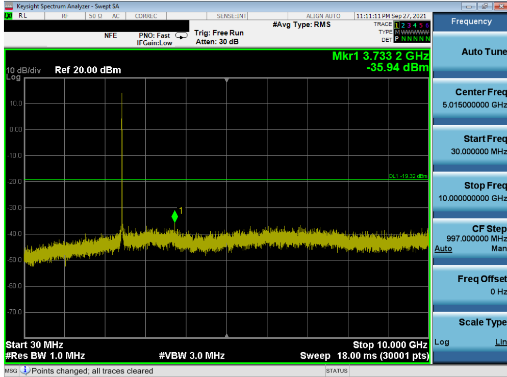
Plot 7-101. Conducted Spurious Plot SISO ANT2 (802.11b – Ch. 6)
