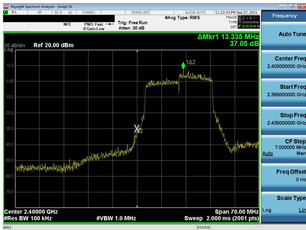
Plot 7-90. Band Edge Plot SISO ANT2 (802.11ax (2.4GHz) – Ch. 1)
