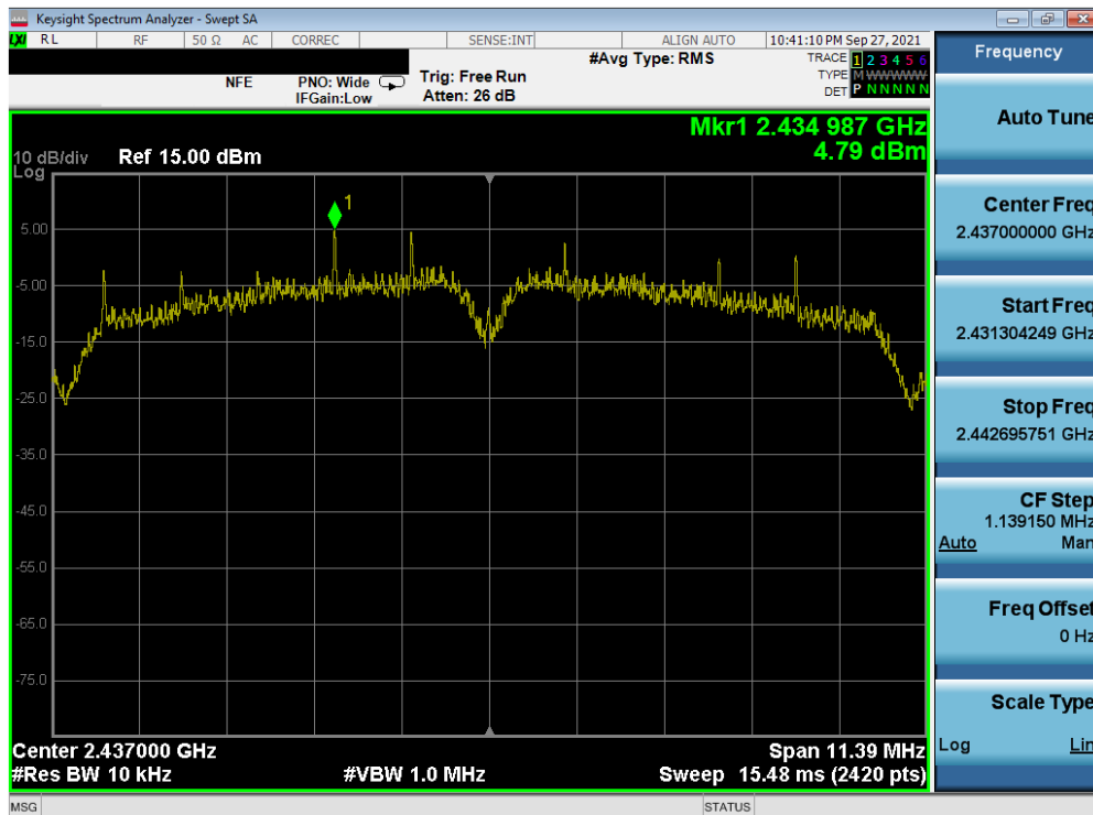
Plot 7-50. Power Spectral Density Plot MIMO ANT1 (802.11b (2.4GHz) – Ch. 6)
