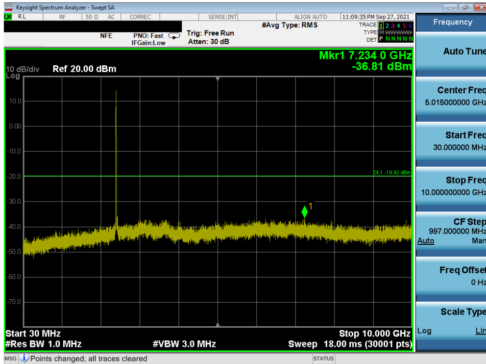
Plot 7-99. Conducted Spurious Plot SISO ANT2 (802.11b – Ch. 1)
