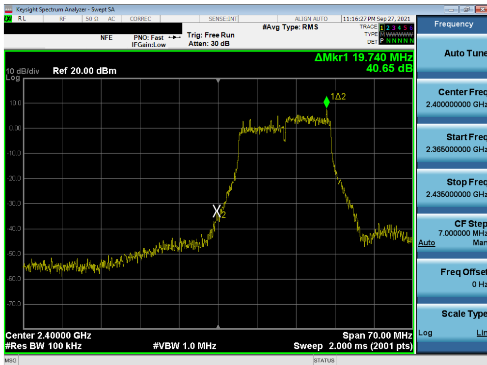
Plot 7-85. Band Edge Plot SISO ANT2 (802.11g- Ch. 1)
