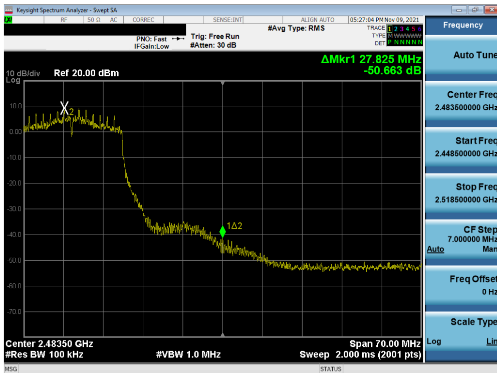
Plot 7-88. Band Edge Plot SISO ANT2 (802.11n (2.4GHz) – Ch. 10)
