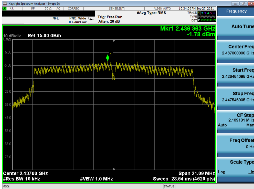
Plot 7-65. Power Spectral Density Plot MIMO ANT2 (802.11g) (2.4GHz) – Ch. 6)
