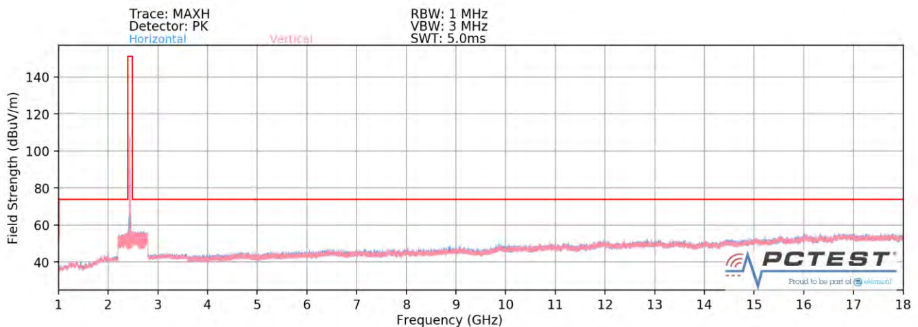
Plot 7-106. Radiated Spurious Plot above 1GHz SISO ANT1 (802.11b – Ch. 6)
