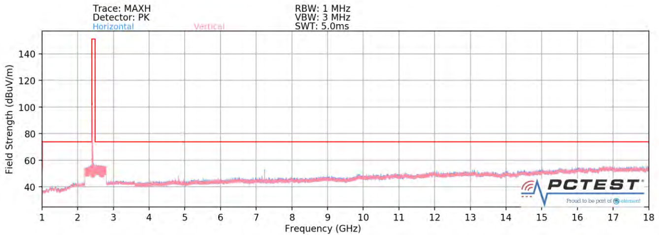
Plot 7-109. Radiated Spurious Plot above 1GHz SISO ANT2 (802.11b – Ch. 1)
