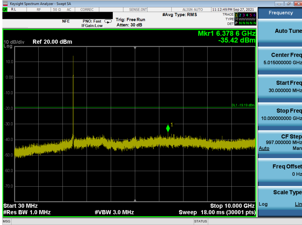
Plot 7-103. Conducted Spurious Plot SISO ANT2 (802.11b – Ch. 11)
