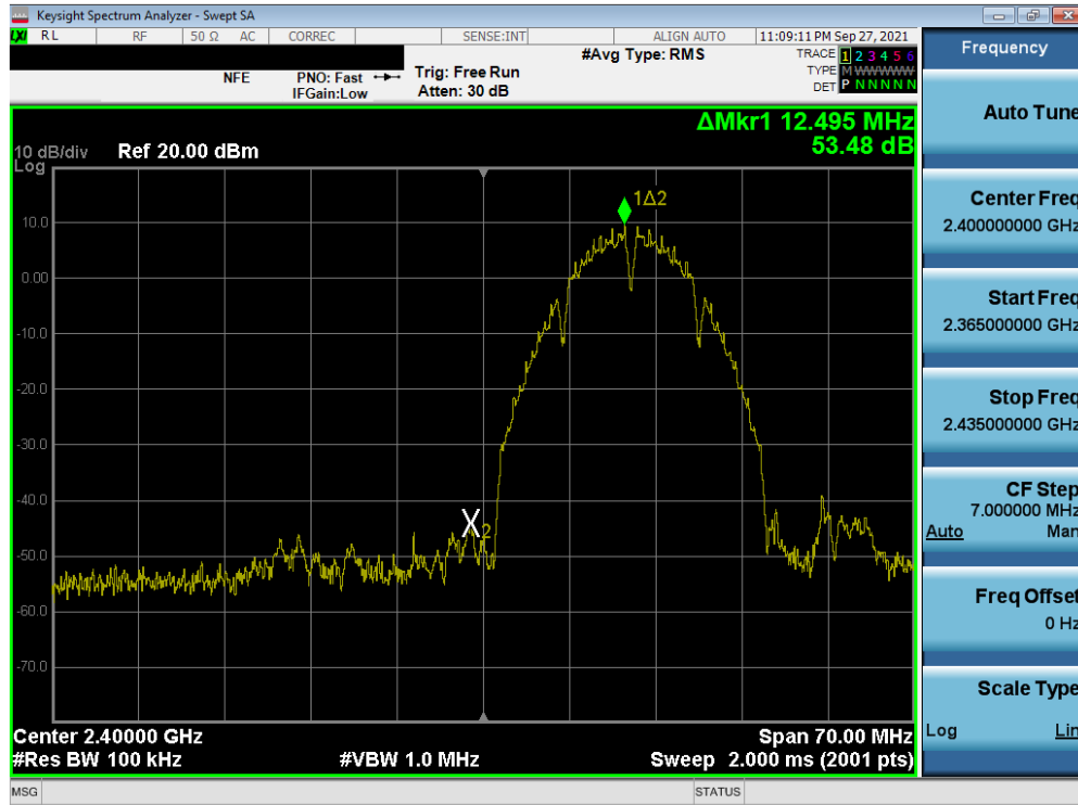
Plot 7-83. Band Edge Plot SISO ANT2 (802.11b – Ch. 1)
