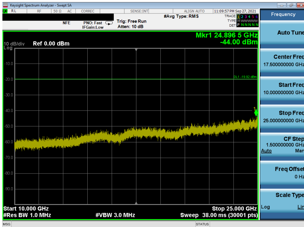
Plot 7-100. Conducted Spurious Plot SISO ANT2 (802.11b – Ch. 1)
