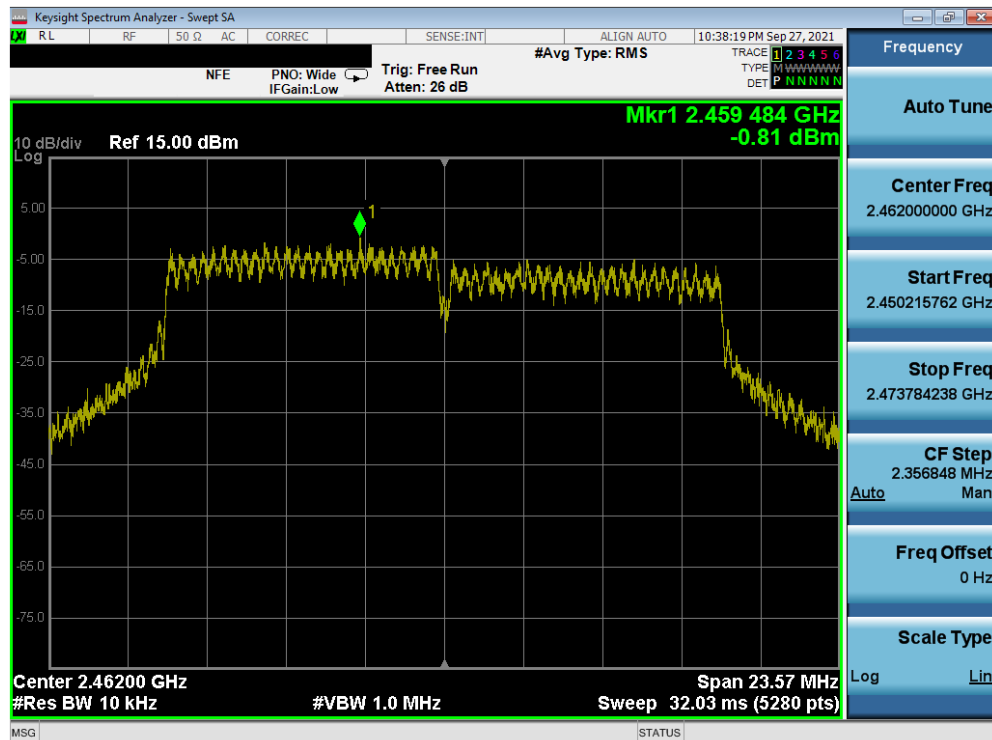
Plot 7-54. Power Spectral Density Plot MIMO ANT1 (802.11g) (2.4GHz) – Ch. 11)
