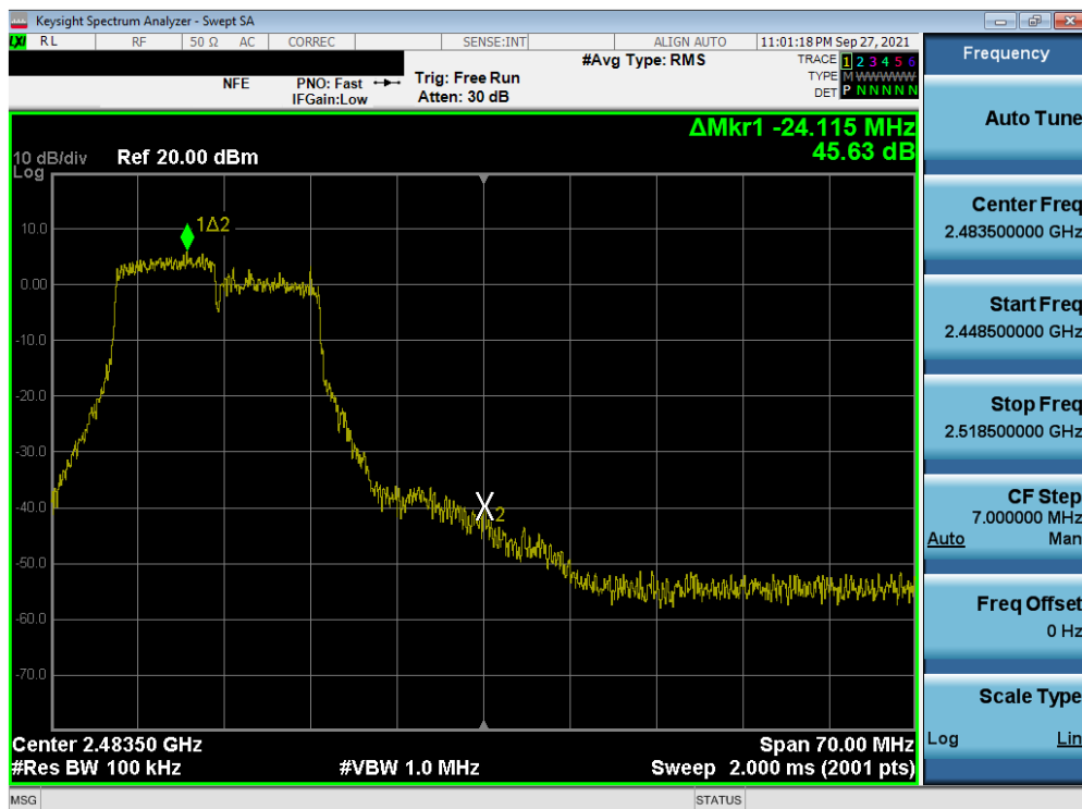
Plot 7-76. Band Edge Plot SISO ANT1 (802.11g - Ch. 11)
