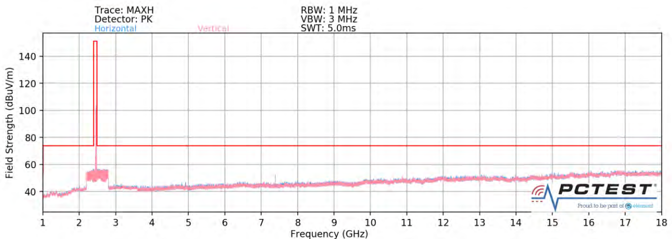
Plot 7-111. Radiated Spurious Plot above 1GHz SISO ANT2 (802.11b – Ch. 11)
