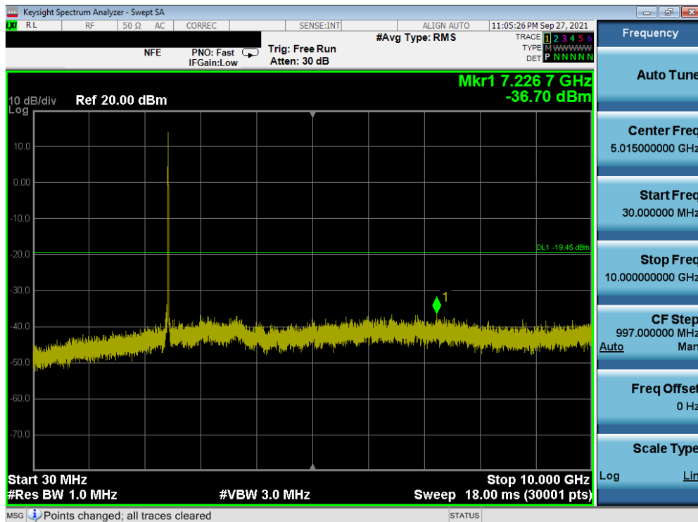
Plot 7-95. Conducted Spurious Plot SISO ANT1 (802.11b – Ch. 6)
