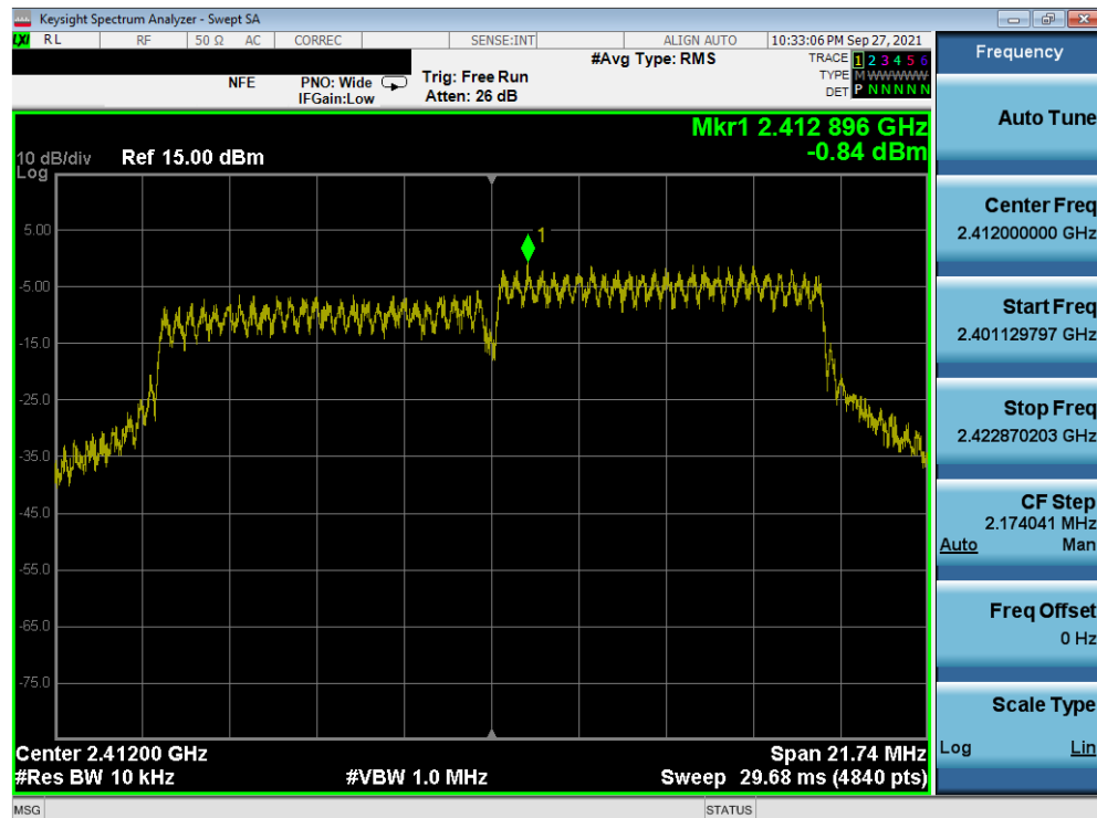
Plot 7-64. Power Spectral Density Plot MIMO ANT2 (802.11g) (2.4GHz) – Ch. 1)
