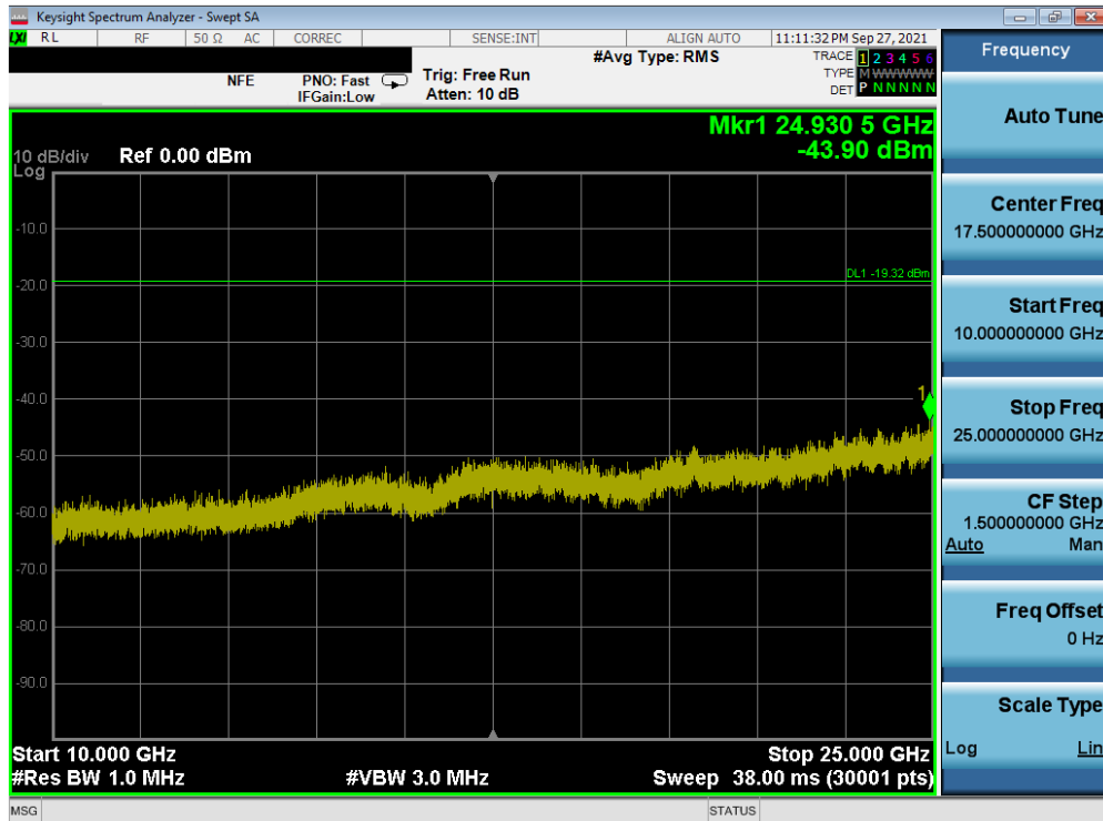
Plot 7-102. Conducted Spurious Plot SISO ANT2 (802.11b – Ch. 6)
