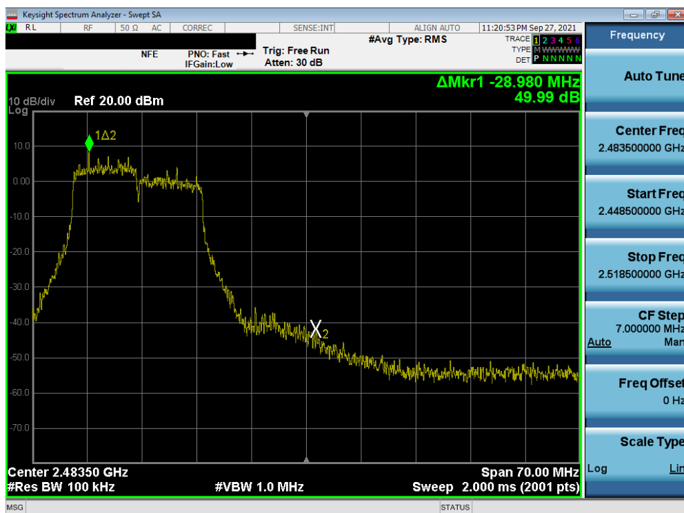
Plot 7-86. Band Edge Plot SISO ANT2 (802.11g - Ch. 11)
