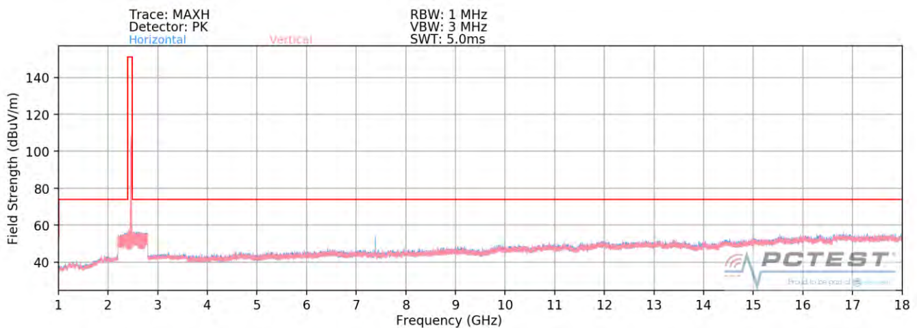
Plot 7-115. Radiated Spurious Plot above 1GHz MIMO/CDD (802.11g – Ch. 11)
