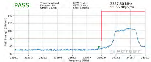
Plot 7-124. Radiated Restricted Lower Band Edge Measurement SISO ANT2 (Peak)
