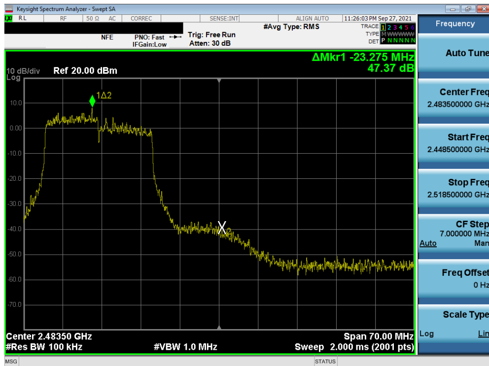
Plot 7-92. Band Edge Plot SISO ANT2 (802.11ax (2.4GHz) – Ch. 11)
