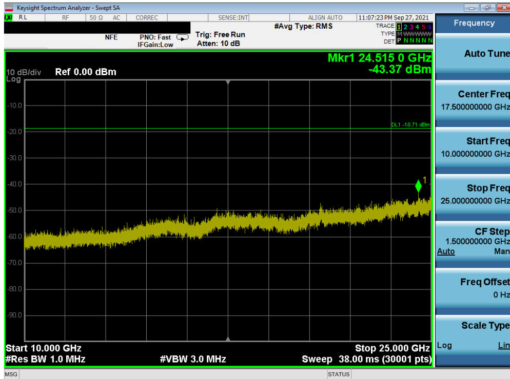
Plot 7-98. Conducted Spurious Plot SISO ANT1 (802.11b – Ch. 11)
