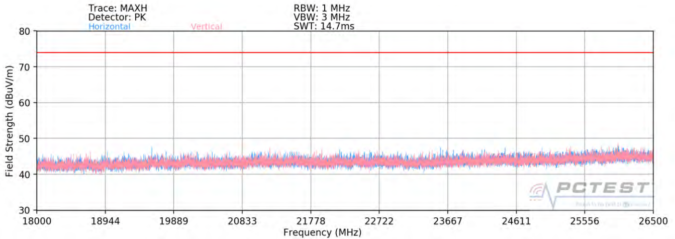
Plot 7-112. Radiated Spurious Plot above 18GHz SISO ANT2
