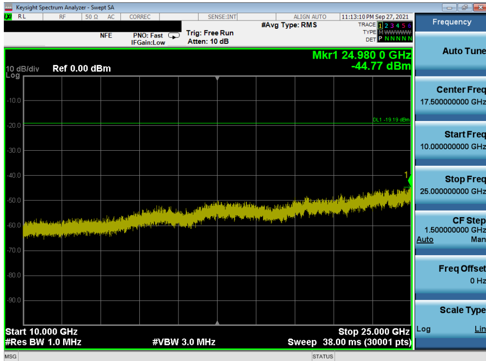
Plot 7-104. Conducted Spurious Plot SISO ANT2 (802.11b – Ch. 11)
