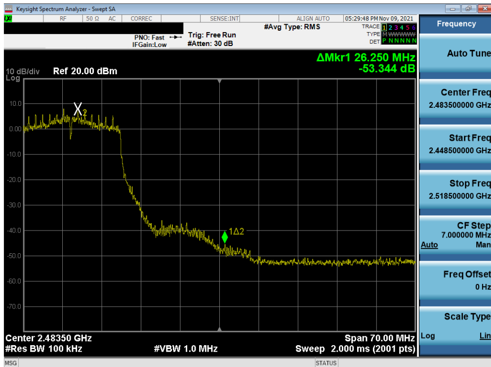
Plot 7-78. Band Edge Plot SISO ANT1 (802.11n (2.4GHz) – Ch. 10)
