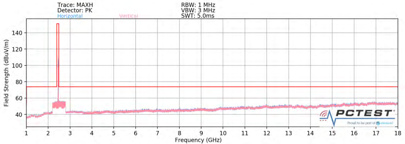
Plot 7-107. Radiated Spurious Plot above 1GHz SISO ANT1 (802.11b – Ch. 11)
