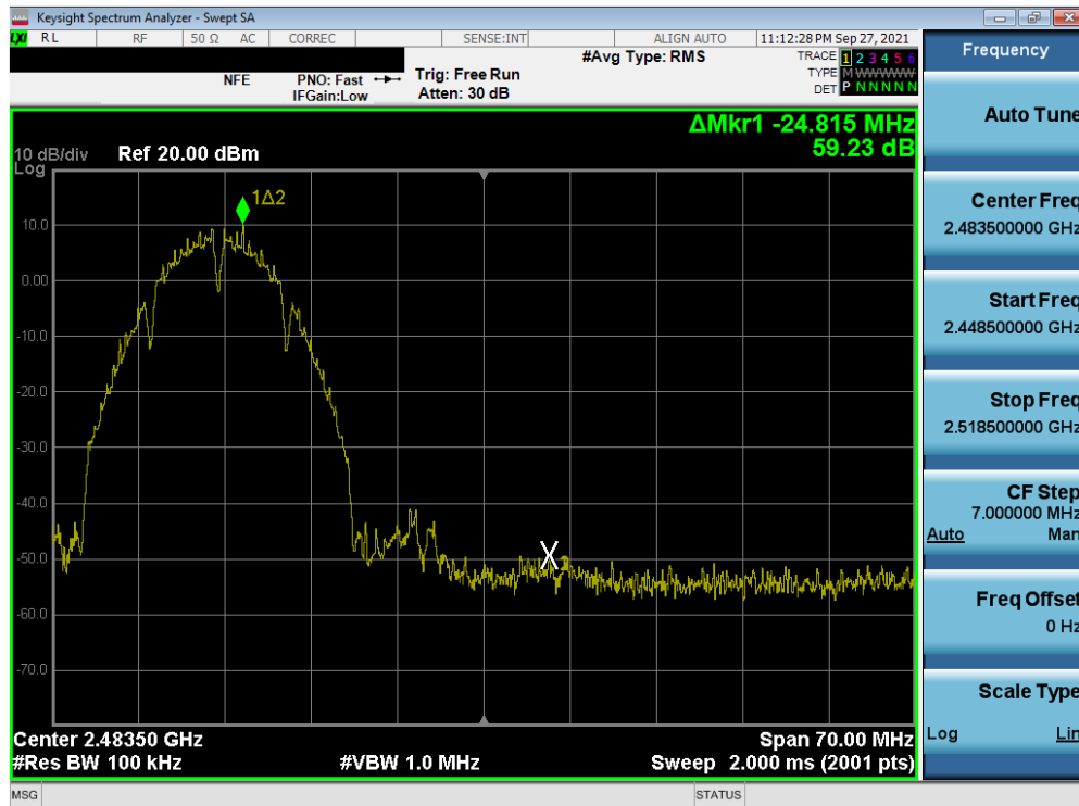
Plot 7-84. Band Edge Plot SISO ANT2 (802.11b – Ch. 11)
