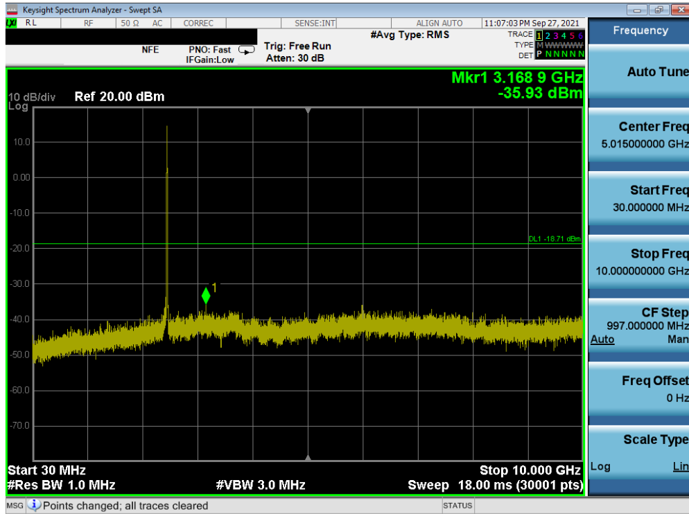
Plot 7-97. Conducted Spurious Plot SISO ANT1 (802.11b – Ch. 11)
