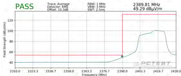
Plot 7-117. Radiated Restricted Lower Band Edge Measurement SISO ANT1 (Average)
