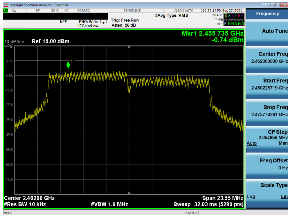
Plot 7-66. Power Spectral Density Plot MIMO ANT2 (802.11g) (2.4GHz) – Ch. 11)
