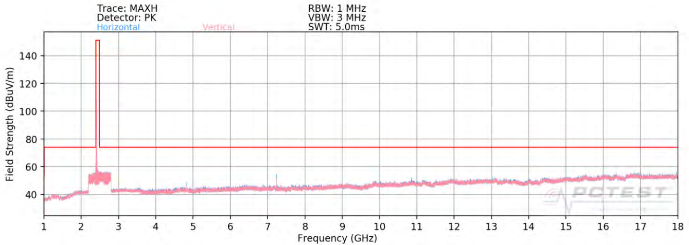
Plot 7-113. Radiated Spurious Plot above 1GHz MIMO/CDD (802.11g – Ch. 1)
