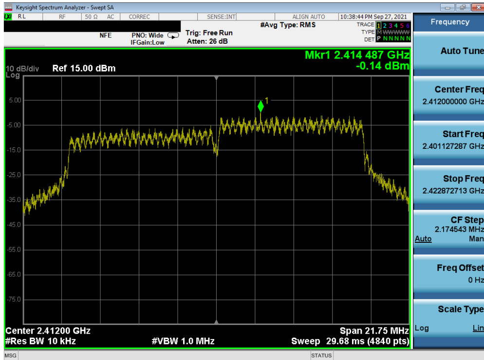
Plot 7-52. Power Spectral Density Plot MIMO ANT1 (802.11g (2.4GHz) – Ch. 1)
