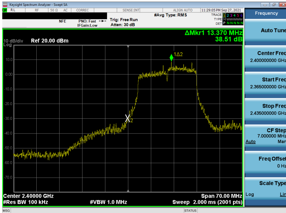
Plot 7-87. Band Edge Plot SISO ANT2 (802.11n (2.4GHz) – Ch. 1)
