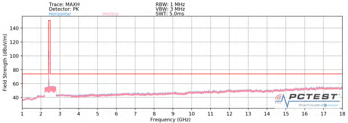
Plot 7-105. Radiated Spurious Plot above 1GHz SISO ANT1 (802.11b – Ch. 1)
