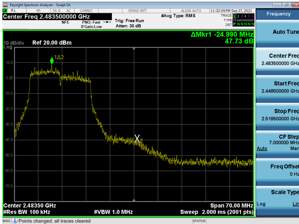
Plot 7-89. Band Edge Plot SISO ANT2 (802.11n (2.4GHz) – Ch. 11)
