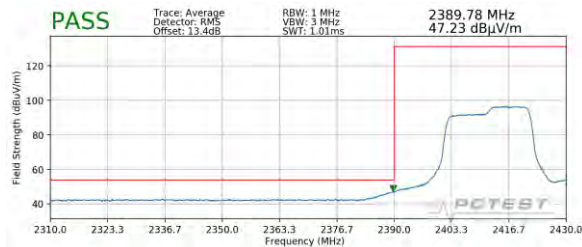
Plot 7-123. Radiated Restricted Lower Band Edge Measurement SISO ANT2 (Average)
