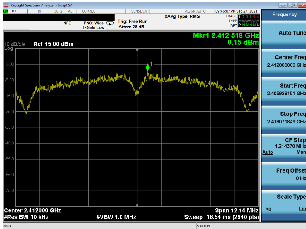
Plot 7-61. Power Spectral Density Plot MIMO ANT2 (802.11b (2.4GHz) – Ch. 1)
