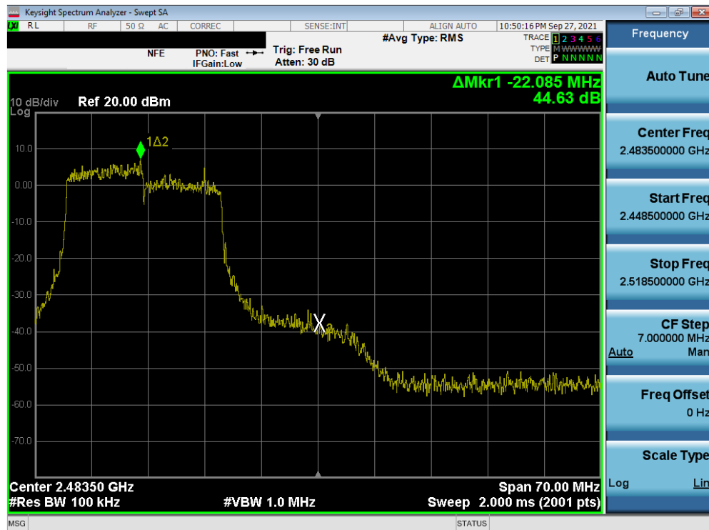
Plot 7-82. Band Edge Plot SISO ANT1 (802.11ax (2.4GHz) – Ch. 11)
