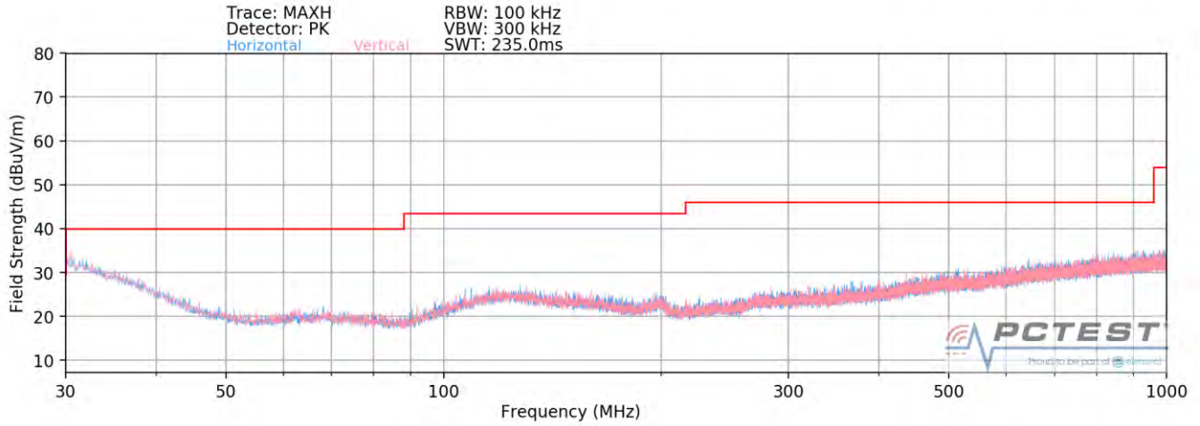
Plot 7-135. Radiated Spurious Plot below 1GHz MIMO
