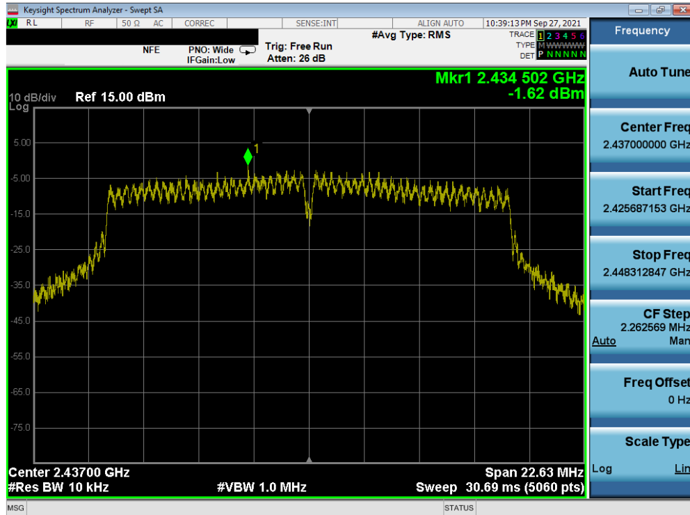
Plot 7-53. Power Spectral Density Plot MIMO ANT1 (802.11g) (2.4GHz) – Ch. 6)
