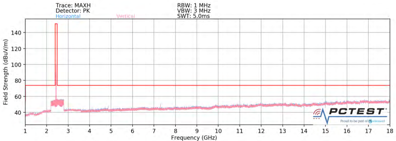
Plot 7-110. Radiated Spurious Plot above 1GHz SISO ANT2 (802.11b – Ch. 6)
