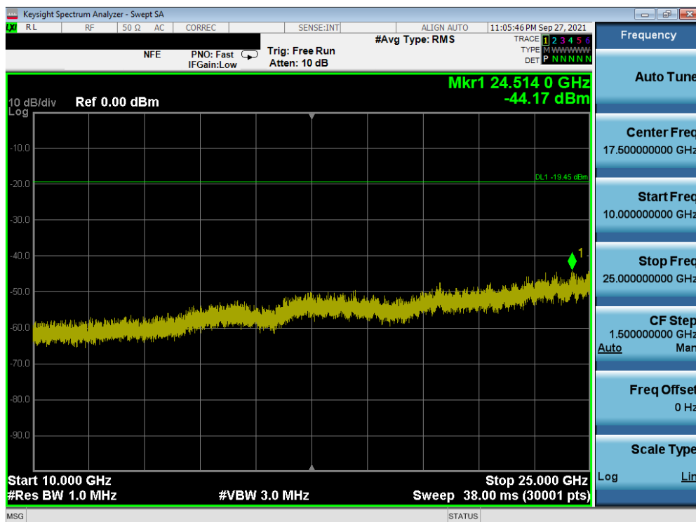
Plot 7-96. Conducted Spurious Plot SISO ANT1 (802.11b – Ch. 6)
