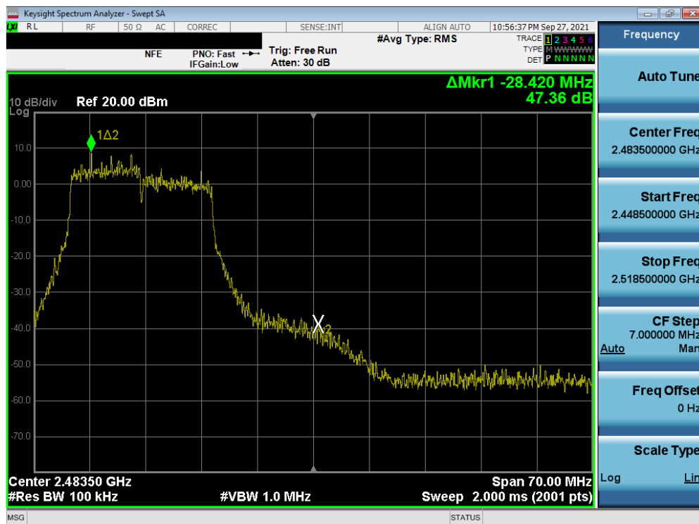
Plot 7-79. Band Edge Plot SISO ANT1 (802.11n (2.4GHz) – Ch. 11)
