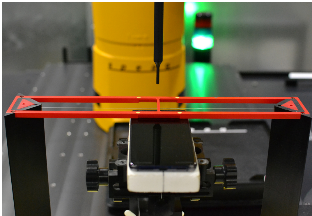
Figure 17-1 Ear Reference Point HAC Phantom Alignment
