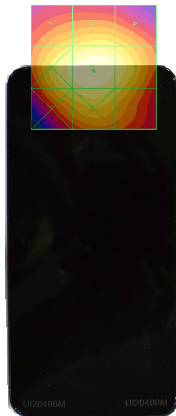
Figure 17-4 E-Field WD Scan overlay
