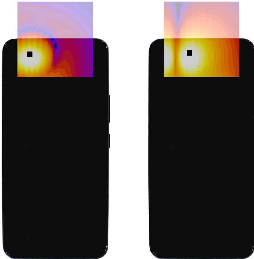
Figure 17-3 T-Coil Scan Overlay Magnetic Field Distributions
