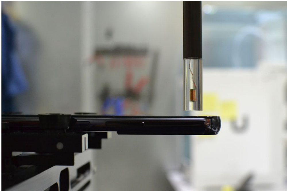
Figure 17-2 Test Setup for Wireless Device
