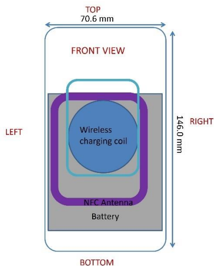
Figure E-2 NFC Antenna Locations
