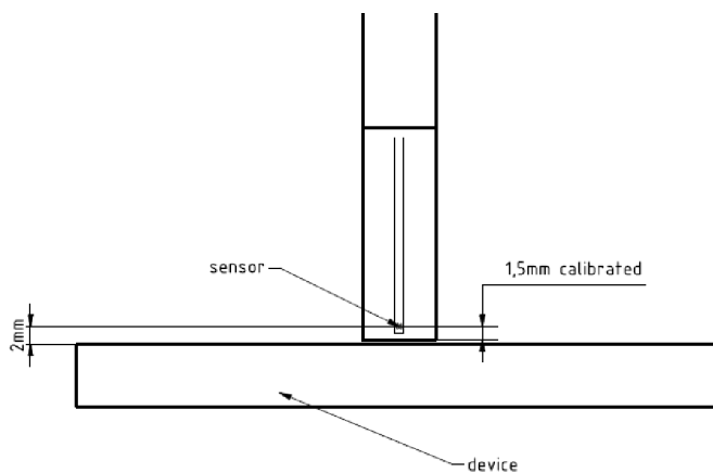
Figure D-2 EUMmWVx Probe
