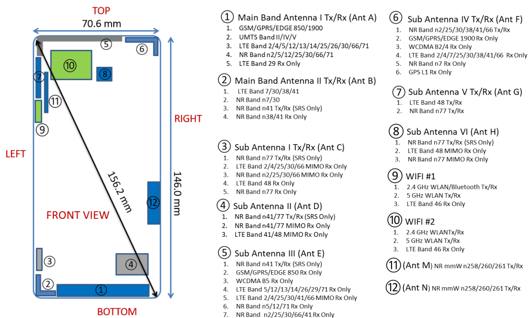
Figure D-1 DUT Antenna Locations
