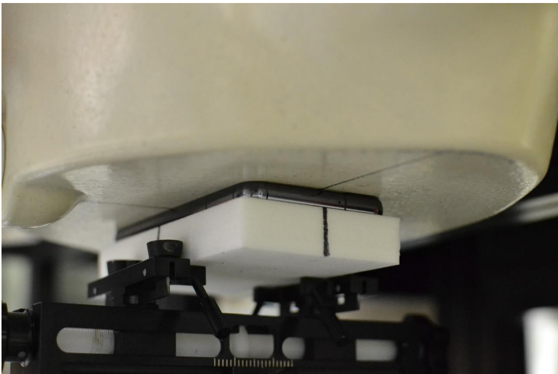
Test Setup Photo 14 – Body, Back Side at 0mm
