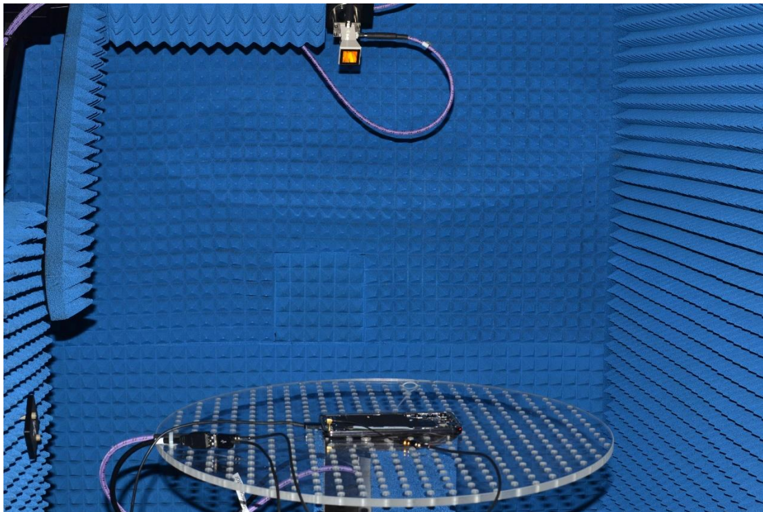
Test Setup Photo 7 – Radiated Power Measurement Setup (Figure 7-1)
