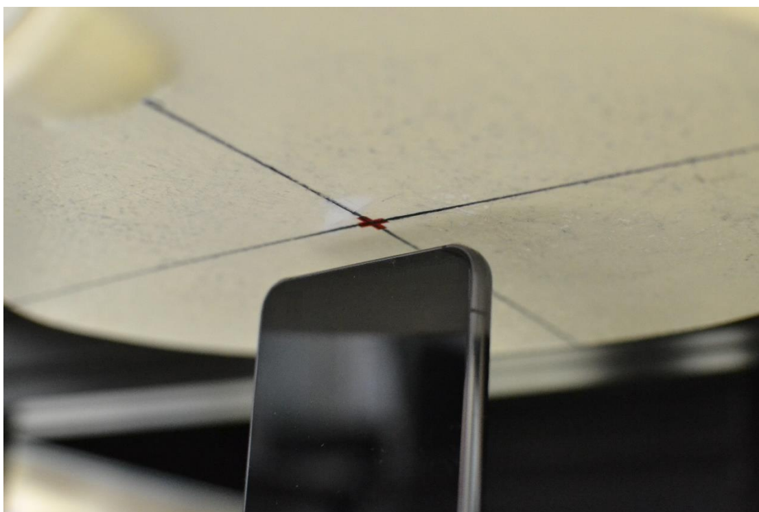
Test Setup Photo 12 – Body, Bottom Edge at 10 mm
