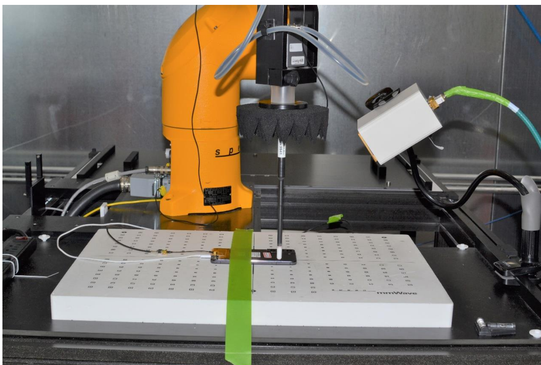
Test Setup Photo 8 – Power Density Setup Back Side (Figure 7-2)
