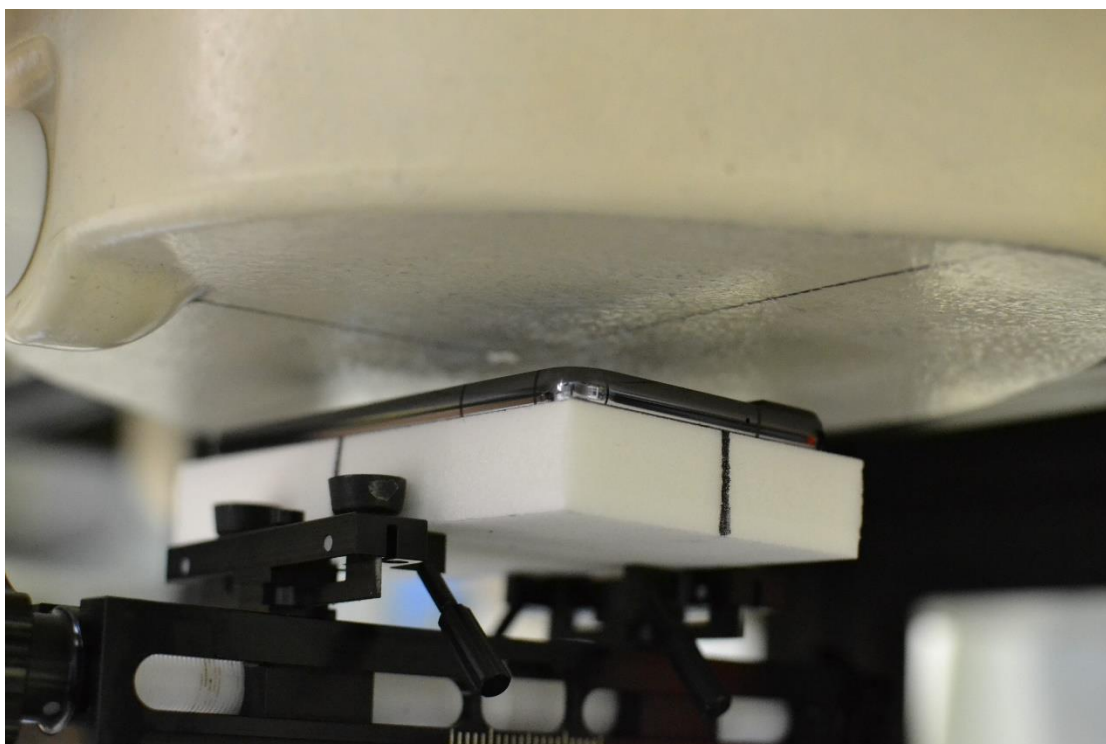
Test Setup Photo 10 – Body, Back Side at 15mm
