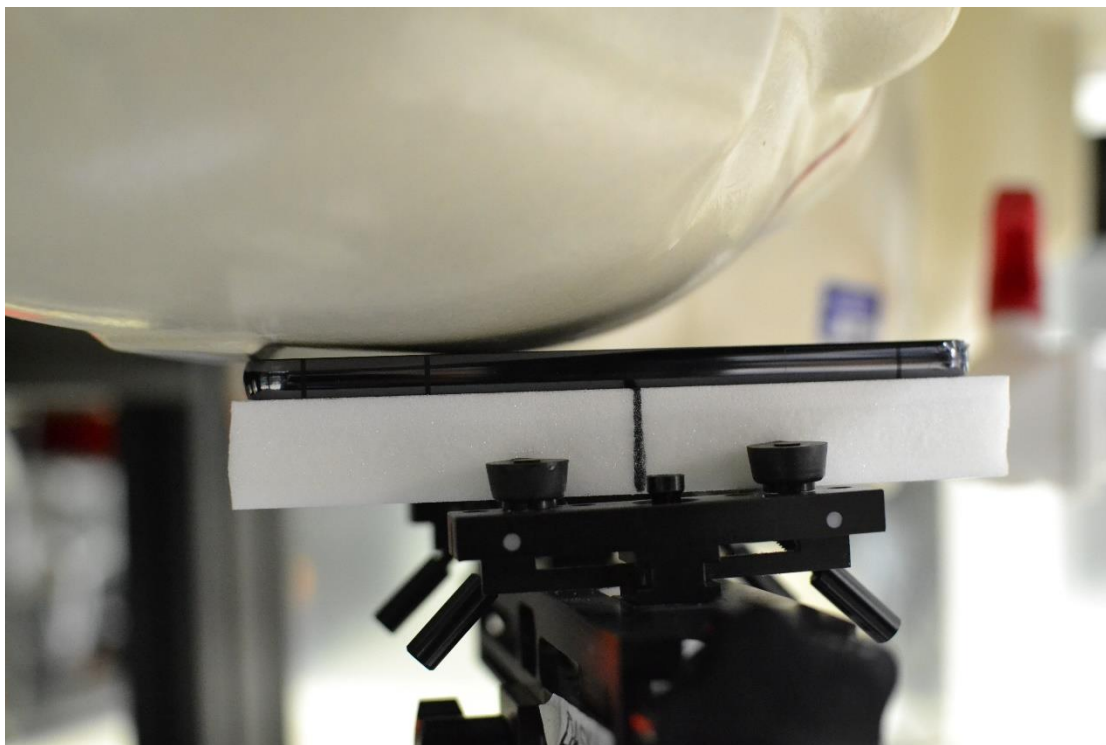
Test Setup Photo 9 – Right Head, Cheek
