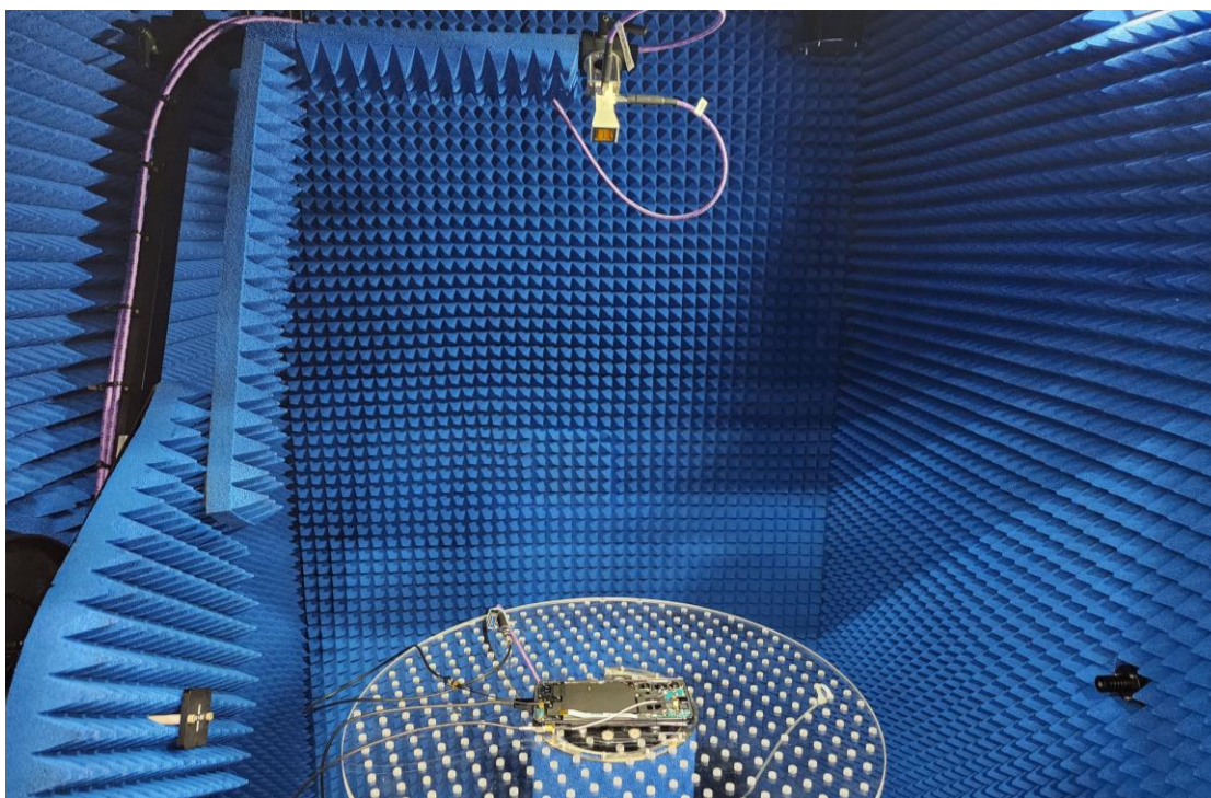
Test Setup Photo 16 – sub6 NR + mmW Power Measurement Setup (Figure 7-2)
