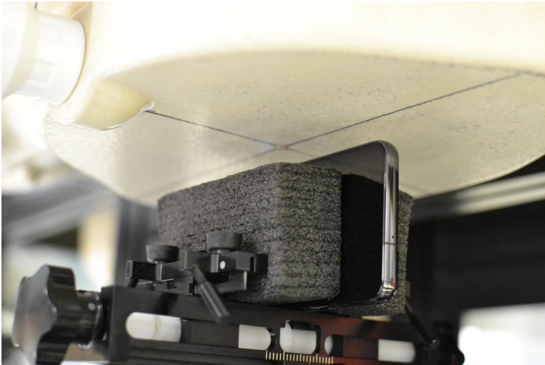
Test Setup Photo 13 – Body, Left Edge at 10 mm
