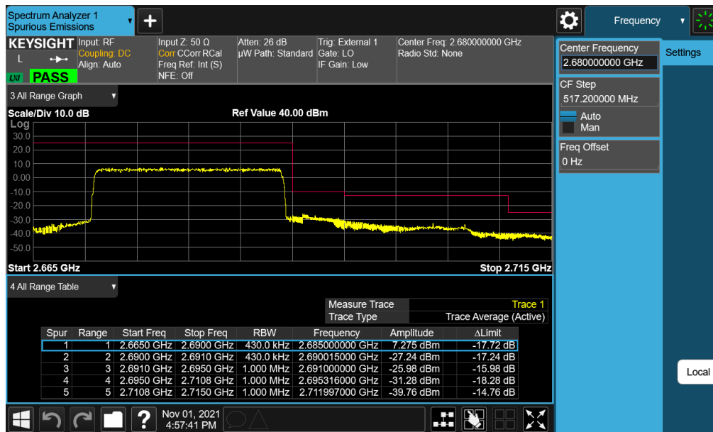
Plot 7-19. Upper ACP Plot (LTE Band 41(PC2) - 20MHz QPSK - Full RB)
