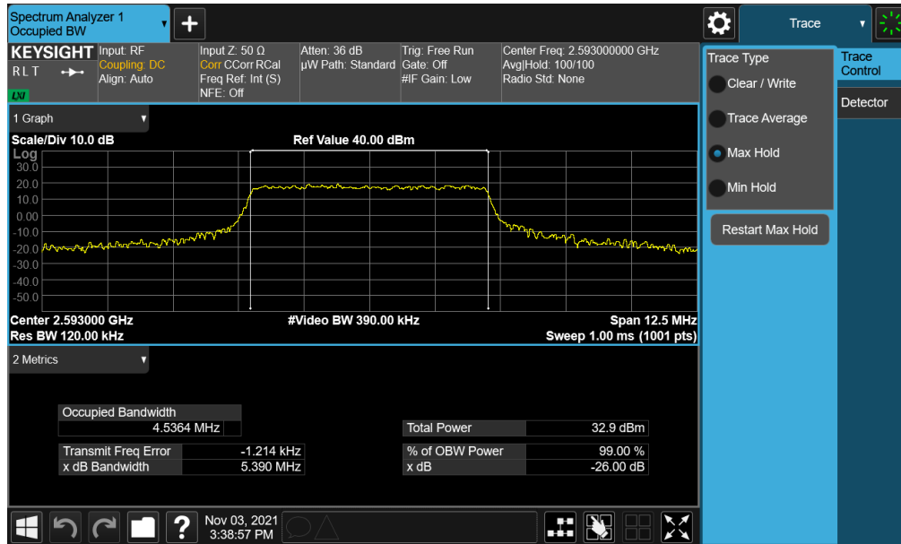
Plot 7-7. Occupied Bandwidth Plot (LTE Band 41(PCI) - 5MHz QPSK - Full RB)
