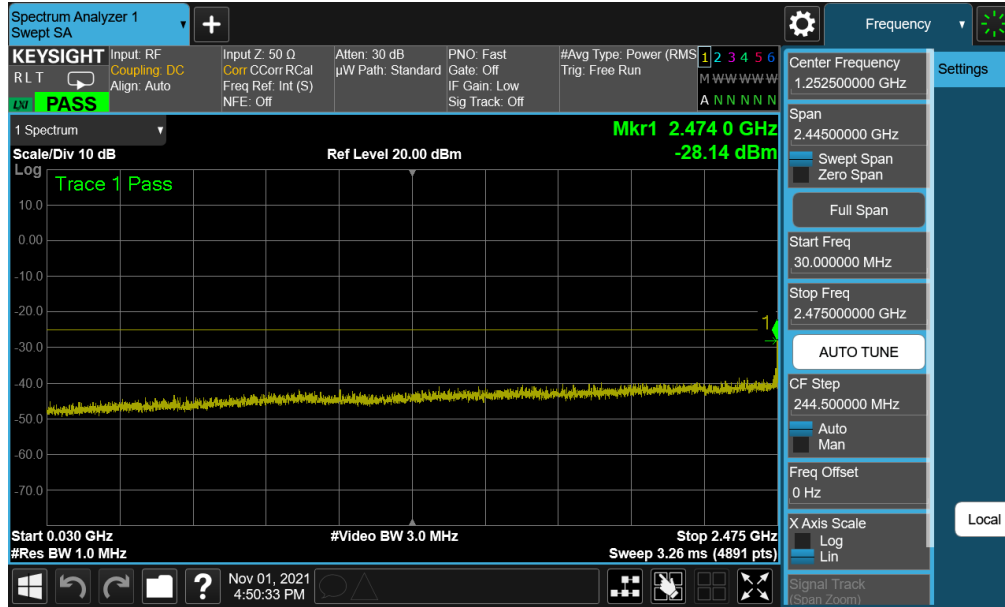
Plot 7-9. Conducted Spurious Plot (LTE Band 41(PC2) - 20MHz QPSK - RB Size 1, RB Offset 0 - Low Channel)
