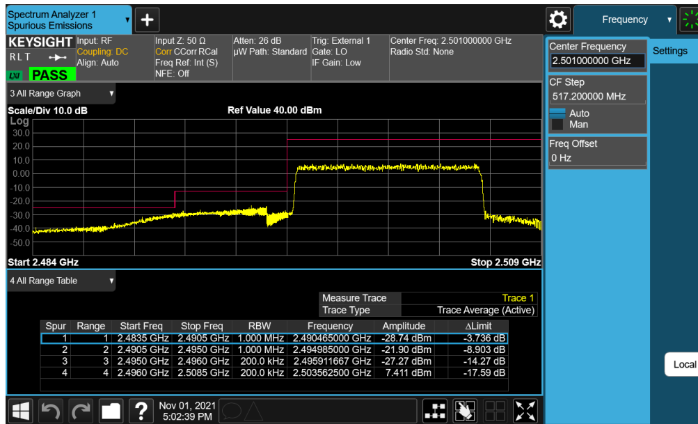
Plot 7-22. Lower ACP Plot (LTE Band 41(PC2) - 10MHz QPSK – Full RB)
