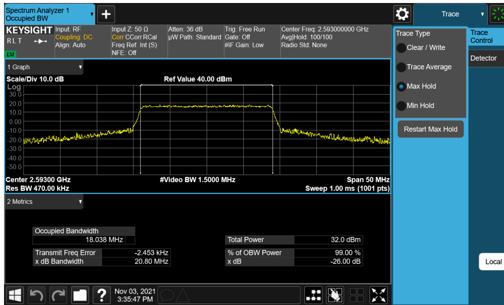
Plot 7-2. Occupied Bandwidth Plot (LTE Band 41(PC2) - 20MHz 16-QAM - Full RB)
