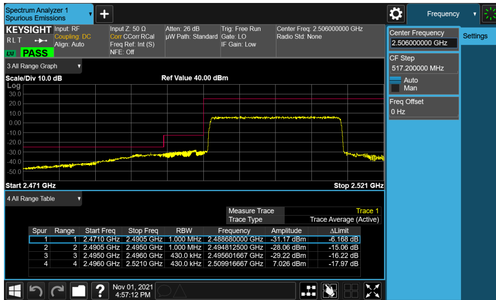
Plot 7-18. Lower ACP Plot (LTE Band 41(PC2) - 20MHz QPSK - Full RB)
