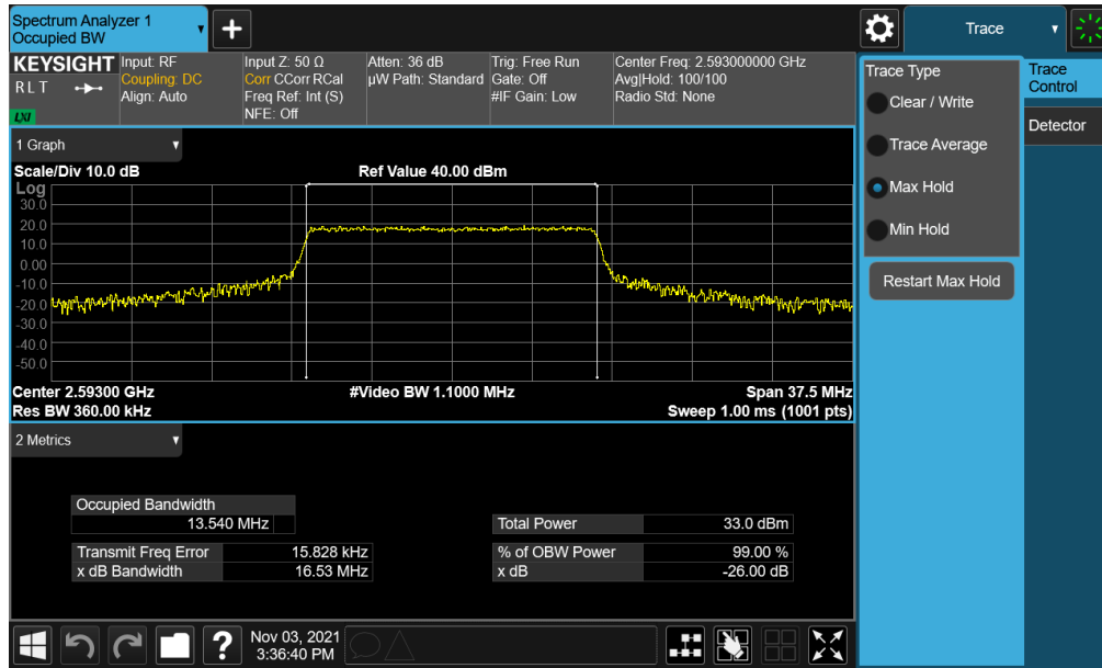
Plot 7-3. Occupied Bandwidth Plot (LTE Band 41(PC2) - 15MHz QPSK - Full RB)
