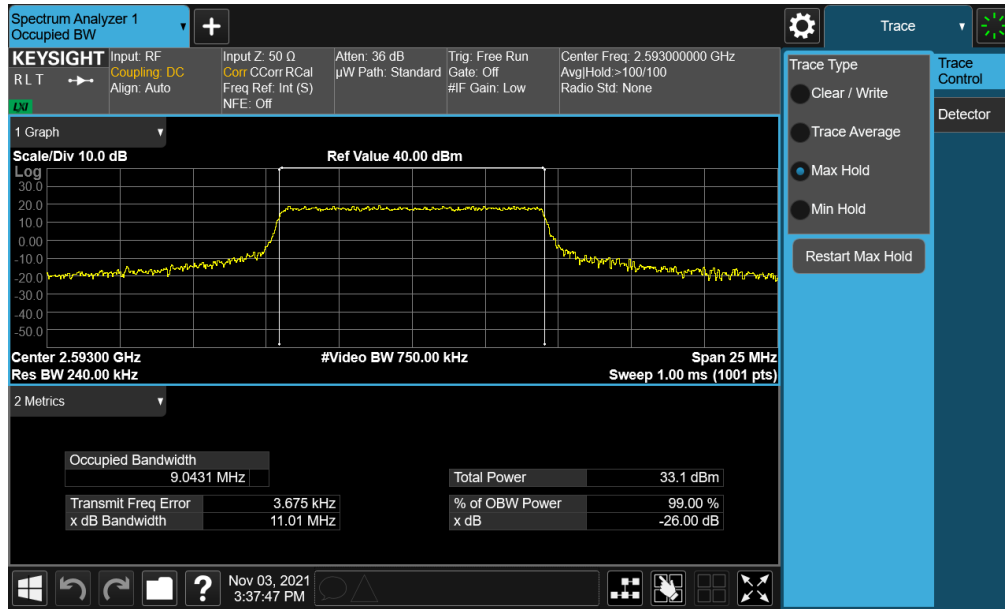
Plot 7-5. Occupied Bandwidth Plot (LTE Band 41(PC2) - 10MHz QPSK - Full RB)
