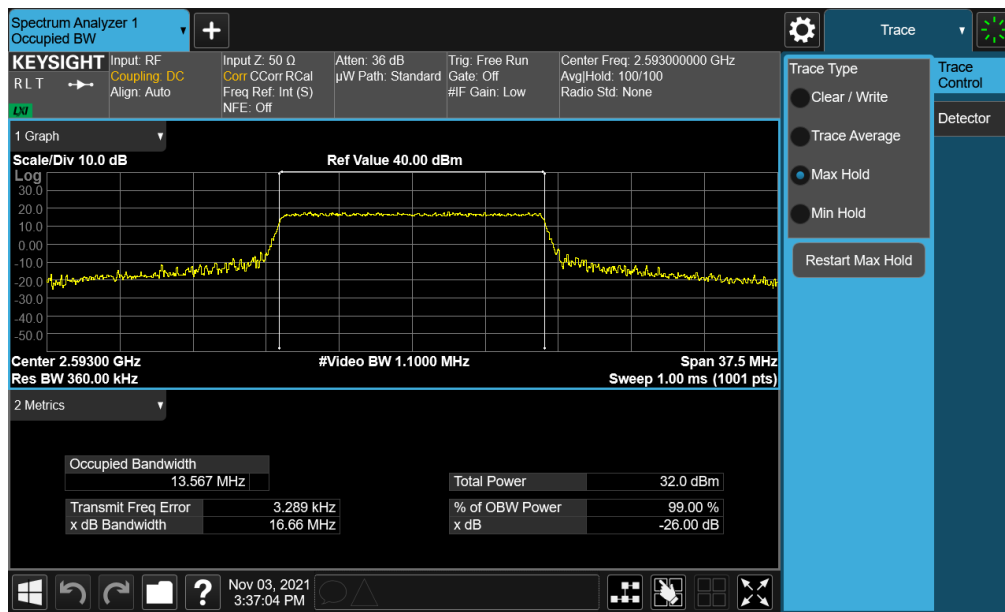
Plot 7-4. Occupied Bandwidth Plot (LTE Band 41(PC2) - 15MHz 16-QAM - Full RB)
