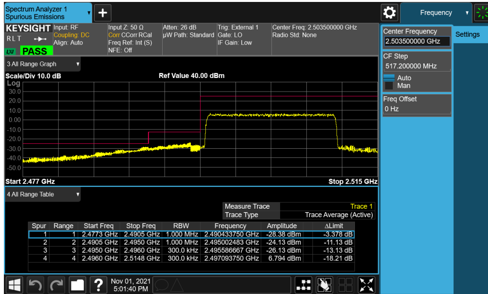
Plot 7-20. Lower ACP Plot (LTE Band 41(PC2) - 15MHz QPSK – Full RB)
