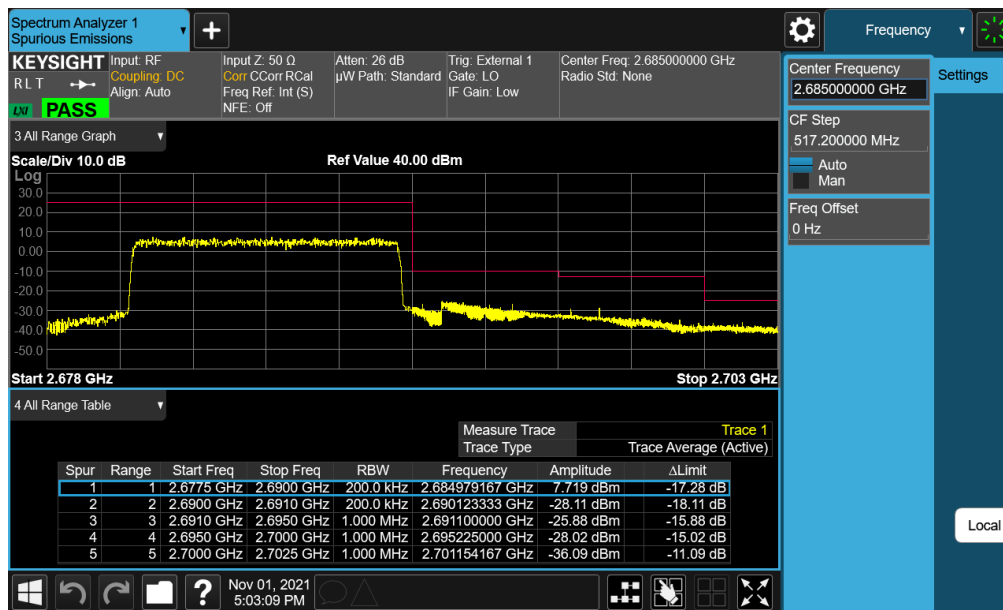
Plot 7-23. Upper ACP Plot (LTE Band 41(PC2) - 10MHz QPSK – Full RB)
