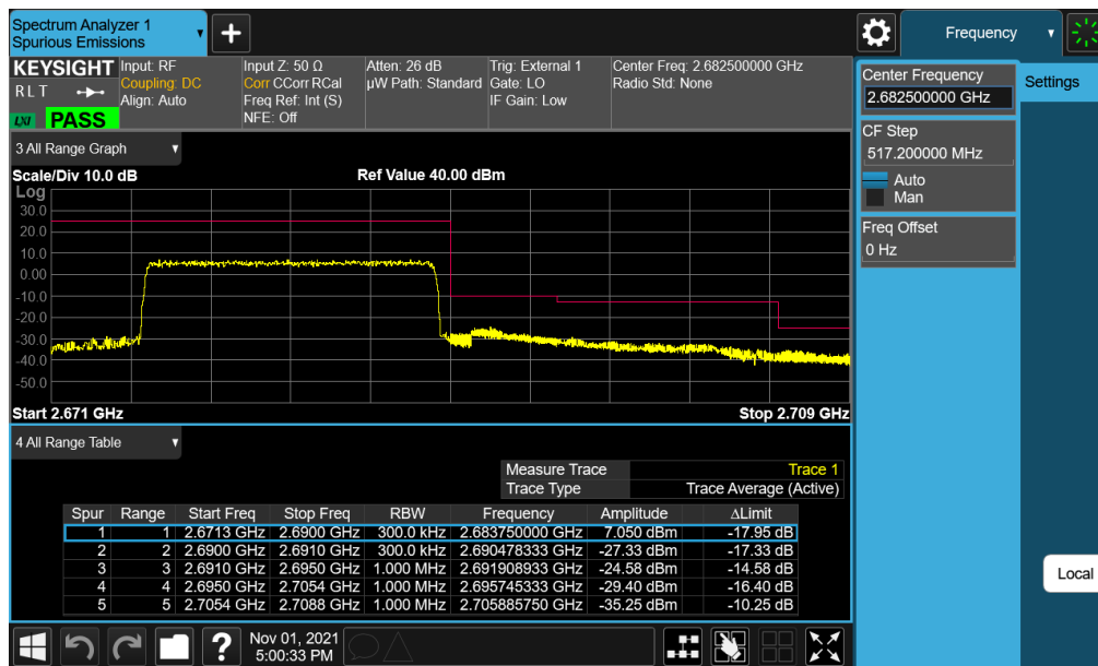
Plot 7-21. Upper ACP Plot (LTE Band 41(PC2) - 15MHz QPSK – Full RB)
