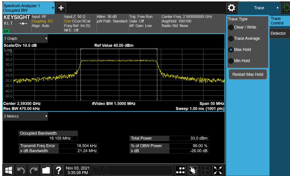
Plot 7-1. Occupied Bandwidth Plot (LTE Band 41(PC2) - 20MHz QPSK - Full RB)
