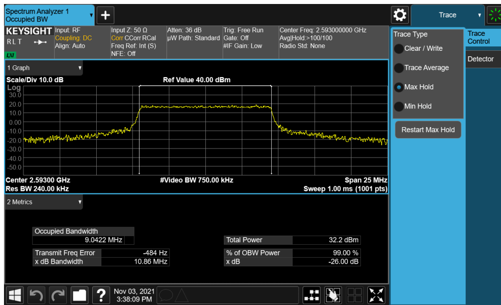
Plot 7-6. Occupied Bandwidth Plot (LTE Band 41(PC2) - 10MHz 16-QAM - Full RB)
