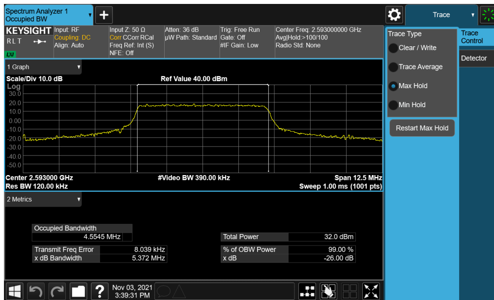
Plot 7-8. Occupied Bandwidth Plot (LTE Band 41(PCI) - 5MHz 16-QAM - Full RB)
