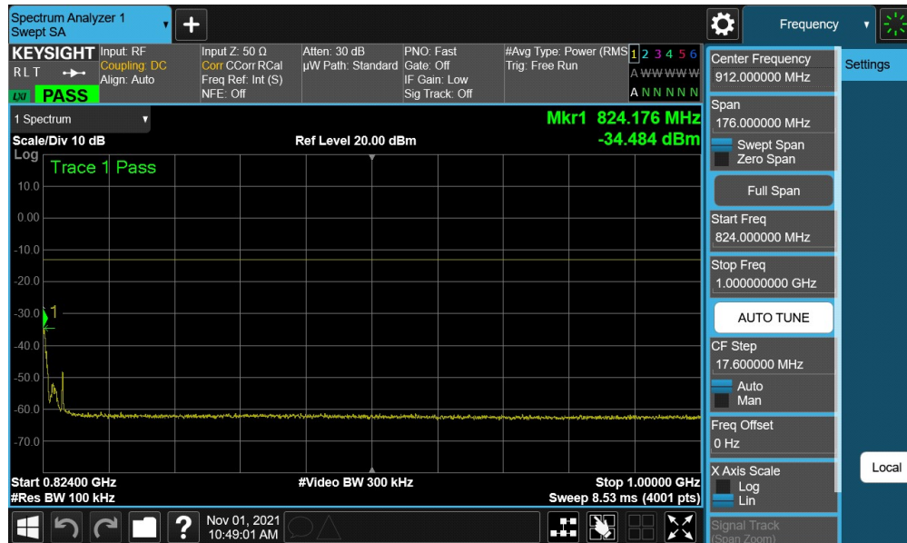
Plot 7-12. Conducted Spurious Plot (LTE Band 26 - 15MHz QPSK - RB Size 1, RB Offset 0)
