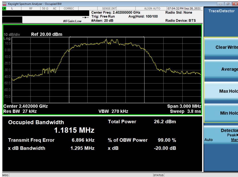
Plot 7-16. 20dB Bandwidth Plot (Bluetooth, 3Mbps – Ch. 0) Antenna 2
