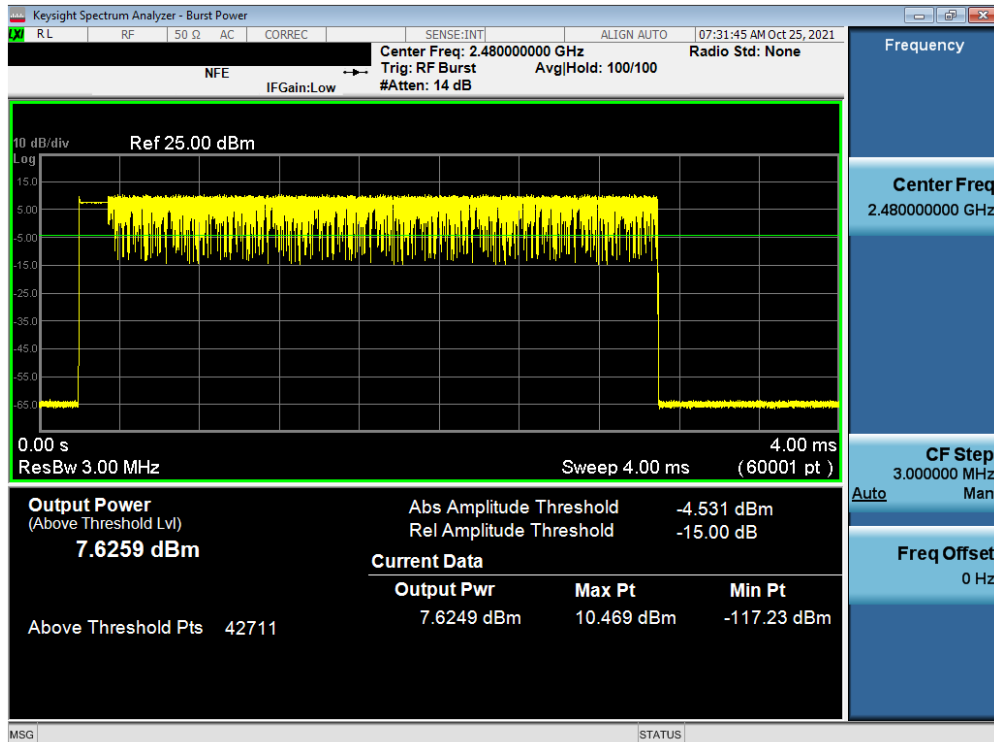
Plot 7-90. Average Conducted Power (3Mbps – Ch. 78) Antenna 2 iPA
