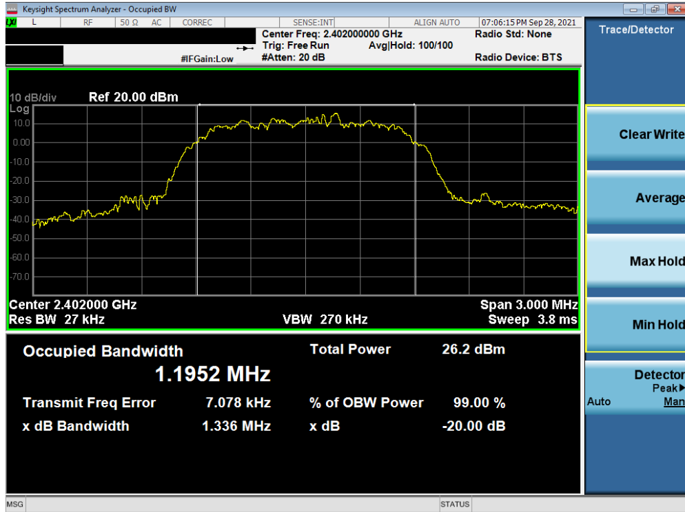
Plot 7-13. 20dB Bandwidth Plot (Bluetooth, 2Mbps – Ch. 0) Antenna 2
