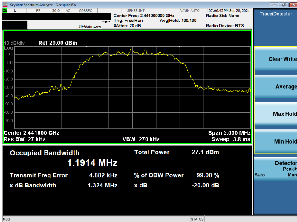
Plot 7-14. 20dB Bandwidth Plot (Bluetooth, 2Mbps – Ch. 39) Antenna 2
