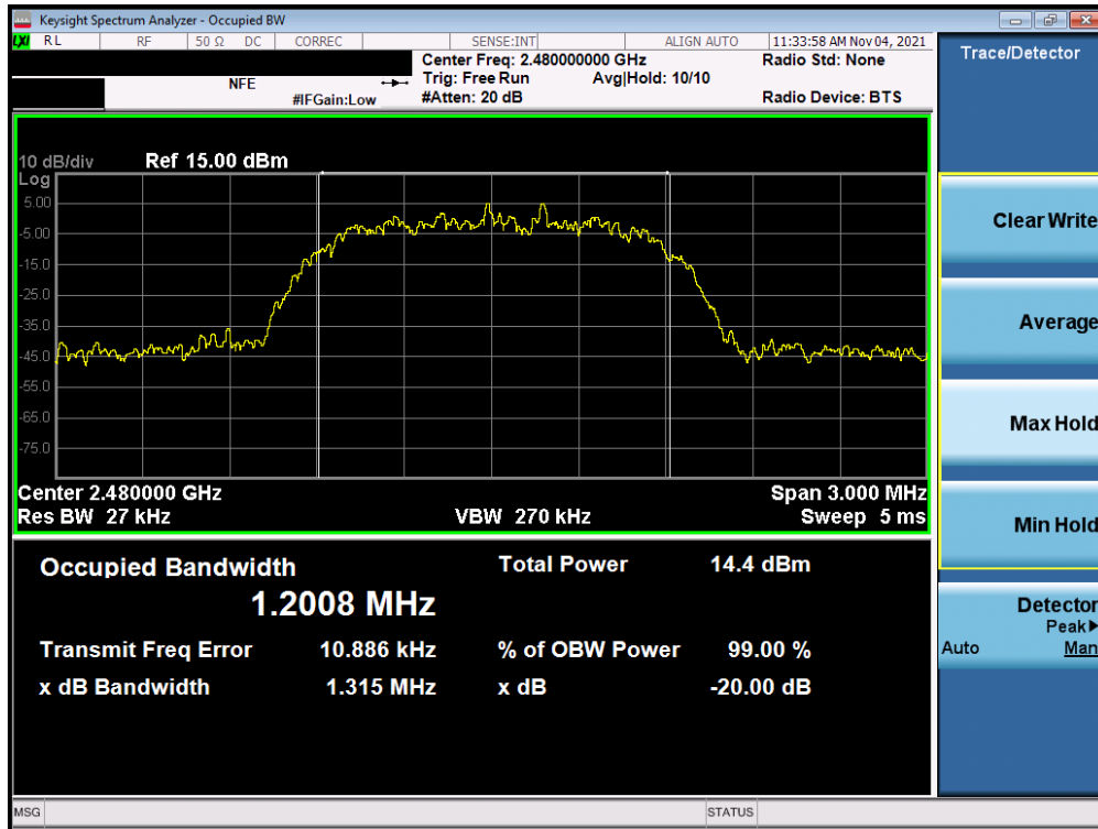
Plot 7-6. 20dB Bandwidth Plot (Bluetooth, 2Mbps – Ch. 78) Antenna 1
