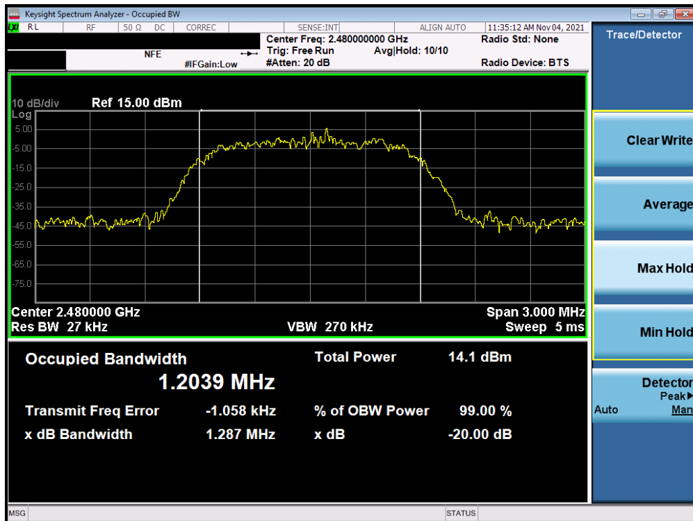
Plot 7-9. 20dB Bandwidth Plot (Bluetooth, 3Mbps – Ch. 78) Antenna 1
