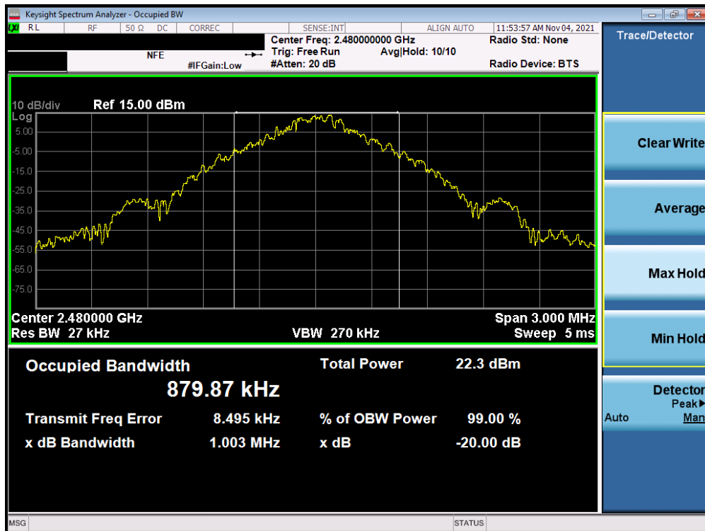
Plot 7-12. 20dB Bandwidth Plot (Bluetooth, 1Mbps – Ch. 78) Antenna 2
