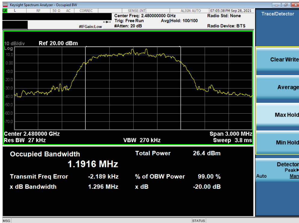
Plot 7-18. 20dB Bandwidth Plot (Bluetooth, 3Mbps – Ch. 78) Antenna 2
