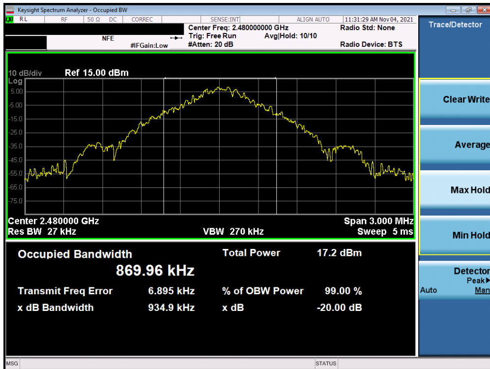
Plot 7-3. 20dB Bandwidth Plot (Bluetooth, 1Mbps – Ch. 78) Antenna 1
