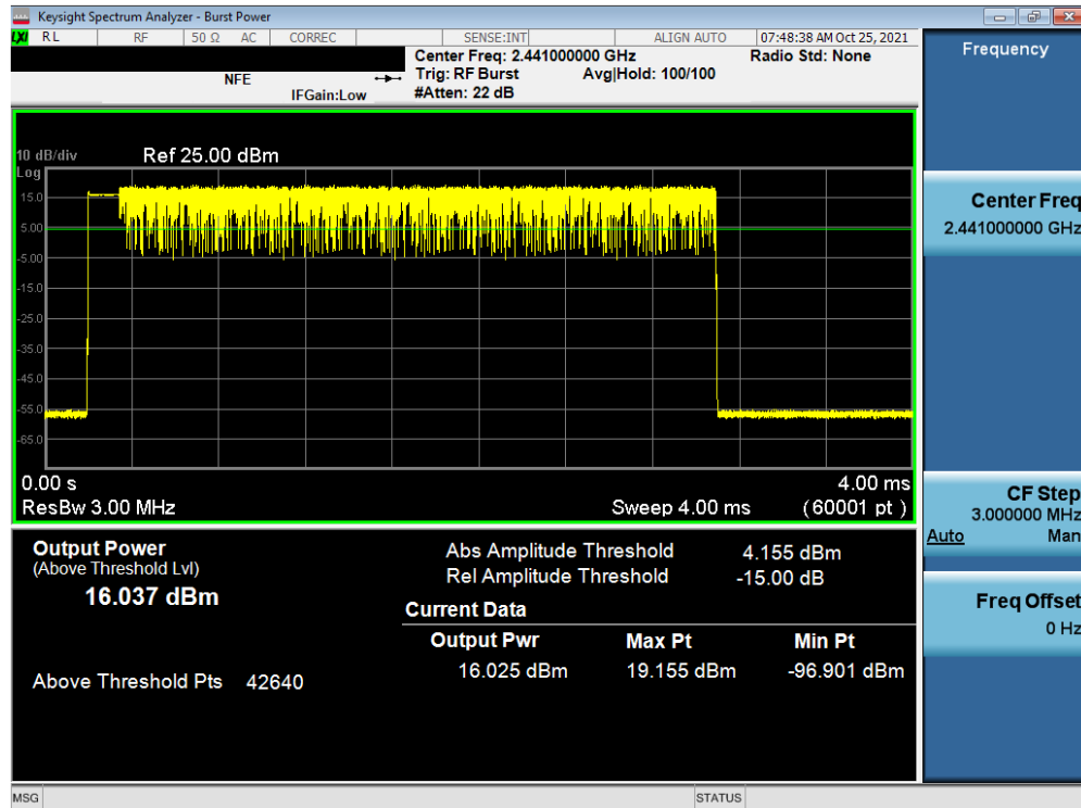
Plot 7-86. Average Conducted Power (3Mbps – Ch. 39) Antenna 2 ePA
