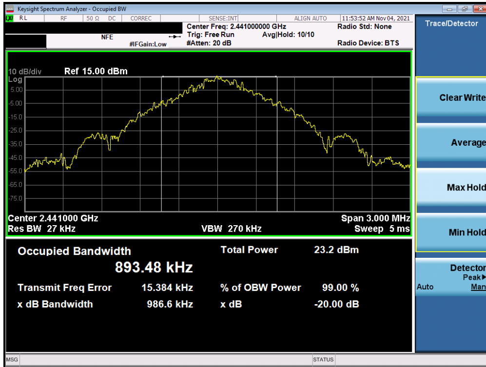
Plot 7-11. 20dB Bandwidth Plot (Bluetooth, 1Mbps – Ch. 39) Antenna 2
