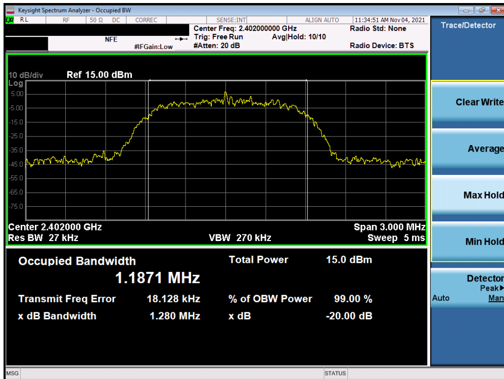
Plot 7-7. 20dB Bandwidth Plot (Bluetooth, 3Mbps – Ch. 0) Antenna 1
