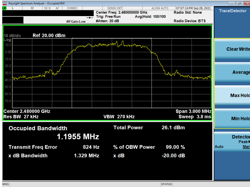
Plot 7-15. 20dB Bandwidth Plot (Bluetooth, 2Mbps – Ch. 78) Antenna 2
