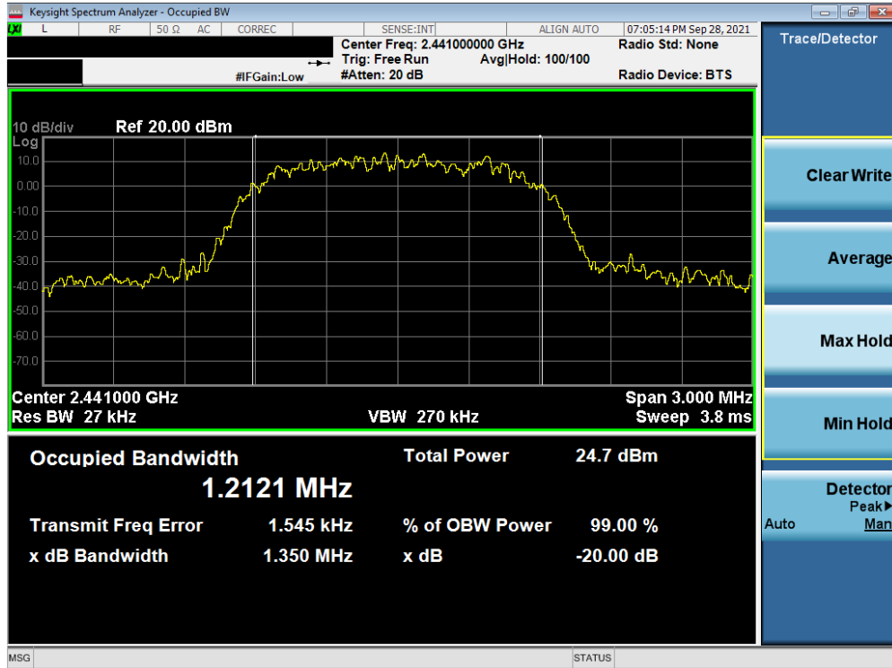
Plot 7-17. 20dB Bandwidth Plot (Bluetooth, 3Mbps – Ch. 39) Antenna 2
