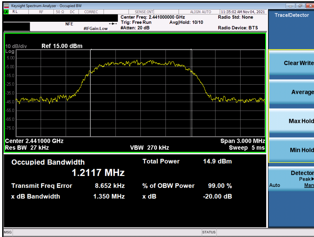
Plot 7-8. 20dB Bandwidth Plot (Bluetooth, 3Mbps – Ch. 39) Antenna 1
