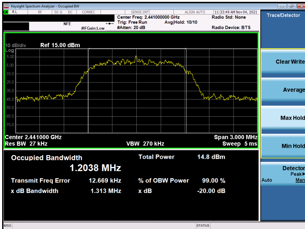
Plot 7-5. 20dB Bandwidth Plot (Bluetooth, 2Mbps – Ch. 39) Antenna 1
