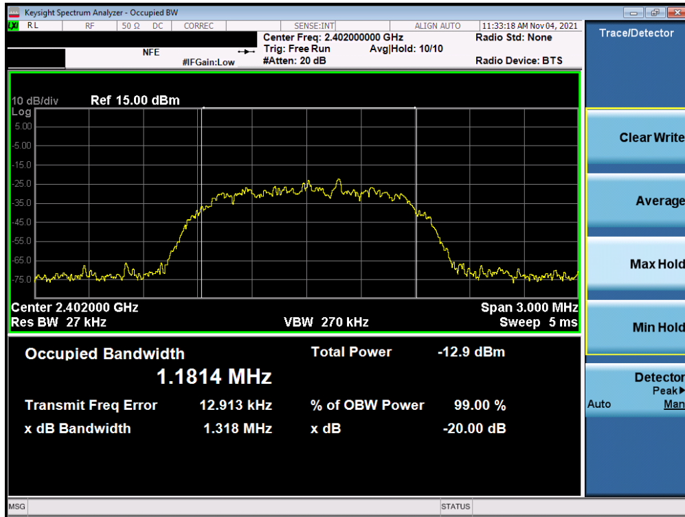
Plot 7-4. 20dB Bandwidth Plot (Bluetooth, 2Mbps – Ch. 0) Antenna 1
