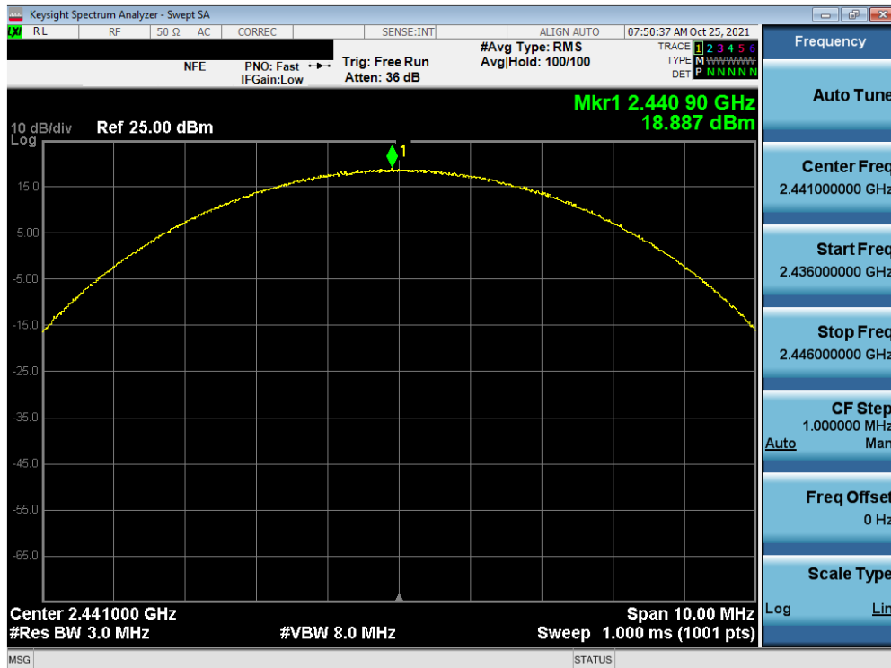
Plot 7-68. Peak Conducted Power 3Mbps – Ch. 39) Antenna 2 ePA
